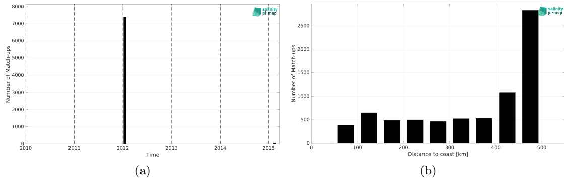
Figure 1: Number of match-ups between TSG (GOSUD-Sailing-ship) and SMOS SSS L3 v8 - 9 Days (CATDS-CEC-LOCEAN) SSS as a function of time (a) and as function of the distance to coast (b) over the Mississippi river plume Pi-MEP region and for the full satellite product period.
