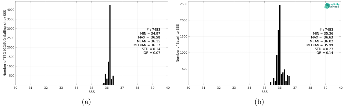
Figure 2: Histograms of SSS from TSG (GOSUD-Sailing-ship) (a) and SMOS SSS L3 v8 - 9 Days (CATDS-CEC-LOCEAN) (b) considering all match-up pairs per bins of 0.1 over the Mississippi river plume Pi-MEP region and for the full satellite product period.
