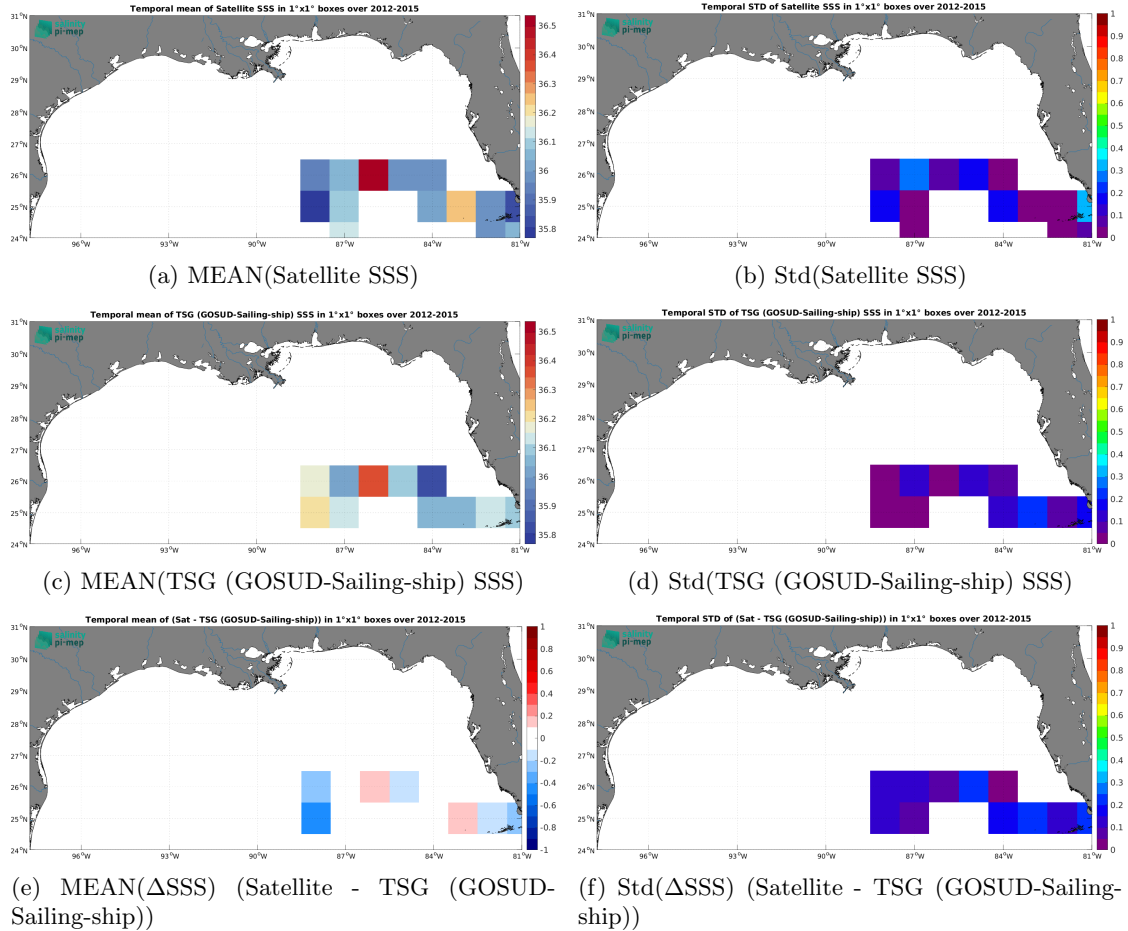
Figure 6: Temporal mean (left) and Std (right) of SSS from SMOS SSS L3 v8 - 9 Days (CATDS-CEC-LOCEAN) (top), TSG (GOSUD-Sailing-ship) (middle), and of \Delta\text{SSS} (Satellite - TSG (GOSUD-Sailing-ship)). Only match-up pairs are used to generate these maps.
