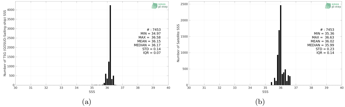
Figure 2: Histograms of SSS from TSG (GOSUD-Sailing-ship) (a) and SMOS SSS L3 v8 - 9 Days (CATDS-CECOS-LOCEAN) (b) considering all match-up pairs per bins of 0.1 over the Mississippi river plume Pi-MEP region and for the full satellite product period.
