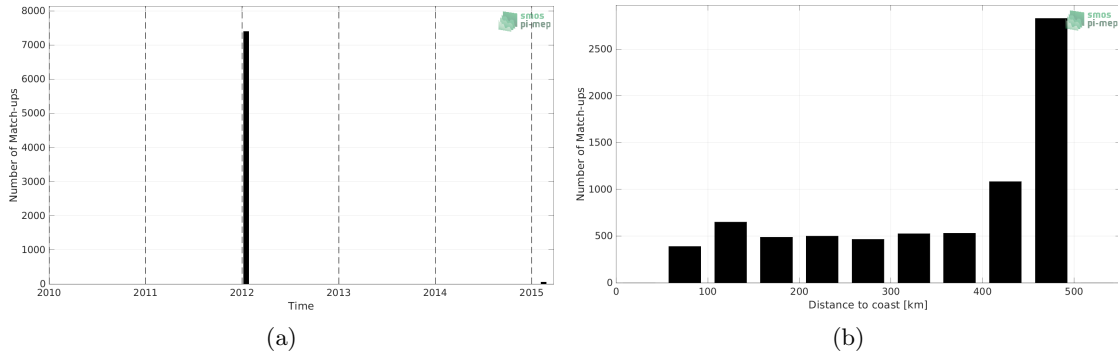
Figure 1: Number of match-ups between TSG (GOSUD-Sailing-ship) and SMOS SSS L3 v8 - 9 Days (CATDS-CECOS-LOCEAN) SSS as a function of time (a) and as function of the distance to coast (b) over the Mississippi river plume Pi-MEP region and for the full satellite product period.
