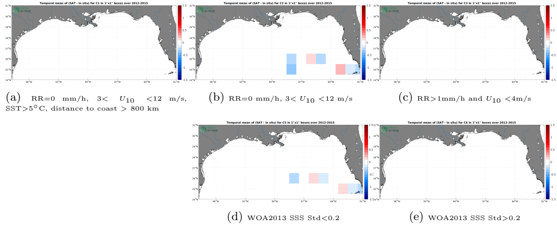
Figure 12: Temporal mean gridded over spatial boxes of size 1^{\circ}\times 1^{\circ} of \Delta SSS (SMOS SSS L3 v8 - 9 Days (CATDS-CECOS-LOCEAN) - TSG (GOSUD-Sailing-ship)) for 5 different subdatasets corresponding to:RR=0 mm/h, 3 < U_{10} < 12 m/s, SST >5^{\circ}\text{C} , distance to coast > 800 km (a), RR=0 mm/h, 3 < U_{10} < 12 m/s (b), RR >1 mm/h and U_{10} < 4 m/s (c), WOA2013 SSS Std <0.2 (d), WOA2013 SSS Std >0.2 (e).
