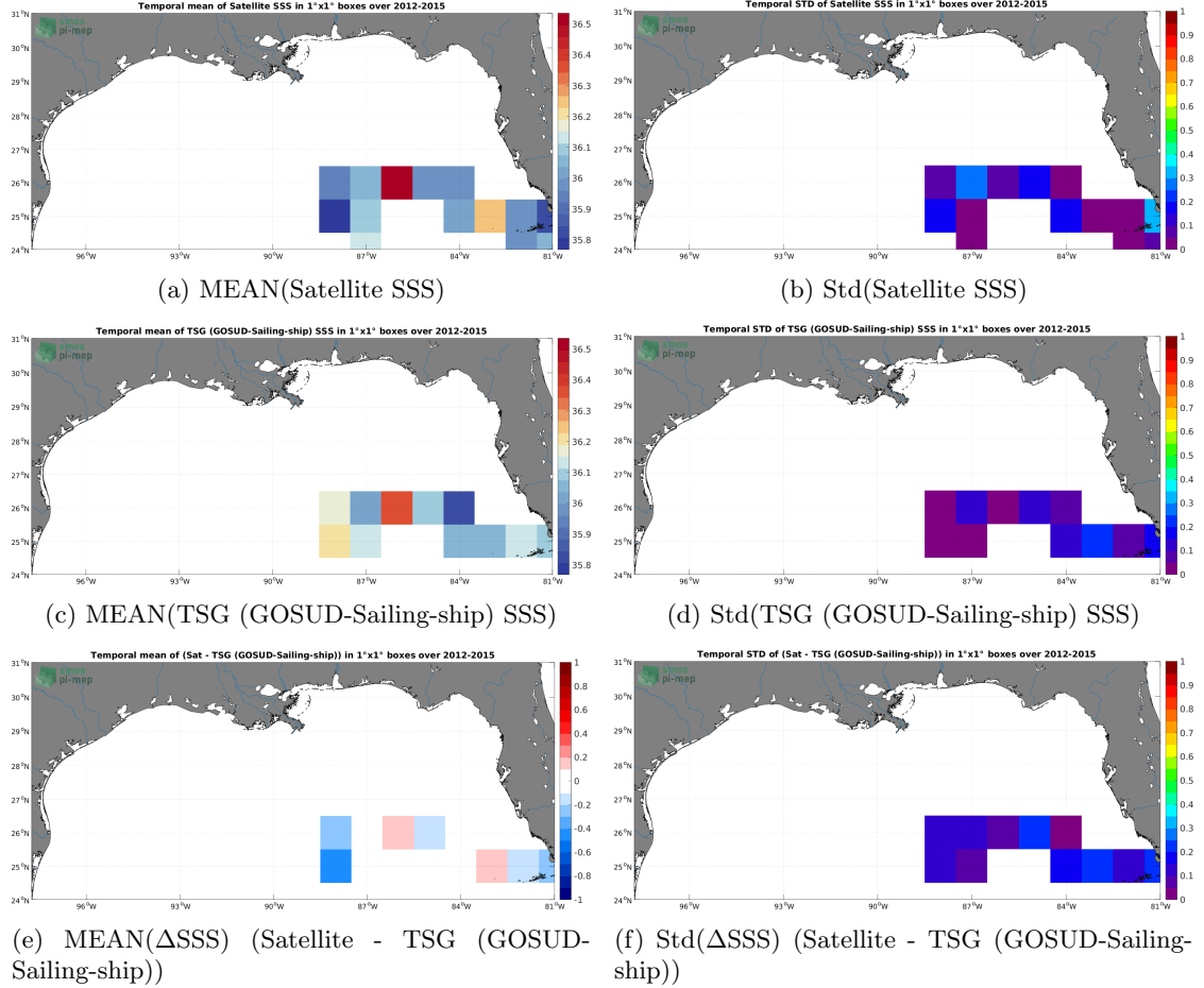
Figure 6: Temporal mean (left) and Std (right) of SSS from SMOS SSS L3 v8 - 9 Days (CATDS-CECOS-LOCEAN) (top), TSG (GOSUD-Sailing-ship) (middle), and of \Delta\text{SSS} (Satellite - TSG (GOSUD-Sailing-ship)). Only match-up pairs are used to generate these maps.
