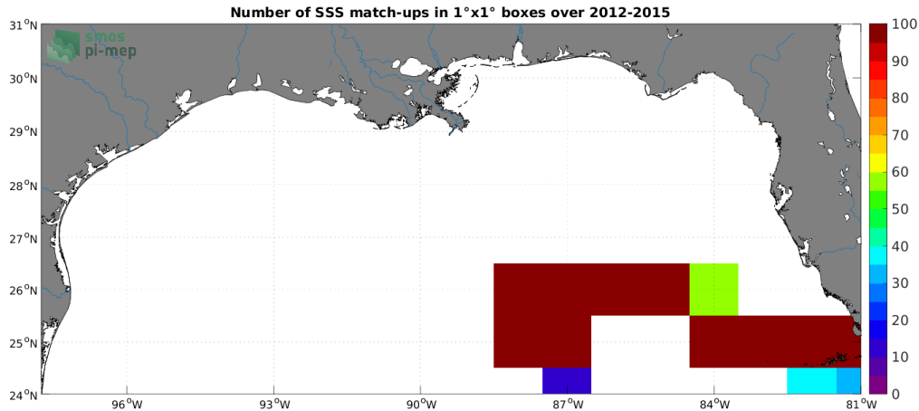
Figure 4: Number of SSS match-ups between TSG (GOSUD-Sailing-ship) SSS and the SMOS SSS L3 v8 - 9 Days (CATDS-CECOS-LOCEAN) SSS product for the Mississippi river plume Pi-MEP region over 1^\circ \times 1^\circ boxes and for the full satellite product period.
