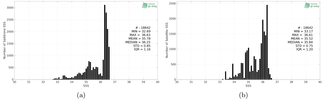
Figure 2: Histograms of SSS from Saildrone (a) and SMOS SSS L3 v8 - 9 Days (CATDS-CECOS-LOCEAN) (b) considering all match-up pairs per bins of 0.1 over the Mississippi river plume Pi-MEP region and for the full satellite product period.
