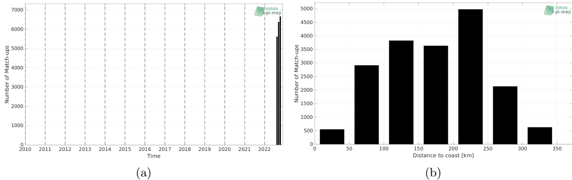
Figure 1: Number of match-ups between Saildrone and SMOS SSS L3 v8 - 9 Days (CATDS-CECOS-LOCEAN) SSS as a function of time (a) and as function of the distance to coast (b) over the Mississippi river plume Pi-MEP region and for the full satellite product period.
