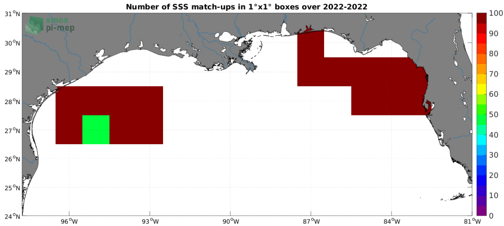
Figure 4: Number of SSS match-ups between Saildrone SSS and the SMOS SSS L3 v8 - 9 Days (CATDS-CECOS-LOCEAN) SSS product for the Mississippi river plume Pi-MEP region over 1^\circ \times 1^\circ boxes and for the full satellite product period.
