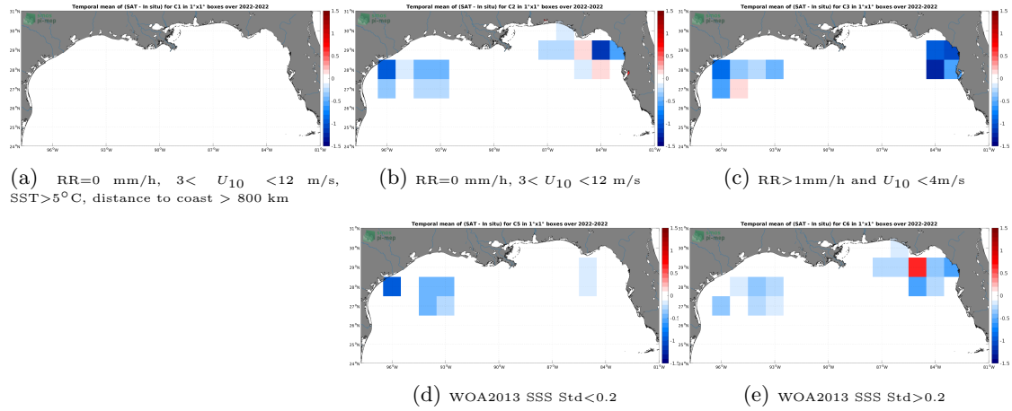
Figure 12: Temporal mean gridded over spatial boxes of size 1^{\circ}\times 1^{\circ} of \Delta\text{SSS} (SMOS SSS L3 v8 - 9 Days (CATDS-CECOS-LOCEAN) - Saildrone) for 5 different subdatasets corresponding to:RR=0 mm/h, 3 < U_{10} < 12 m/s, SST >5^{\circ}\text{C} , distance to coast > 800 km (a), RR=0 mm/h, 3 < U_{10} < 12 m/s (b), RR >1 mm/h and U_{10} < 4 m/s (c), WOA2013 SSS Std <0.2 (d), WOA2013 SSS Std >0.2 (e).
