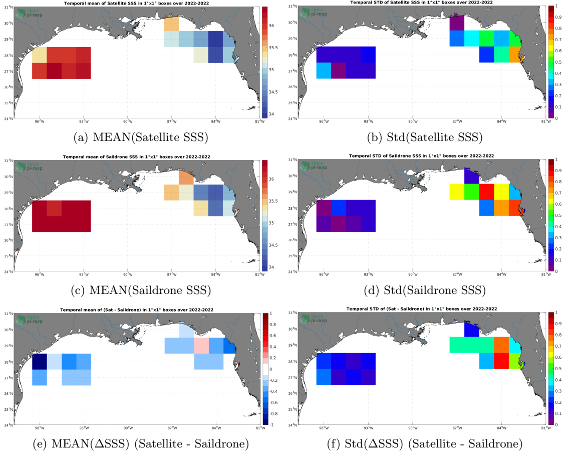
Figure 6: Temporal mean (left) and Std (right) of SSS from SMOS SSS L3 v8 - 9 Days (CATDS-CECOS-LOCEAN) (top), Saildrone (middle), and of \Delta\text{SSS} (Satellite - Saildrone). Only match-up pairs are used to generate these maps.
