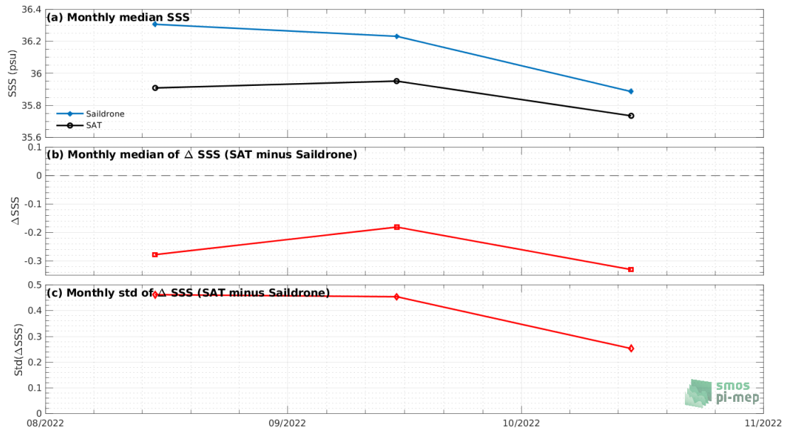
Figure 7: Time series of the monthly median SSS (top), median of \Delta SSS (Satellite - SSSaildrone) and Std of \Delta SSS (Satellite - SSSaildrone) over the Mississippi river plume Pi-MEP region considering all match-ups collected by the Pi-MEP.
