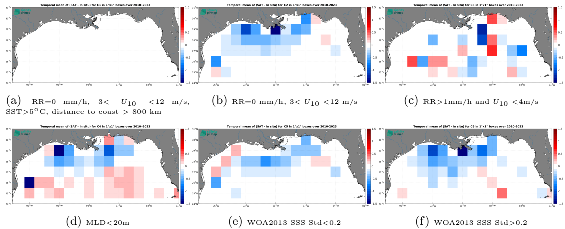
Figure 12: Temporal mean gridded over spatial boxes of size 1^{\circ}\times 1^{\circ} of \Delta\text{SSS} (SMOS SSS L3 v8 - 9 Days (CATDS-CEC-LOCEAN) - Argo) for 6 different subdatasets corresponding to:RR=0 mm/h, 3 < U_{10} < 12 m/s, SST > 5^{\circ}\text{C} , distance to coast > 800 km (a), RR=0 mm/h, 3 < U_{10} < 12 m/s (b), RR > 1\text{mm/h} and U_{10} < 4\text{m/s} (c),MLD < 20\text{m} (d),WOA2013 SSS Std < 0.2 (e),WOA2013 SSS Std > 0.2 (f).
