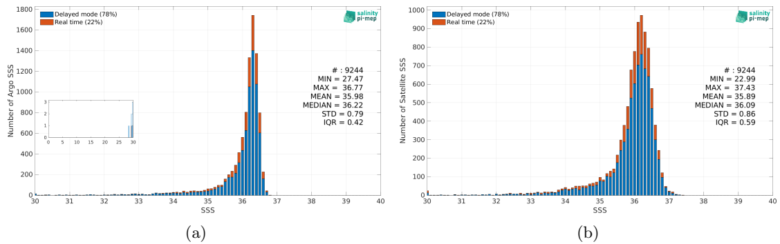
Figure 2: Histograms of SSS from Argo (a) and SMOS SSS L3 v8 - 9 Days (CATDS-CEC-LOCEAN) (b) considering all match-up pairs per bins of 0.1 over the Mississippi river plume Pi-MEP region and for the full satellite product period.
