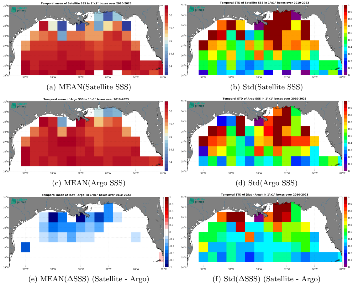
Figure 6: Temporal mean (left) and Std (right) of SSS from SMOS SSS L3 v8 - 9 Days (CATDS-CEC-LOCEAN) (top), Argo (middle), and of \Delta SSS (Satellite - Argo). Only match-up pairs are used to generate these maps.
