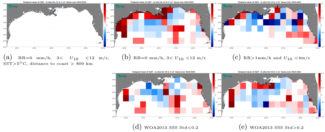
Figure 12: Temporal mean gridded over spatial boxes of size 1^{\circ}\times 1^{\circ} of \Delta\text{SSS} (SMOS SSS L3 v8 - 18 Days (CATDS-CEC-LOCEAN) - TSG (SAMOS)) for 5 different subdatasets corresponding to:RR=0 mm/h, 3 < U_{10} < 12 m/s, SST > 5^{\circ}\text{C} , distance to coast > 800 km (a), RR=0 mm/h, 3 < U_{10} < 12 m/s (b), RR > 1 mm/h and U_{10} < 4 m/s (c), WOA2013 SSS Std < 0.2 (d), WOA2013 SSS Std > 0.2 (e).
