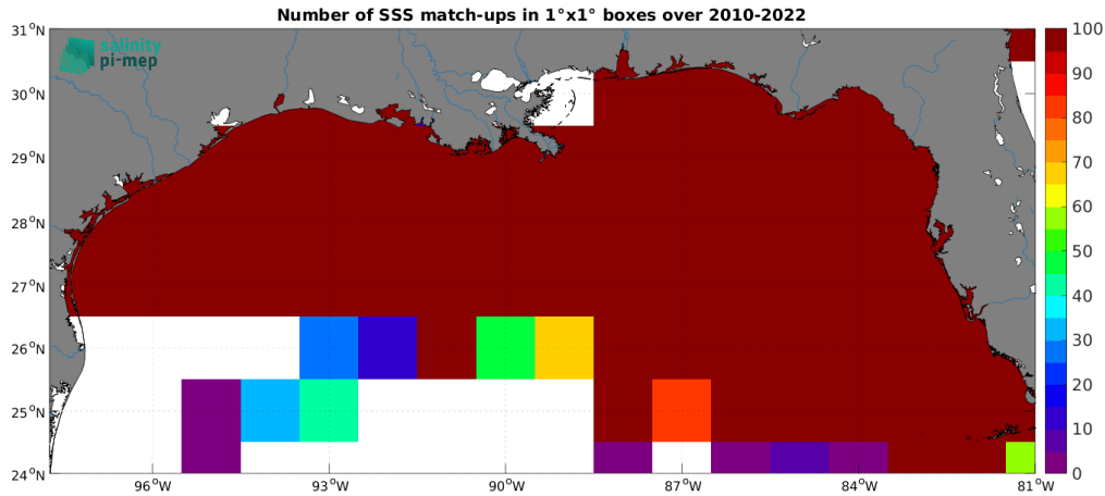
Figure 4: Number of SSS match-ups between TSG (SAMOS) SSS and the SMOS SSS L3 v8 - 18 Days (CATDS-CEC-LOCEAN) SSS product for the Mississippi river plume Pi-MEP region over 1^\circ \times 1^\circ boxes and for the full satellite product period.
