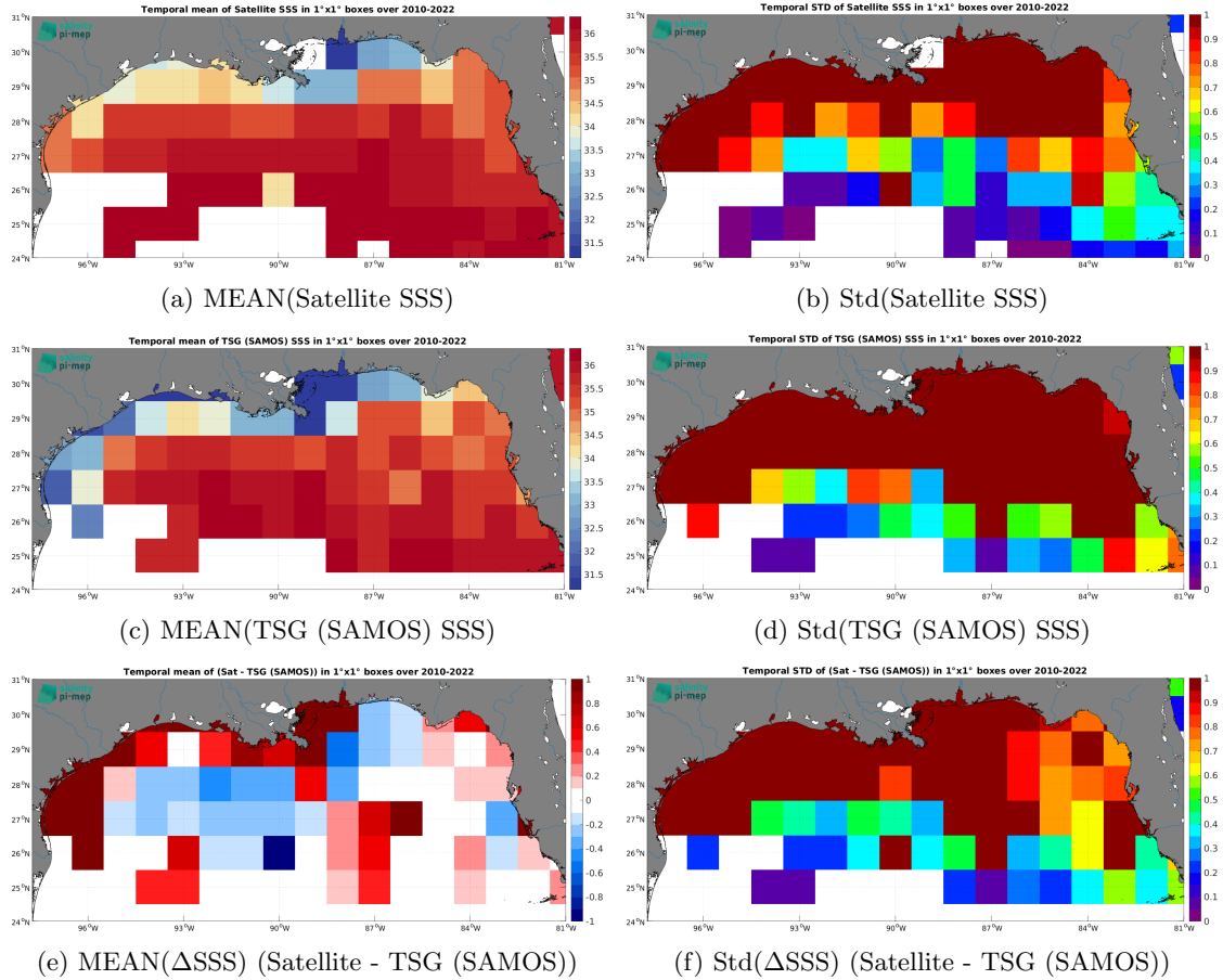
Figure 6: Temporal mean (left) and Std (right) of SSS from SMOS SSS L3 v8 - 18 Days (CATDS-CEC-LOCEAN) (top), TSG (SAMOS) (middle), and of \Delta\text{SSS} (Satellite - TSG (SAMOS)). Only match-up pairs are used to generate these maps.
