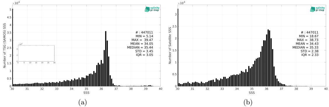
Figure 2: Histograms of SSS from TSG (SAMOS) (a) and SMOS SSS L3 v8 - 18 Days (CATDS-CEC-LOCEAN) (b) considering all match-up pairs per bins of 0.1 over the Mississippi river plume Pi-MEP region and for the full satellite product period.
