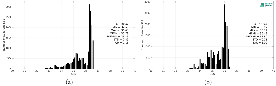
Figure 2: Histograms of SSS from Saildrone (a) and SMOS SSS L3 v8 - 18 Days (CATDS-CEC-LOCEAN) (b) considering all match-up pairs per bins of 0.1 over the Mississippi river plume Pi-MEP region and for the full satellite product period.
