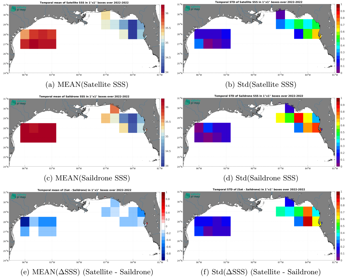
Figure 6: Temporal mean (left) and Std (right) of SSS from SMOS SSS L3 v8 - 18 Days (CATDS-CEC-LOCEAN) (top), Saildrone (middle), and of \Delta SSS (Satellite - Saildrone). Only match-up pairs are used to generate these maps.
