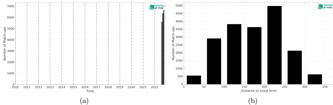
Figure 1: Number of match-ups between Saildrone and SMOS SSS L3 v8 - 18 Days (CATDS-CEC-LOCEAN) SSS as a function of time (a) and as function of the distance to coast (b) over the Mississippi river plume Pi-MEP region and for the full satellite product period.
