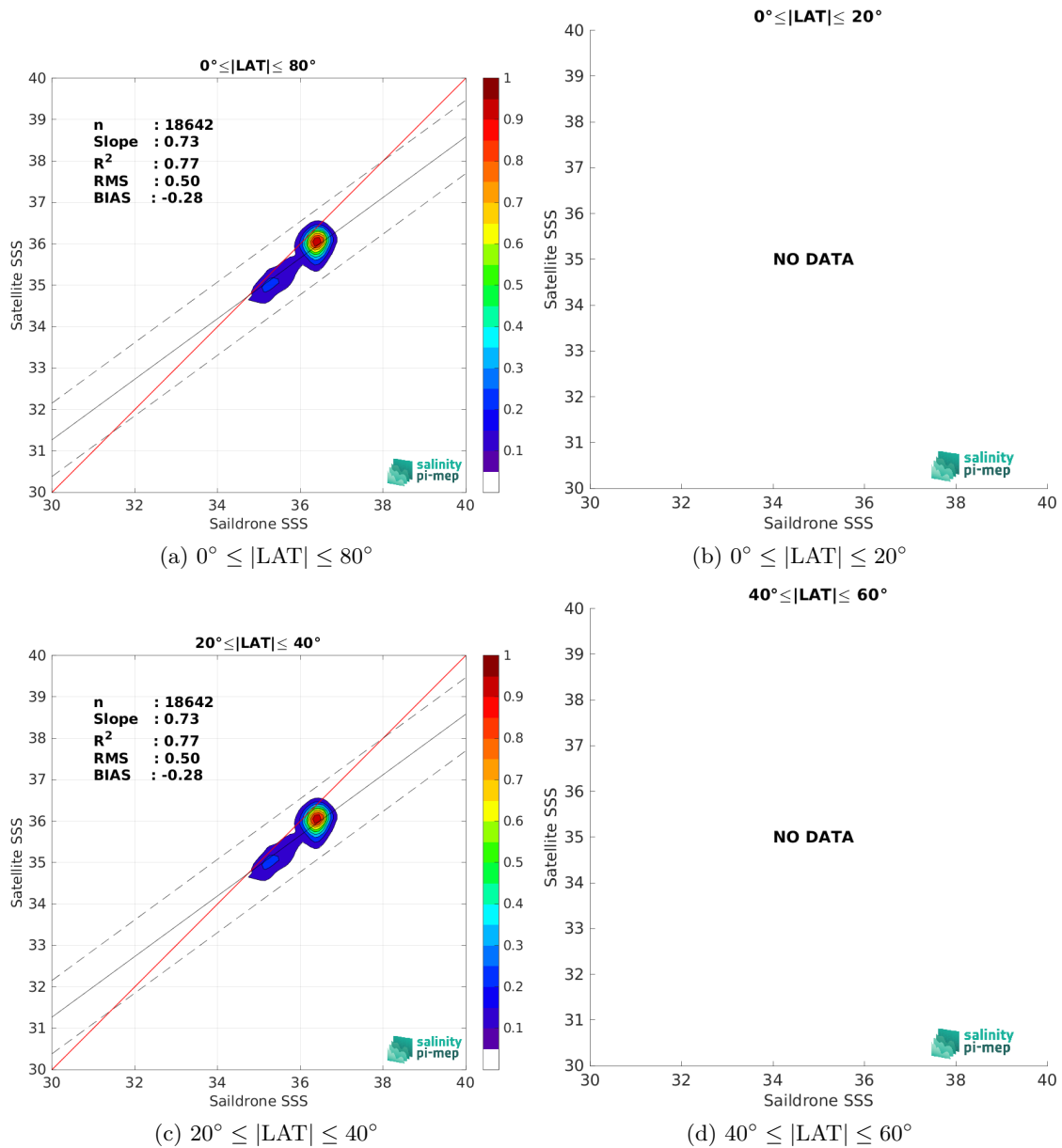
Figure 9: Contour maps of the concentration of SMOS SSS L3 v8 - 18 Days (CATDS-CEC-LOCEAN) SSS (y-axis) versus Saïldrone SSS (x-axis) at match-up pairs for different latitude bands. For each plot, the red line shows x=y . The black thin and dashed lines indicate a linear fit through the data cloud and the \pm 95\% confidence levels, respectively. The number match-up pairs n , the slope and R^2 coefficient of the linear fit, the root mean square (RMS) and the mean bias between satellite and in situ data are indicated for each latitude band in each plots.
