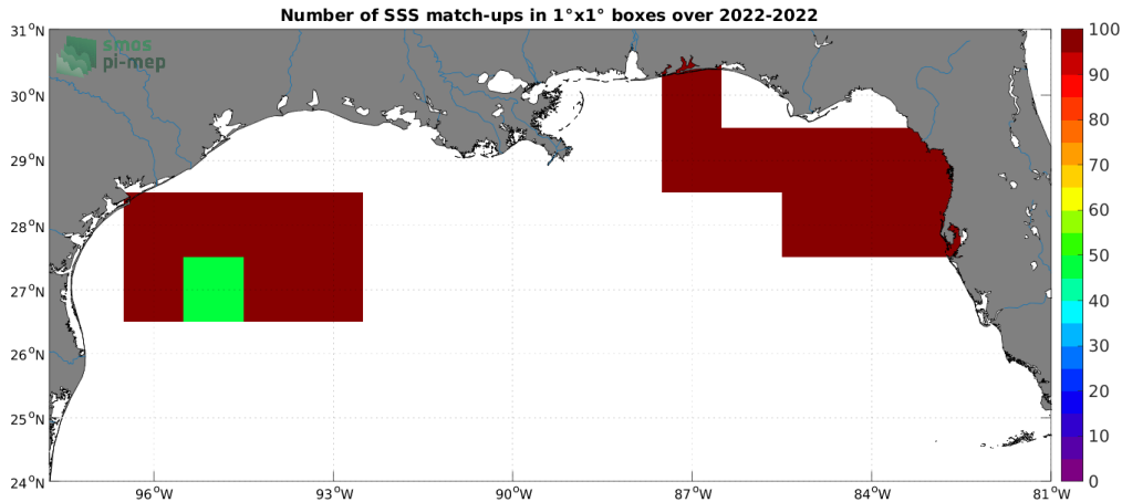
Figure 4: Number of SSS match-ups between Saildrone SSS and the SMOS SSS L3 v8 - 18 Days (CATDS-CECOS-LOCEAN) SSS product for the Mississippi river plume Pi-MEP region over 1^\circ \times 1^\circ boxes and for the full satellite product period.
