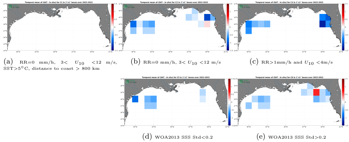
Figure 12: Temporal mean gridded over spatial boxes of size 1^{\circ}\times 1^{\circ} of \Delta\text{SSS} (SMOS SSS L3 v8 - 18 Days (CATDS-CECOS-LOCEAN) - Saildrone) for 5 different subdatasets corresponding to:RR=0 mm/h, 3 < U_{10} < 12 m/s, SST >5^{\circ}\text{C} , distance to coast > 800 km (a), RR=0 mm/h, 3 < U_{10} < 12 m/s (b), RR >1 mm/h and U_{10} < 4 m/s (c), WOA2013 SSS Std <0.2 (d), WOA2013 SSS Std >0.2 (e).
