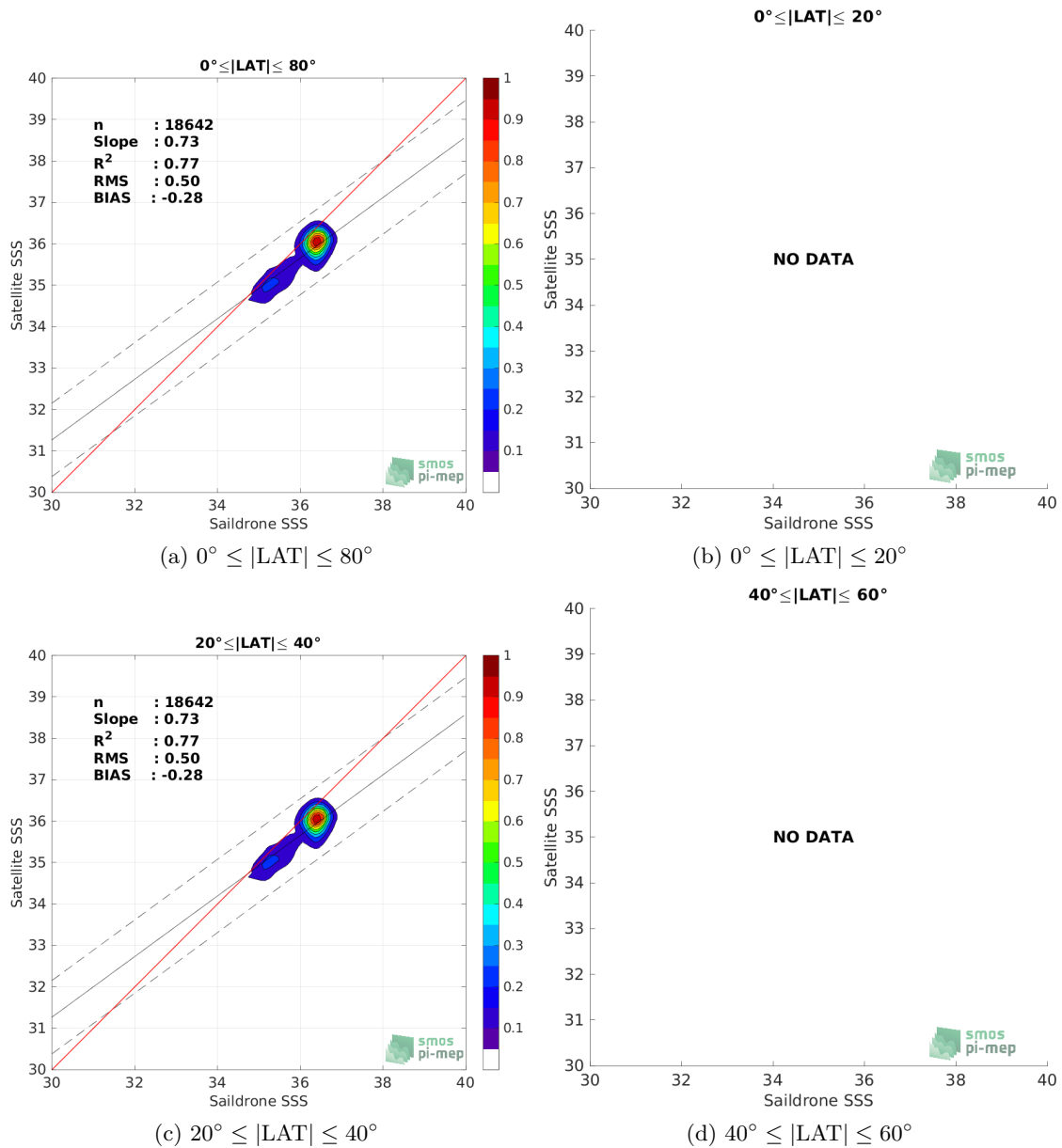
Figure 9: Contour maps of the concentration of SMOS SSS L3 v8 - 18 Days (CATDS-CECOS-LOCEAN) SSS (y-axis) versus Saïldrone SSS (x-axis) at match-up pairs for different latitude bands. For each plot, the red line shows x=y . The black thin and dashed lines indicate a linear fit through the data cloud and the \pm 95\% confidence levels, respectively. The number match-up pairs n , the slope and R^2 coefficient of the linear fit, the root mean square (RMS) and the mean bias between satellite and in situ data are indicated for each latitude band in each plots.
