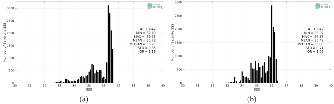
Figure 2: Histograms of SSS from Saildrone (a) and SMOS SSS L3 v8 - 18 Days (CATDS-CECOS-LOCEAN) (b) considering all match-up pairs per bins of 0.1 over the Mississippi river plume Pi-MEP region and for the full satellite product period.
