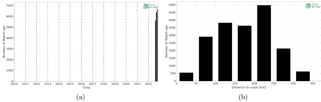
Figure 1: Number of match-ups between Saildrone and SMOS SSS L3 v8 - 18 Days (CATDS-CECOS-LOCEAN) SSS as a function of time (a) and as function of the distance to coast (b) over the Mississippi river plume Pi-MEP region and for the full satellite product period.
