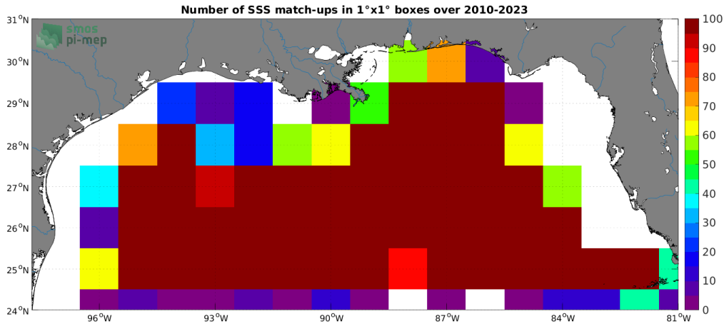
Figure 4: Number of SSS match-ups between Argo SSS and the SMOS SSS L3 v8 - 18 Days (CATDS-CECOS-LOCEAN) SSS product for the Mississippi river plume Pi-MEP region over 1^\circ \times 1^\circ boxes and for the full satellite product period.
