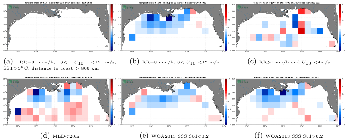
Figure 12: Temporal mean gridded over spatial boxes of size 1^{\circ}\times 1^{\circ} of \Delta\text{SSS} (SMOS SSS L3 v8 - 18 Days (CATDS-CECOS-LOCEAN) - Argo) for 6 different subdatasets corresponding to:RR=0 mm/h, 3 < U_{10} < 12 m/s, SST >5^{\circ}\text{C} , distance to coast > 800 km (a), RR=0 mm/h, 3 < U_{10} < 12 m/s (b), RR >1\text{mm/h} and U_{10} < 4\text{m/s} (c),MLD <20\text{m} (d),WOA2013 SSS Std <0.2 (e),WOA2013 SSS Std >0.2 (f).
