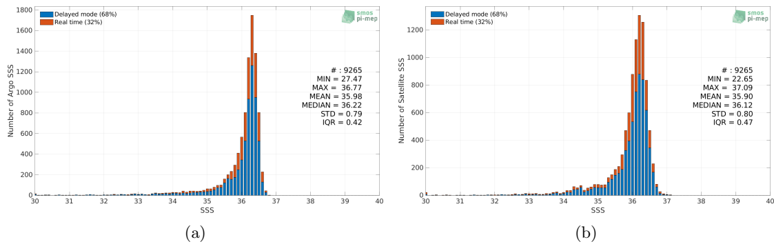
Figure 2: Histograms of SSS from Argo (a) and SMOS SSS L3 v8 - 18 Days (CATDS-CECOS-LOCEAN) (b) considering all match-up pairs per bins of 0.1 over the Mississippi river plume Pi-MEP region and for the full satellite product period.
