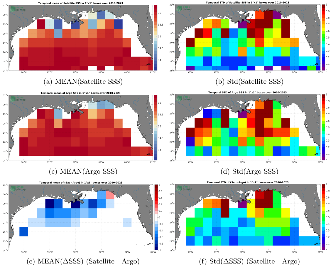
Figure 6: Temporal mean (left) and Std (right) of SSS from SMOS SSS L3 v8 - 18 Days (CATDS-CECOS-LOCEAN) (top), Argo (middle), and of \Delta SSS (Satellite - Argo). Only match-up pairs are used to generate these maps.
