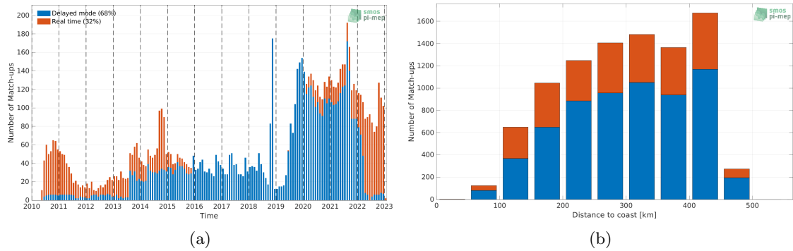
Figure 1: Number of match-ups between Argo and SMOS SSS L3 v8 - 18 Days (CATDS-CECOS-LOCEAN) SSS as a function of time (a) and as function of the distance to coast (b) over the Mississippi river plume Pi-MEP region and for the full satellite product period.
