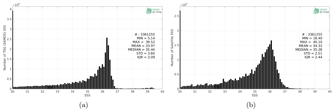
Figure 2: Histograms of SSS from TSG (SAMOS) (a) and SMOS SSS L3 v5 - 9 Days (CATDS-CECOS-LOCEAN) (b) considering all match-up pairs per bins of 0.1 over the Mississippi river plume Pi-MEP region and for the full satellite product period.
