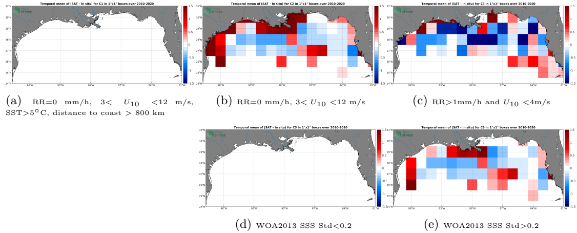
Figure 12: Temporal mean gridded over spatial boxes of size 1^{\circ}\times 1^{\circ} of \Delta\text{SSS} (SMOS SSS L3 v5 - 9 Days (CATDS-CECOS-LOCEAN) - TSG (SAMOS)) for 5 different subdatasets corresponding to:RR=0 mm/h, 3 < U_{10} < 12 m/s, SST >5^{\circ}\text{C} , distance to coast > 800 km (a), RR=0 mm/h, 3 < U_{10} < 12 m/s (b), RR >1 mm/h and U_{10} < 4 m/s (c), WOA2013 SSS Std <0.2 (d), WOA2013 SSS Std >0.2 (e).
