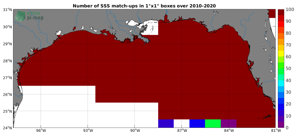
Figure 4: Number of SSS match-ups between TSG (SAMOS) SSS and the SMOS SSS L3 v5 - 9 Days (CATDS-CECOS-LOCEAN) SSS product for the Mississippi river plume Pi-MEP region over 1^\circ \times 1^\circ boxes and for the full satellite product period.
