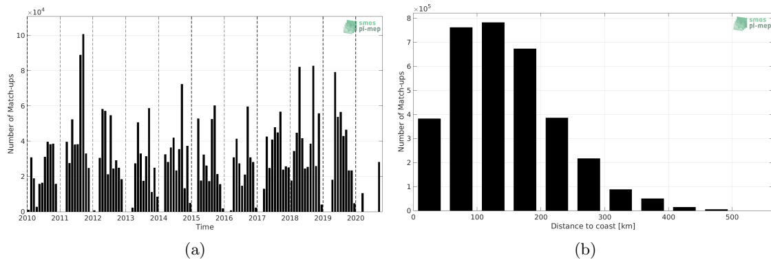
Figure 1: Number of match-ups between TSG (SAMOS) and SMOS SSS L3 v5 - 9 Days (CATDS-CECOS-LOCEAN) SSS as a function of time (a) and as function of the distance to coast (b) over the Mississippi river plume Pi-MEP region and for the full satellite product period.
