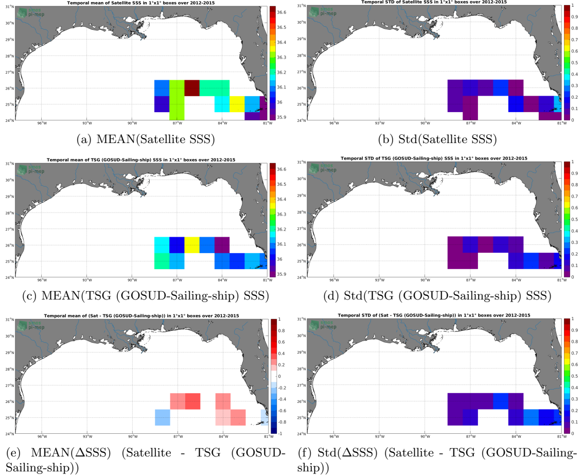
Figure 6: Temporal mean (left) and Std (right) of SSS from SMOS SSS L3 v5 - 9 Days (CATDS-CECOS-LOCEAN) (top), TSG (GOSUD-Sailing-ship) (middle), and of \Delta\text{SSS} (Satellite - TSG (GOSUD-Sailing-ship)). Only match-up pairs are used to generate these maps.
