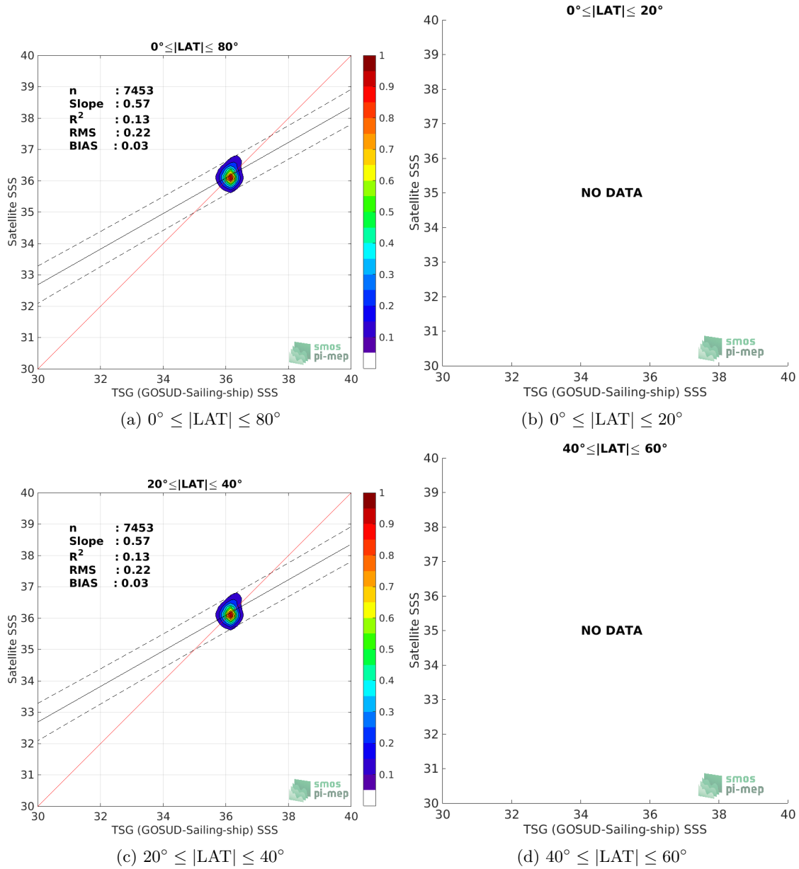
Figure 9: Contour maps of the concentration of SMOS SSS L3 v5 - 9 Days (CATDS-CECOS-LOCEAN) SSS (y-axis) versus TSG (GOSUD-Sailing-ship) SSS (x-axis) at match-up pairs for different latitude bands. For each plot, the red line shows x=y . The black thin and dashed lines indicate a linear fit through the data cloud and the \pm 95\% confidence levels, respectively. The number match-up pairs n , the slope and R^2 coefficient of the linear fit, the root mean square (RMS) and the mean bias between satellite and in situ data are indicated for each latitude band in each plots.
