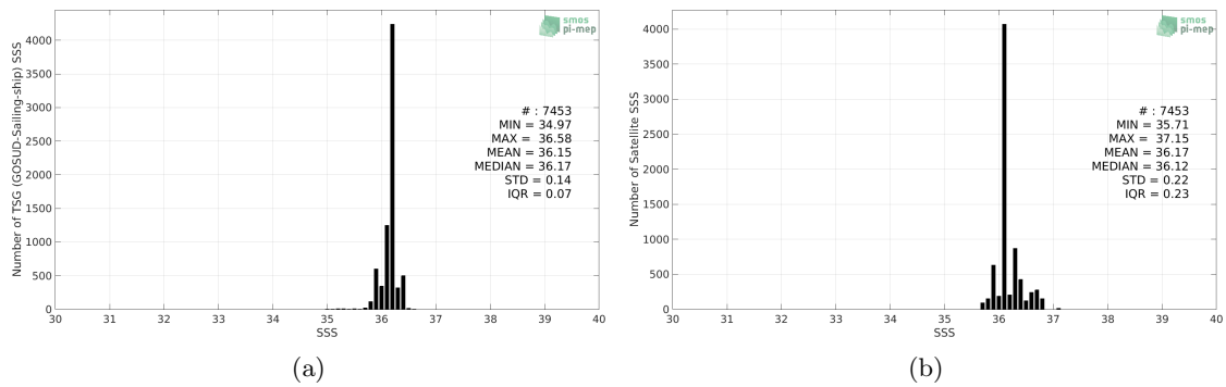
Figure 2: Histograms of SSS from TSG (GOSUD-Sailing-ship) (a) and SMOS SSS L3 v5 - 9 Days (CATDS-CECOS-LOCEAN) (b) considering all match-up pairs per bins of 0.1 over the Mississippi river plume Pi-MEP region and for the full satellite product period.
