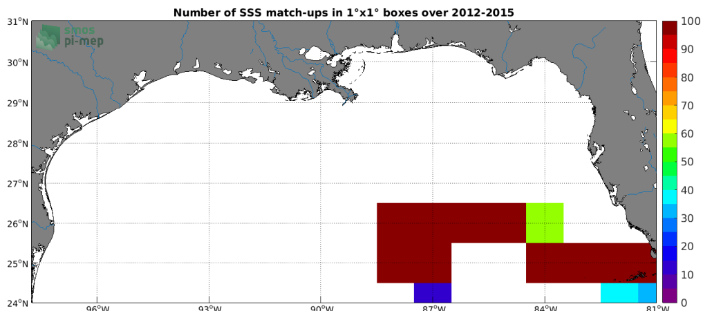
Figure 4: Number of SSS match-ups between TSG (GOSUD-Sailing-ship) SSS and the SMOS SSS L3 v5 - 9 Days (CATDS-CECOS-LOCEAN) SSS product for the Mississippi river plume Pi-MEP region over 1^\circ \times 1^\circ boxes and for the full satellite product period.
