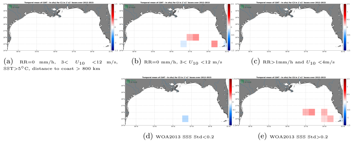
Figure 12: Temporal mean gridded over spatial boxes of size 1^\circ \times 1^\circ of \Delta SSS (SMOS SSS L3 v5 - 9 Days (CATDS-CECOS-LOCEAN) - TSG (GOSUD-Sailing-ship)) for 5 different subdatasets corresponding to: RR=0 mm/h, 3 < U_{10} < 12 m/s, SST > 5^\circ\text{C} , distance to coast > 800 km (a), RR=0 mm/h, 3 < U_{10} < 12 m/s (b), RR > 1 mm/h and U_{10} < 4 m/s (c), WOA2013 SSS Std < 0.2 (d), WOA2013 SSS Std > 0.2 (e).
