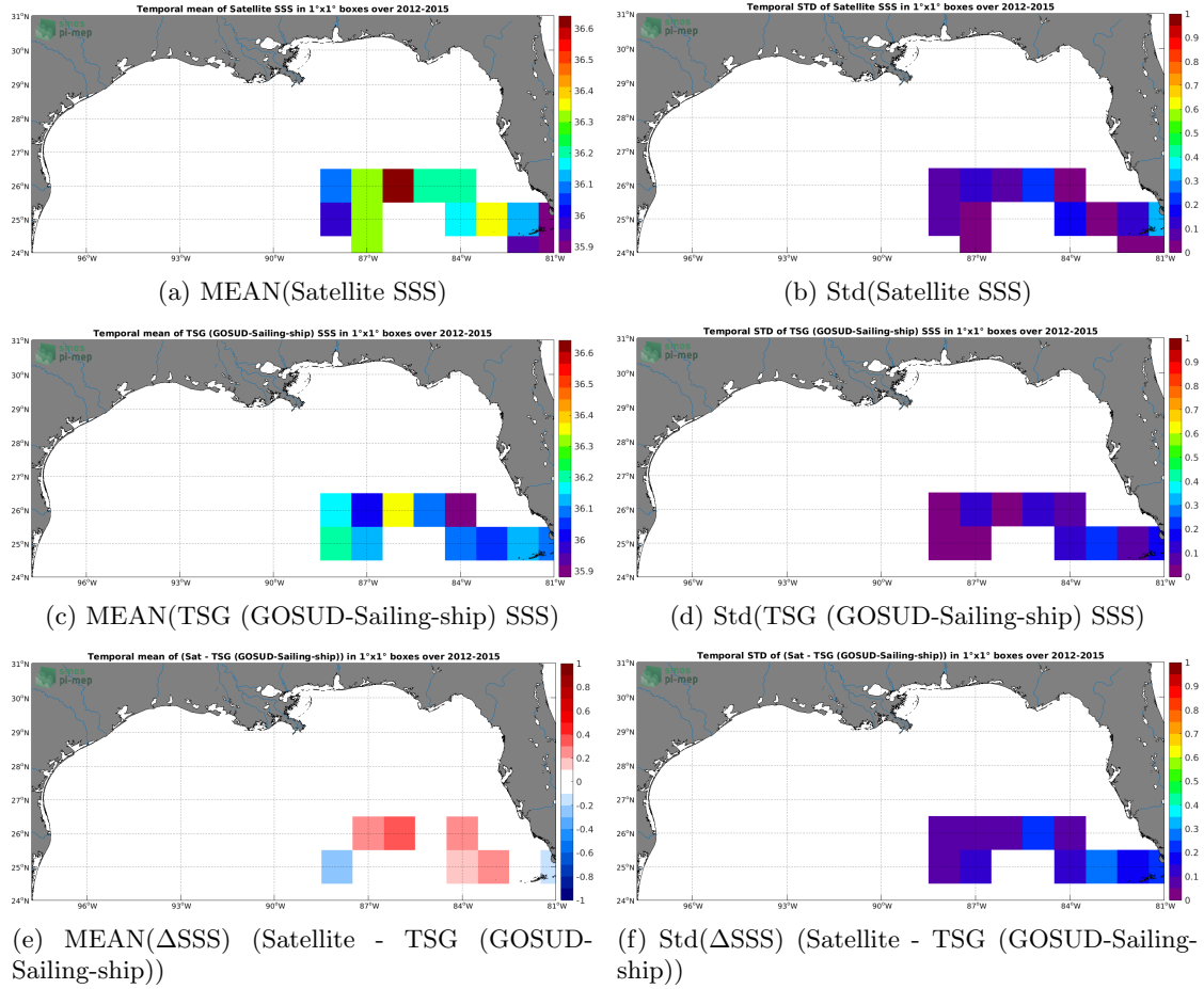
Figure 6: Temporal mean (left) and Std (right) of SSS from SMOS SSS L3 v5 - 9 Days (CATDS-CECOS-LOCEAN) (top), TSG (GOSUD-Sailing-ship) (middle), and of \Delta SSS (Satellite - TSG (GOSUD-Sailing-ship)). Only match-up pairs are used to generate these maps.
