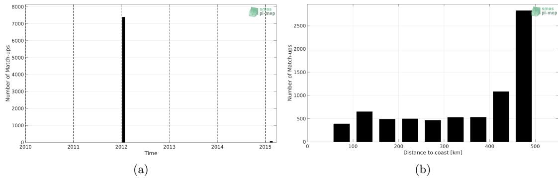
Figure 1: Number of match-ups between TSG (GOSUD-Sailing-ship) and SMOS SSS L3 v5 - 9 Days (CATDS-CECOS-LOCEAN) SSS as a function of time (a) and as function of the distance to coast (b) over the Mississippi river plume Pi-MEP region and for the full satellite product period.
