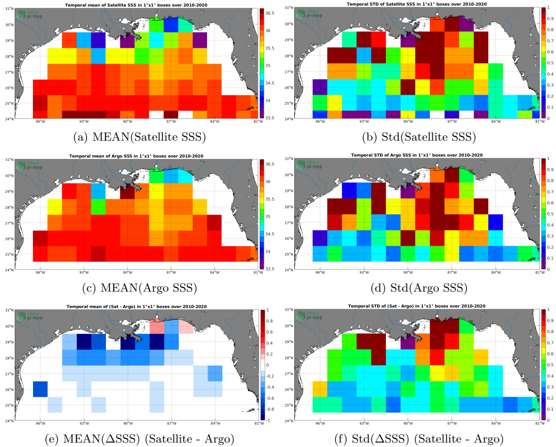
Figure 6: Temporal mean (left) and Std (right) of SSS from SMOS SSS L3 v5 - 9 Days (CATDS-CECOS-LOCEAN) (top), Argo (middle), and of \Delta\text{SSS} (Satellite - Argo). Only match-up pairs are used to generate these maps.
