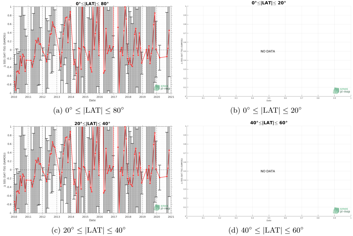
Figure 10: Monthly median (red curves) of \Delta SSS (Satellite - in situ TSG (SAMOS)) and \pm 1 Std (black vertical thick bars) as function of time for all the collected Pi-MEP match-up pairs estimated over the Mississippi river plume Pi-MEP region and for the full satellite product period are shown for different latitude bands: (a) 80^\circ\text{S}-80^\circ\text{N} , (b) 20^\circ\text{S}-20^\circ\text{N} , (c) 40^\circ\text{S}-20^\circ\text{S} and 20^\circ\text{N}-40^\circ\text{N} and (d) 60^\circ\text{S}-40^\circ\text{S} and 40^\circ\text{N}-60^\circ\text{N} .
