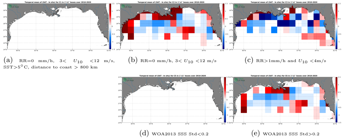
Figure 12: Temporal mean gridded over spatial boxes of size 1^{\circ}\times 1^{\circ} of \Delta\text{SSS} (SMOS SSS L3 v5 - 18 Days (CATDS-CECOS-LOCEAN) - TSG (SAMOS)) for 5 different subdatasets corresponding to:RR=0 mm/h, 3 < U_{10} < 12 m/s, SST >5^{\circ}\text{C} , distance to coast > 800 km (a), RR=0 mm/h, 3 < U_{10} < 12 m/s (b), RR >1 mm/h and U_{10} < 4 m/s (c), WOA2013 SSS Std <0.2 (d), WOA2013 SSS Std >0.2 (e).
