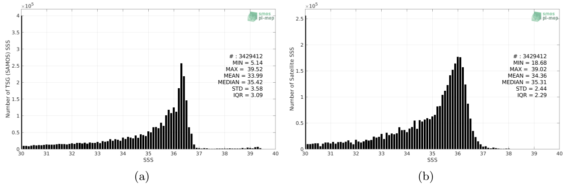
Figure 2: Histograms of SSS from TSG (SAMOS) (a) and SMOS SSS L3 v5 - 18 Days (CATDS-CECOS-LOCEAN) (b) considering all match-up pairs per bins of 0.1 over the Mississippi river plume Pi-MEP region and for the full satellite product period.
