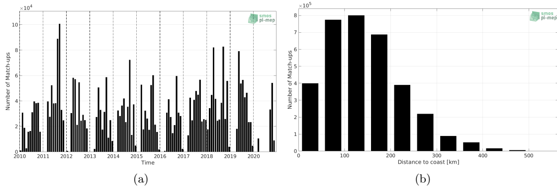
Figure 1: Number of match-ups between TSG (SAMOS) and SMOS SSS L3 v5 - 18 Days (CATDS-CECOS-LOCEAN) SSS as a function of time (a) and as function of the distance to coast (b) over the Mississippi river plume Pi-MEP region and for the full satellite product period.
