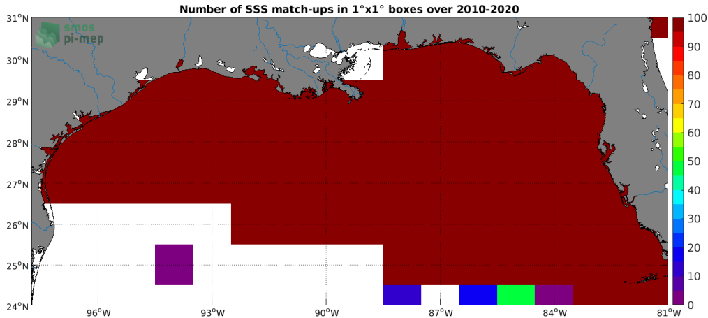
Figure 4: Number of SSS match-ups between TSG (SAMOS) SSS and the SMOS SSS L3 v5 - 18 Days (CATDS-CECOS-LOCEAN) SSS product for the Mississippi river plume Pi-MEP region over 1^\circ \times 1^\circ boxes and for the full satellite product period.
