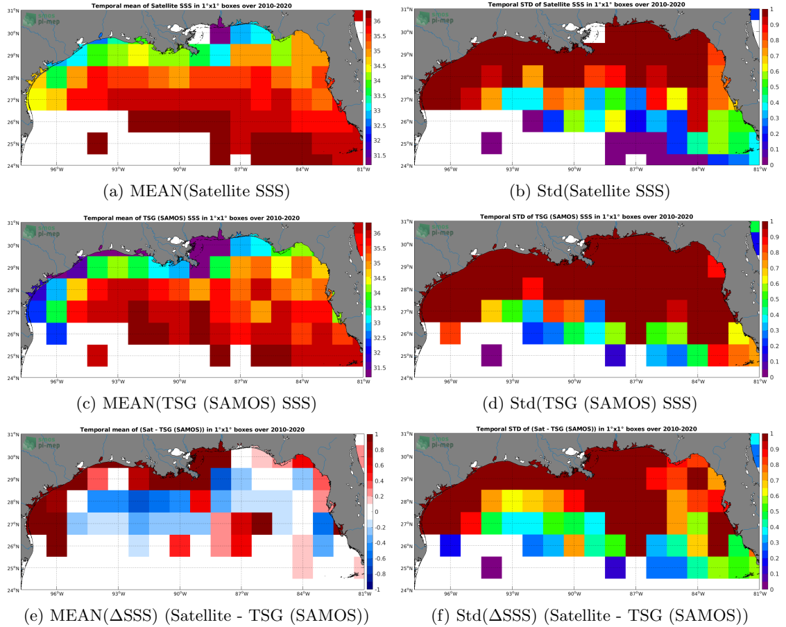
Figure 6: Temporal mean (left) and Std (right) of SSS from SMOS SSS L3 v5 - 18 Days (CATDS-CECOS-LOCEAN) (top), TSG (SAMOS) (middle), and of \Delta\text{SSS} (Satellite - TSG (SAMOS)). Only match-up pairs are used to generate these maps.
