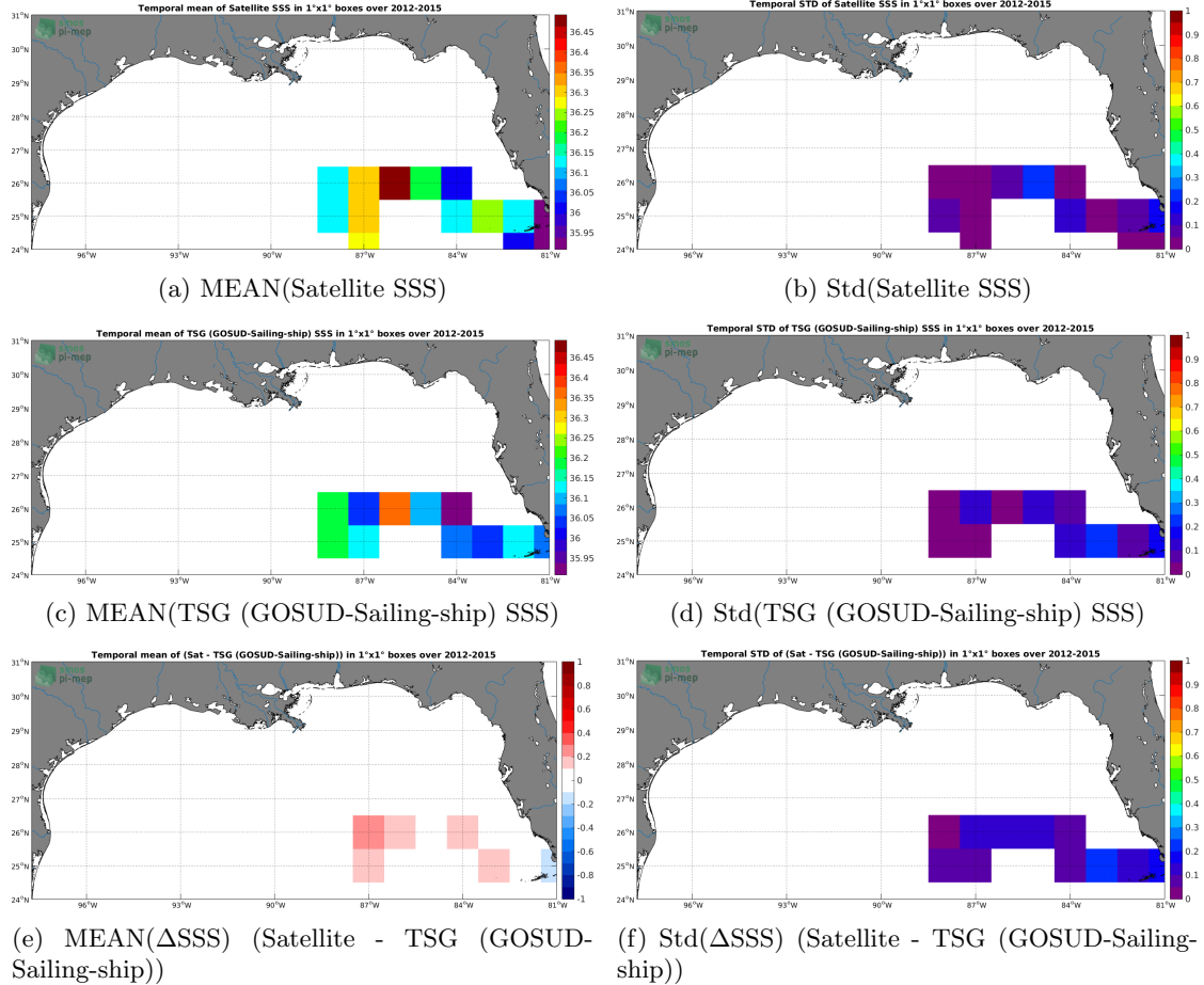
Figure 6: Temporal mean (left) and Std (right) of SSS from SMOS SSS L3 v5 - 18 Days (CATDS-CECOS-LOCEAN) (top), TSG (GOSUD-Sailing-ship) (middle), and of \Delta\text{SSS} (Satellite - TSG (GOSUD-Sailing-ship)). Only match-up pairs are used to generate these maps.
