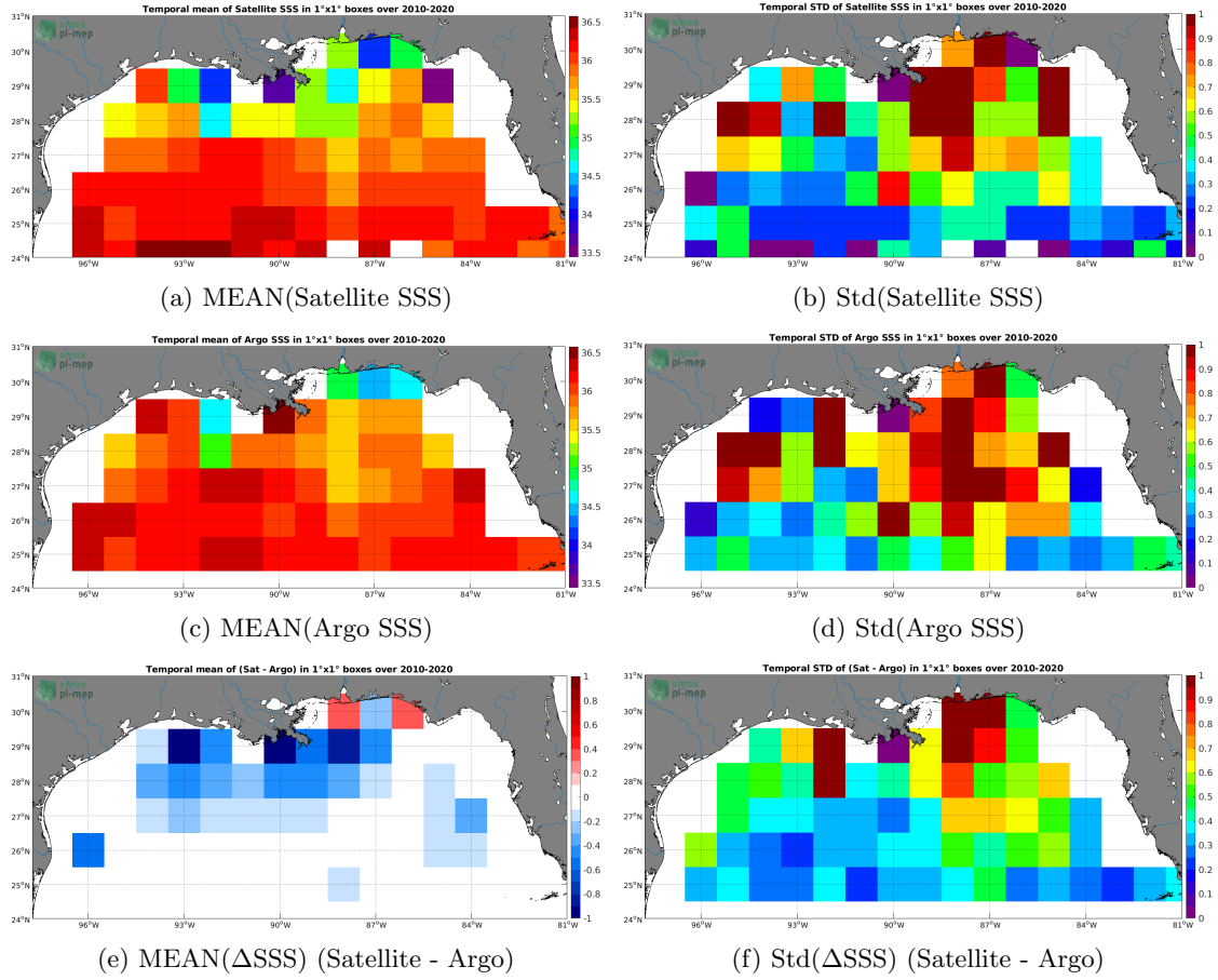
Figure 6: Temporal mean (left) and Std (right) of SSS from SMOS SSS L3 v5 - 18 Days (CATDS-CECOS-LOCEAN) (top), Argo (middle), and of \Delta SSS (Satellite - Argo). Only match-up pairs are used to generate these maps.
