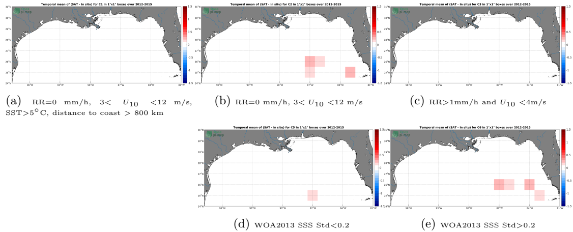
Figure 12: Temporal mean gridded over spatial boxes of size 1^{\circ}\times 1^{\circ} of \Delta SSS (SMOS-L3-CATDS-CECOS-LOCEAN-V4-18DAYS-25KM - TSG-GOSUD-Sailing-ship) for 5 different subdatasets corresponding to:RR=0 mm/h, 3 < U_{10} < 12 m/s, SST >5^{\circ}\text{C} , distance to coast > 800 km (a), RR=0 mm/h, 3 < U_{10} < 12 m/s (b), RR >1 mm/h and U_{10} < 4 m/s (c), WOA2013 SSS Std <0.2 (d), WOA2013 SSS Std >0.2 (e).
