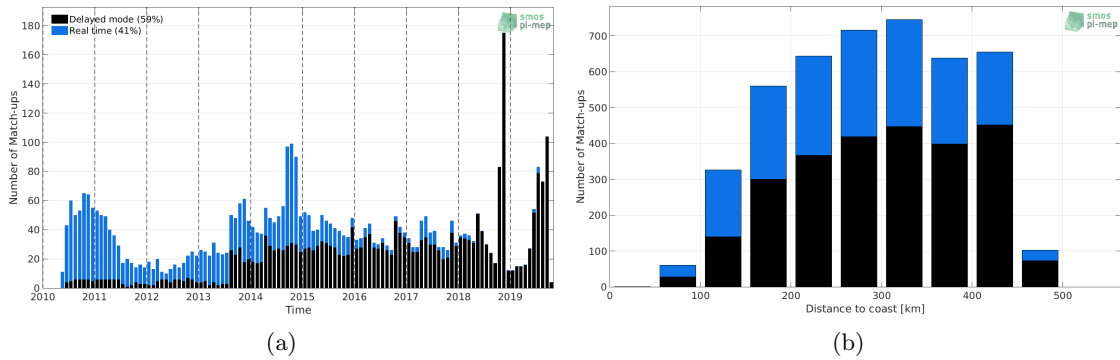
Figure 1: Number of match-ups between Argo and SMOS SSS L3 v4 - 18 Days (CATDS-CECOS-LOCEAN) SSS as a function of time (a) and as function of the distance to coast (b) over the Mississippi river plume Pi-MEP region and for the full satellite product period.
