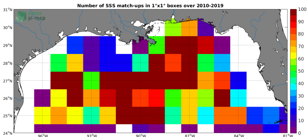
Figure 4: Number of SSS match-ups between Argo SSS and the SMOS SSS L3 v4 - 18 Days (CATDS-CECOS-LOCEAN) SSS product for the Mississippi river plume Pi-MEP region over 1^\circ \times 1^\circ boxes and for the full satellite product period.
