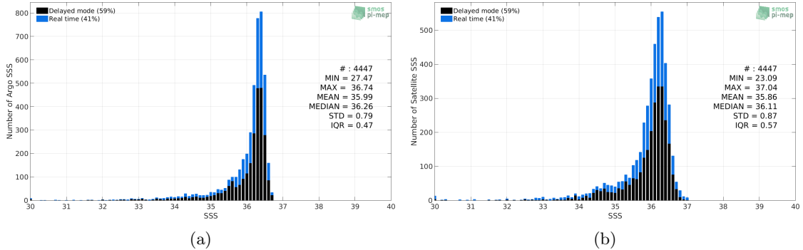
Figure 2: Histograms of SSS from Argo (a) and SMOS SSS L3 v4 - 18 Days (CATDS-CECOS-LOCEAN) (b) considering all match-up pairs per bins of 0.1 over the Mississippi river plume Pi-MEP region and for the full satellite product period.
