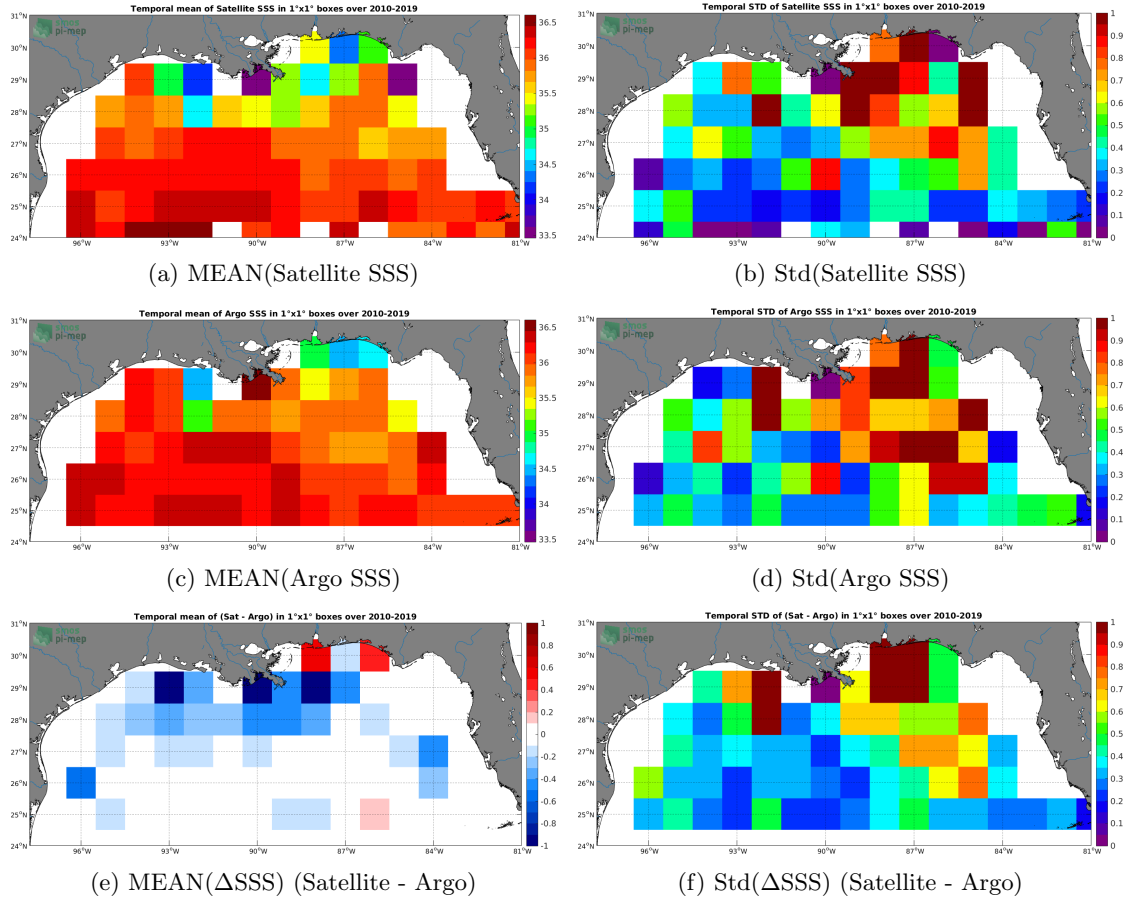
Figure 6: Temporal mean (left) and Std (right) of SSS from SMOS SSS L3 v4 - 18 Days (CATDS-CECOS-LOCEAN) (top), Argo (middle), and of \Delta SSS (Satellite - Argo). Only match-up pairs are used to generate these maps.
