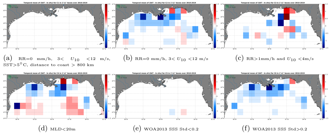
Figure 12: Temporal mean gridded over spatial boxes of size 1^{\circ}\times 1^{\circ} of \Delta\text{SSS} (SMOS SSS L3 v4 - 18 Days (CATDS-CECOS-LOCEAN) - Argo) for 6 different subdatasets corresponding to:RR=0 mm/h, 3 < U_{10} < 12 m/s, SST > 5^{\circ}\text{C} , distance to coast > 800 km (a), RR=0 mm/h, 3 < U_{10} < 12 m/s (b), RR > 1\text{mm/h} and U_{10} < 4\text{m/s} (c),MLD < 20\text{m} (d),WOA2013 SSS Std < 0.2 (e),WOA2013 SSS Std > 0.2 (f).
