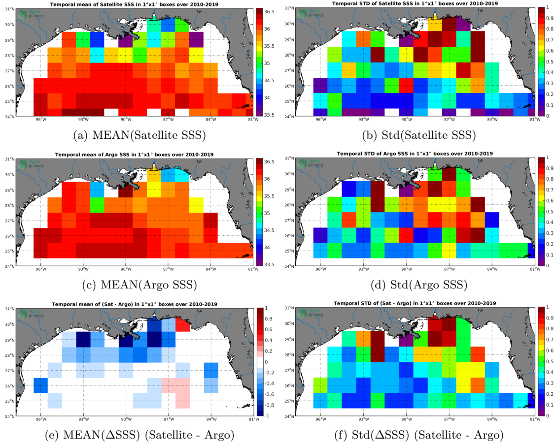
Figure 6: Temporal mean (left) and Std (right) of SSS from SMOS-L3-CATDS-CECOS-LOCEAN-V4-18DAYS-25KM (top), Argo (middle), and of \Delta SSS (Satellite - Argo). Only match-up pairs are used to generate these maps.
