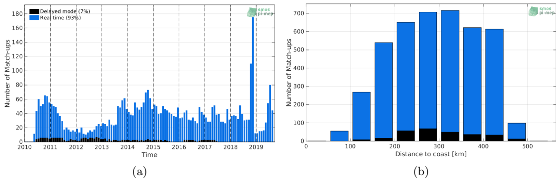
Figure 1: Number of match-ups between Argo and SMOS-L3-CATDS-CECOS-LOCEAN-V4-18DAYS-25KM SSS as a function of time (a) and as function of the distance to coast (b) over the Mississippi river plume Pi-MEP region and for the full satellite product period.
