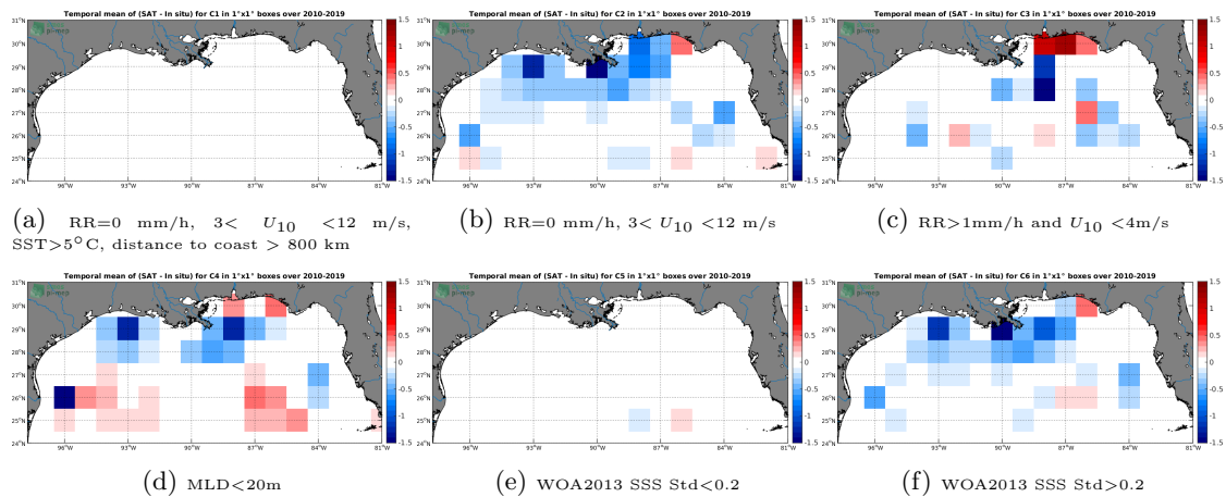
Figure 12: Temporal mean gridded over spatial boxes of size 1^\circ \times 1^\circ of \Delta SSS (SMOS-L3-CATDS-CECOS-LOCEAN-V4-18DAYS-25KM - Argo) for 6 different subdatasets corresponding to:RR=0 mm/h, 3 < U_{10} < 12 m/s, SST >5^\circ\text{C} , distance to coast > 800 km (a), RR=0 mm/h, 3 < U_{10} < 12 m/s (b), RR >1 mm/h and U_{10} < 4 m/s (c),MLD <20 m (d),WOA2013 SSS Std <0.2 (e),WOA2013 SSS Std >0.2 (f).
