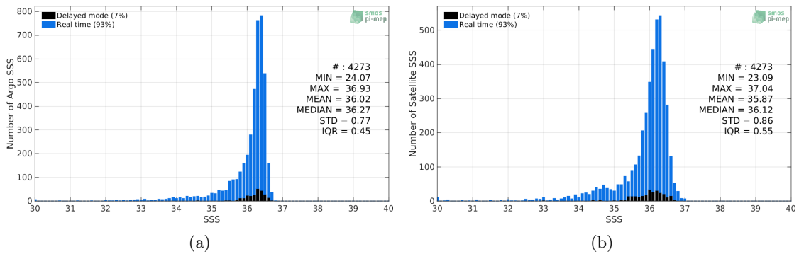
Figure 2: Histograms of SSS from Argo (a) and SMOS-L3-CATDS-CECOS-LOCEAN-V4-18DAYS-25KM (b) considering all match-up pairs per bins of 0.1 over the Mississippi river plume Pi-MEP region and for the full satellite product period.
