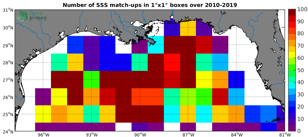
Figure 4: Number of SSS match-ups between Argo SSS and the SMOS-L3-CATDS-CECOS-LOCEAN-V4-18DAYS-25KM SSS product for the Mississippi river plume Pi-MEP region over 1°x1° boxes and for the full satellite product period.
