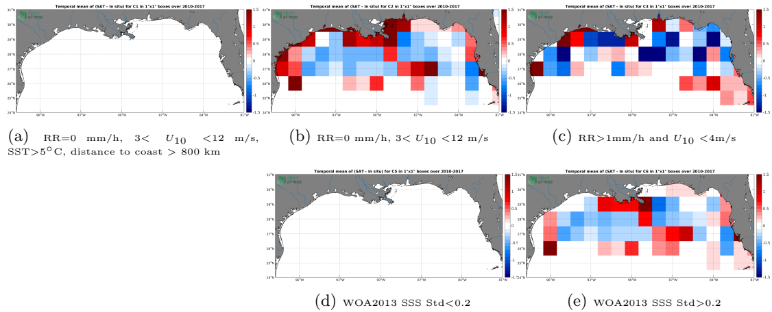
Figure 12: Temporal mean gridded over spatial boxes of size 1^\circ \times 1^\circ of \Delta SSS (SMOS-L3-CATDS-CECOS-LOCEAN-V3-9DAYS-25KM - TSG-SAMOS) for 5 different subdatasets corresponding to: RR=0 mm/h, 3 < U_{10} < 12 m/s, SST >5^\circ C, distance to coast > 800 km (a), RR=0 mm/h, 3 < U_{10} < 12 m/s (b), RR >1 mm/h and U_{10} < 4 m/s (c), WOA2013 SSS Std <0.2 (d), WOA2013 SSS Std >0.2 (e).
