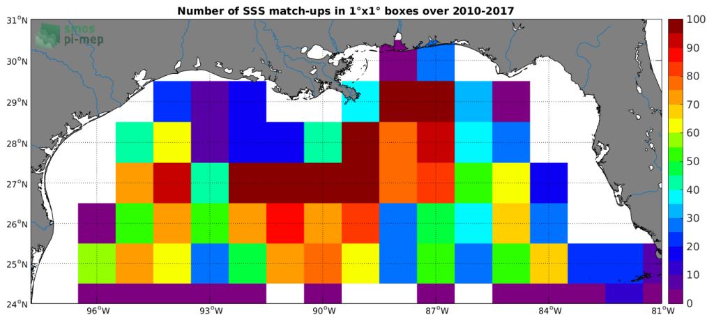
Figure 4: Number of SSS match-ups between Argo SSS and the SMOS-L3-CATDS-CECOS-LOCEAN-V3-9DAYS-25KM SSS product for the Mississippi river plume Pi-MEP region over 1°x1° boxes and for the full satellite product period.
