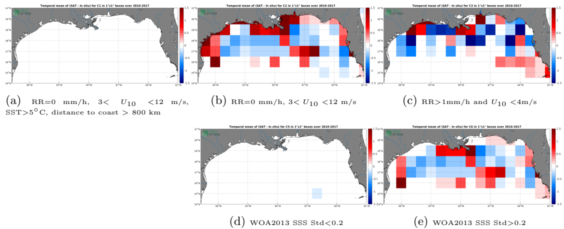
Figure 12: Temporal mean gridded over spatial boxes of size 1^\circ \times 1^\circ of \Delta SSS (SMOS-L3-CATDS-CECOS-LOCEAN-V3-18DAYS-25KM - TSG-SAMOS) for 5 different subdatasets corresponding to: RR=0 mm/h, 3 < U_{10} < 12 m/s, SST > 5^\circ\text{C} , distance to coast > 800 km (a), RR=0 mm/h, 3 < U_{10} < 12 m/s (b), RR > 1 mm/h and U_{10} < 4 m/s (c), WOA2013 SSS Std < 0.2 (d), WOA2013 SSS Std > 0.2 (e).
