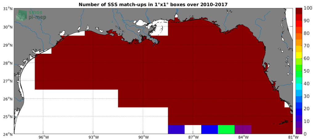
Figure 4: Number of SSS match-ups between TSG-SAMOS SSS and the SMOS-L3-CATDS-CECOS-LOCEAN-V3-18DAYS-25KM SSS product for the Mississippi river plume Pi-MEP region over 1°x1° boxes and for the full satellite product period.
