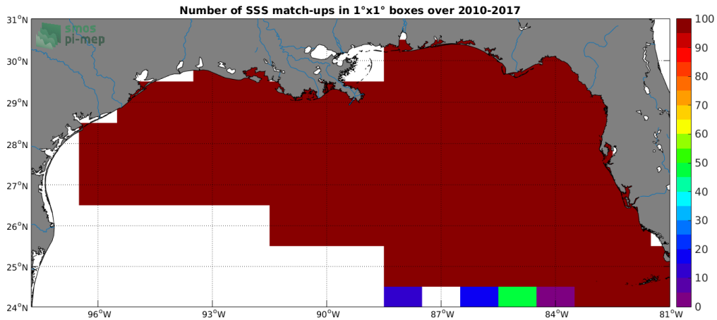
Figure 4: Number of SSS match-ups between TSG-SAMOS SSS and the SMOS-L3-CATDS-CECOS-LOCEAN-V3-18DAYS-25KM SSS product for the Mississippi river plume Pi-MEP region over 1^\circ \times 1^\circ boxes and for the full satellite product period.
