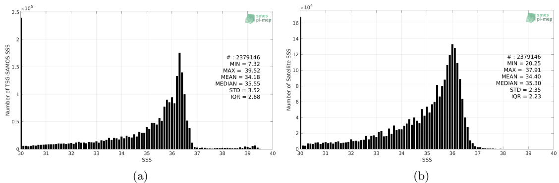
Figure 2: Histograms of SSS from TSG-SAMOS (a) and SMOS-L3-CATDS-CECOS-LOCEAN-V3-18DAYS-25KM (b) considering all match-up pairs per bins of 0.1 over the Mississippi river plume Pi-MEP region and for the full satellite product period.
