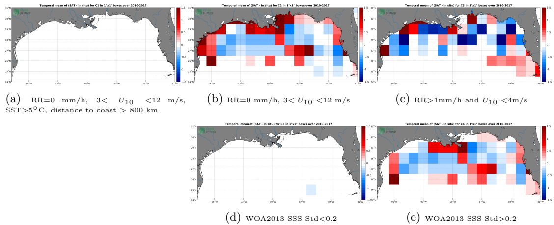
Figure 12: Temporal mean gridded over spatial boxes of size 1^\circ \times 1^\circ of \Delta SSS (SMOS-L3-CATDS-CECOS-LOCEAN-V3-18DAYS-25KM - TSG-SAMOS) for 5 different subdatasets corresponding to:RR=0 mm/h, 3 < U_{10} < 12 m/s, SST >5^\circ C, distance to coast > 800 km (a), RR=0 mm/h, 3 < U_{10} < 12 m/s (b), RR >1 mm/h and U_{10} < 4 m/s (c), WOA2013 SSS Std <0.2 (d), WOA2013 SSS Std >0.2 (e).
