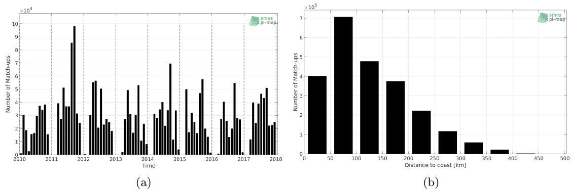
Figure 1: Number of match-ups between TSG-SAMOS and SMOS-L3-CATDS-CECOS-LOCEAN-V3-18DAYS-25KM SSS as a function of time (a) and as function of the distance to coast (b) over the Mississippi river plume Pi-MEP region and for the full satellite product period.
