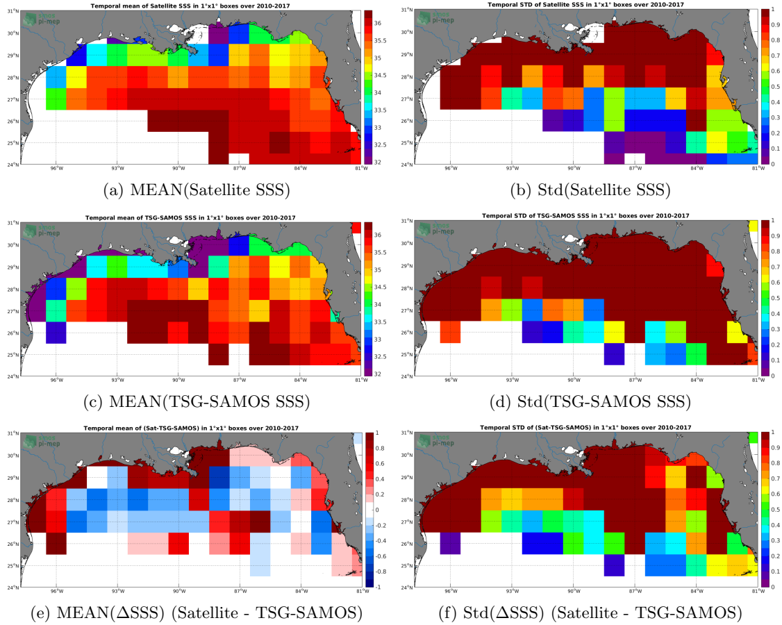
Figure 6: Temporal mean (left) and Std (right) of SSS from SMOS-L3-CATDS-CECOS-LOCEAN-V3-18DAYS-25KM (top), TSG-SAMOS (middle), and of \Delta SSS (Satellite - TSG-SAMOS). Only match-up pairs are used to generate these maps.
