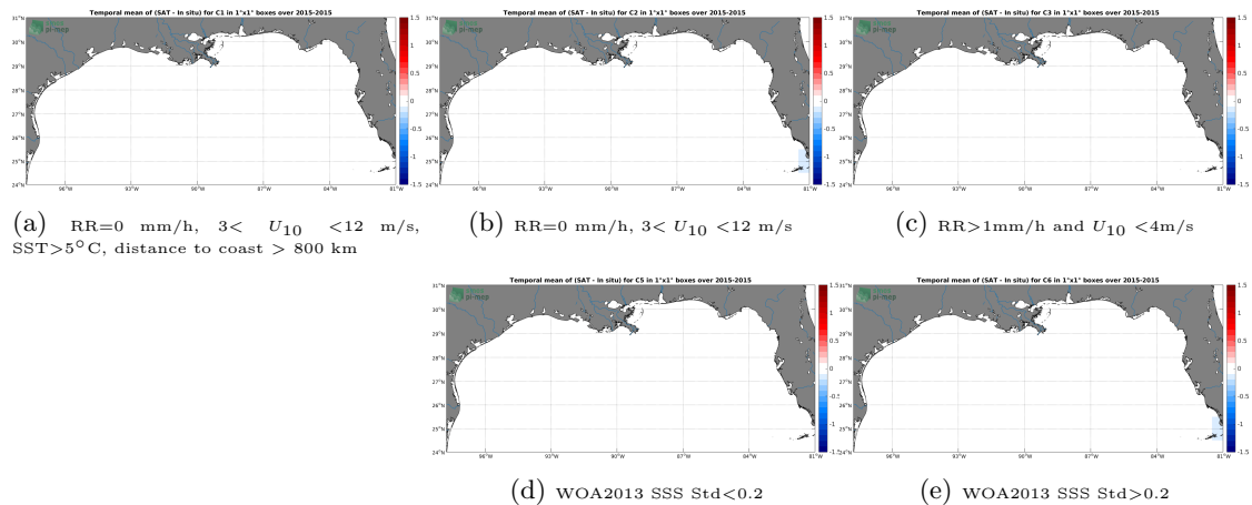
Figure 12: Temporal mean gridded over spatial boxes of size 1^\circ \times 1^\circ of \Delta SSS (SMOS-L3-CATDS-CECOS-LOCEAN-V3-18DAYS-25KM - TSG-GOSUD-Sailing-ship) for 5 different subdatasets corresponding to:RR=0 mm/h, 3 < U_{10} < 12 m/s, SST >5^\circ\text{C} , distance to coast > 800 km (a), RR=0 mm/h, 3 < U_{10} < 12 m/s (b), RR >1 mm/h and U_{10} < 4 m/s (c), WOA2013 SSS Std <0.2 (d), WOA2013 SSS Std >0.2 (e).
