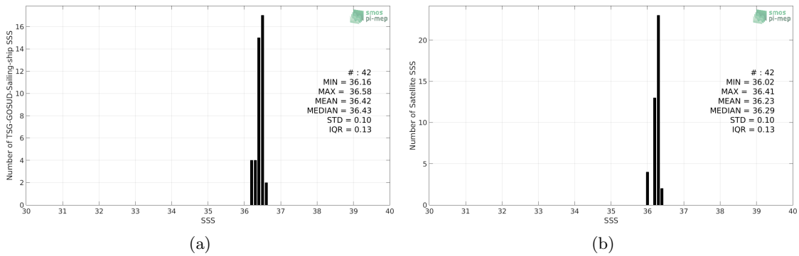
Figure 2: Histograms of SSS from TSG-GOSUD-Sailing-ship (a) and SMOS-L3-CATDS-CECOS-LOCEAN-V3-18DAYS-25KM (b) considering all match-up pairs per bins of 0.1 over the Mississippi river plume Pi-MEP region and for the full satellite product period.
