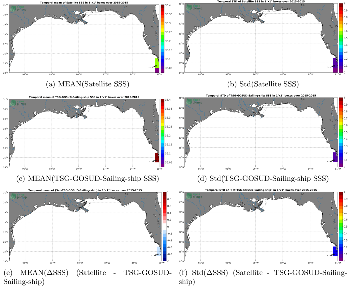
Figure 6: Temporal mean (left) and Std (right) of SSS from SMOS-L3-CATDS-CECOS-LOCEAN-V3-18DAYS-25KM (top), TSG-GOSUD-Sailing-ship (middle), and of \Delta SSS (Satellite - TSG-GOSUD-Sailing-ship). Only match-up pairs are used to generate these maps.
