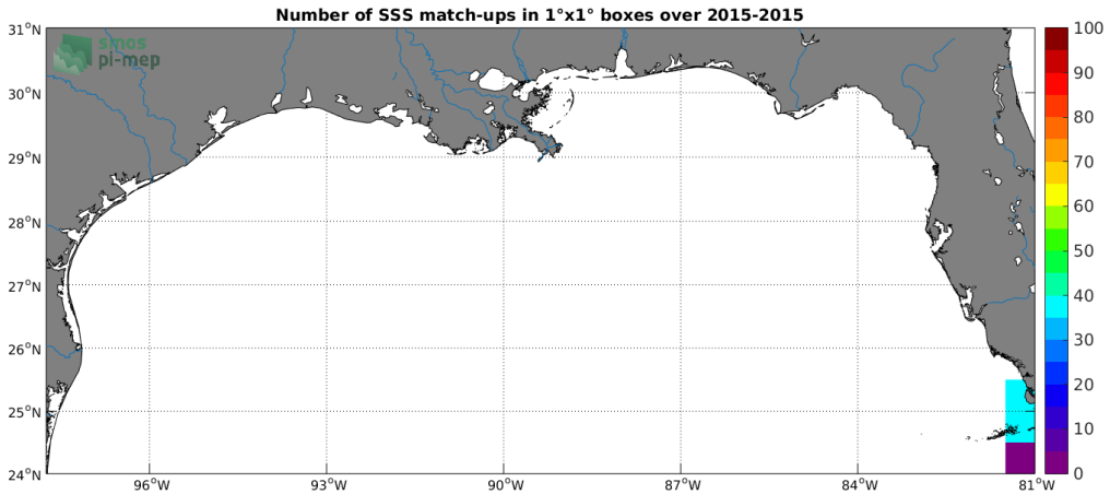
Figure 4: Number of SSS match-ups between TSG-GOSUD-Sailing-ship SSS and the SMOS-L3-CATDS-CECOS-LOCEAN-V3-18DAYS-25KM SSS product for the Mississippi river plume Pi-MEP region over 1^{\circ} \times 1^{\circ} boxes and for the full satellite product period.
