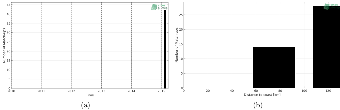
Figure 1: Number of match-ups between TSG-GOSUD-Sailing-ship and SMOS-L3-CATDS-CECOS-LOCEAN-V3-18DAYS-25KM SSS as a function of time (a) and as function of the distance to coast (b) over the Mississippi river plume Pi-MEP region and for the full satellite product period.
