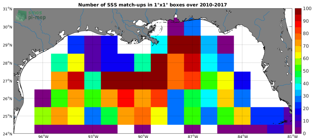
Figure 4: Number of SSS match-ups between Argo SSS and the SMOS-L3-CATDS-CECOS-LOCEAN-V3-18DAYS-25KM SSS product for the Mississippi river plume Pi-MEP region over 1°x1° boxes and for the full satellite product period.
