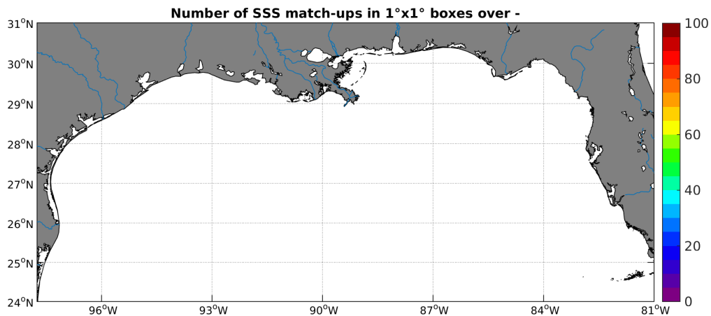
Figure 4: Number of SSS match-ups between TSG-LEGOS-DM SSS and the SMOS-L3-CATDS-CECOS-LOCEAN-V2.1-9DAYS-25KM SSS product for the Mississippi river plume Pi-MEP region over 1^\circ \times 1^\circ boxes and for the full satellite product period.
