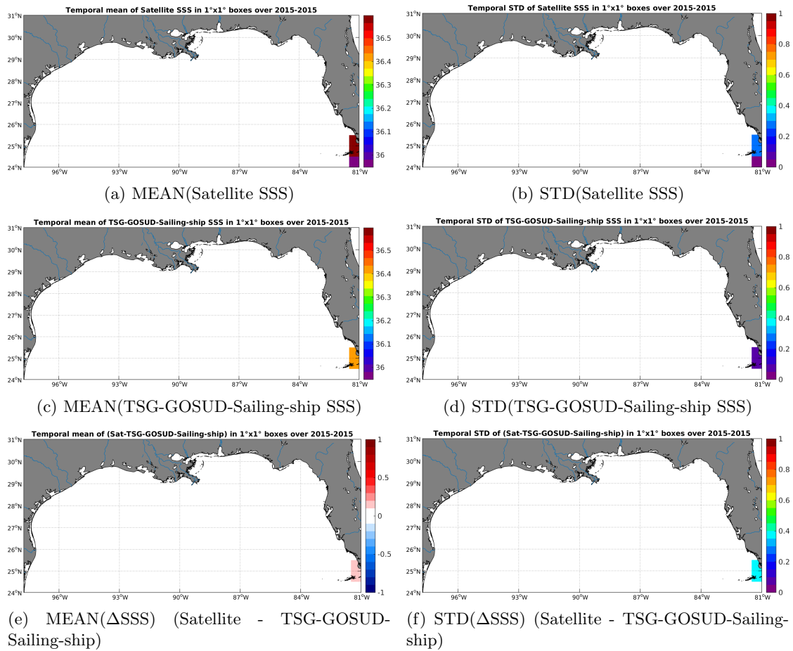
Figure 6: Temporal mean (left) and STD (right) of SSS from SMOS-L3-CATDS-CECOS-LOCEAN-V2.1-9DAYS-25KM (top), TSG-GOSUD-Sailing-ship (middle), and of \Delta SSS (Satellite - TSG-GOSUD-Sailing-ship). Only match-up pairs are used to generate these maps.
