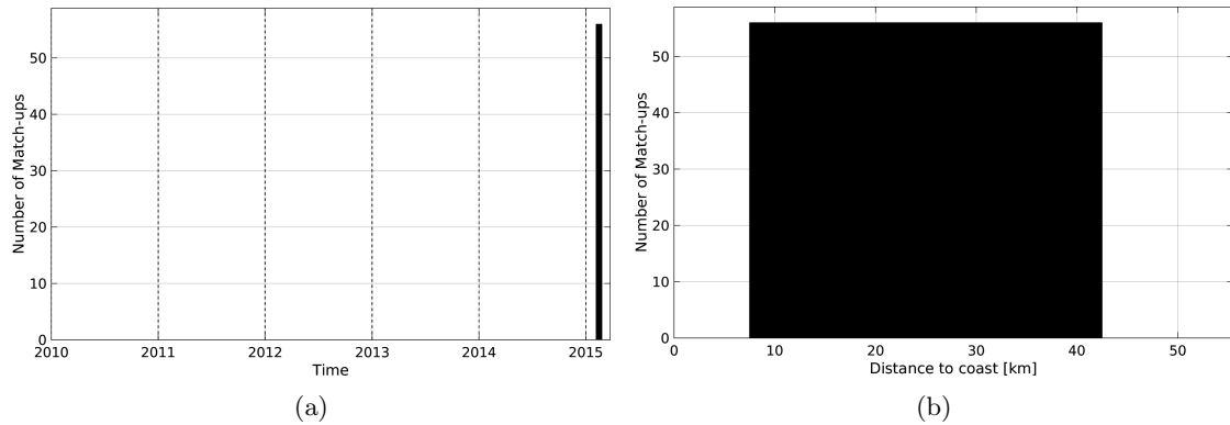
Figure 1: Number of match-ups between TSG-GOSUD-Sailing-ship and SMOS-L3-CATDS-CECOS-LOCEAN-V2.1-9DAYS-25KM SSS as a function of time (a) and as function of the distance to coast (b) over the Mississippi river plume Pi-MEP region and for the full satellite product period.
