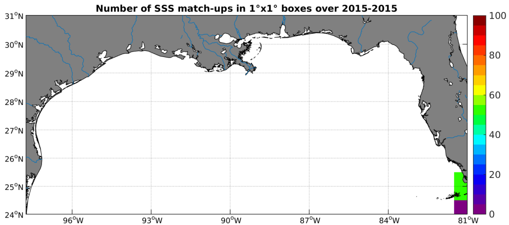
Figure 4: Number of SSS match-ups between TSG-GOSUD-Sailing-ship SSS and the SMOS-L3-CATDS-CECOS-LOCEAN-V2.1-9DAYS-25KM SSS product for the Mississippi river plume Pi-MEP region over 1^{\circ} \times 1^{\circ} boxes and for the full satellite product period.
