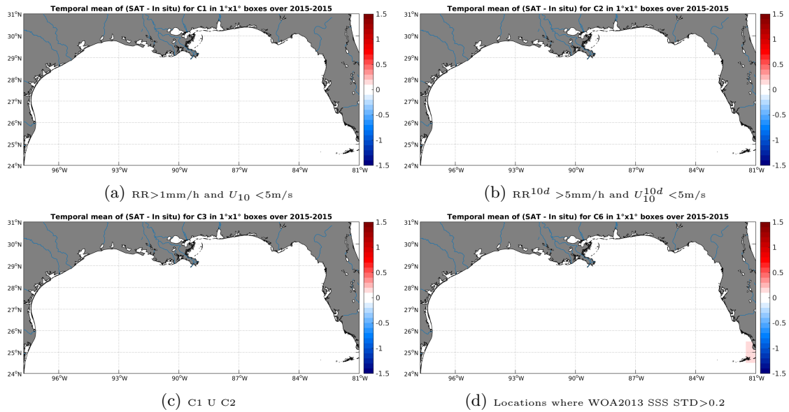
Figure 12: Temporal mean gridded over spatial boxes of size 1^\circ \times 1^\circ of \Delta SSS (SMOS-L3-CATDS-CECOS-LOCEAN-V2.1-9DAYS-25KM - TSG-GOSUD-Sailing-ship) for 4 different subdatasets corresponding to:RR >1 mm/h and U_{10} < 5 m/s (a), RR^{10d} > 5 mm/h and U_{10}^{10d} < 5 m/s (b), C1 U C2 (c),Locations where WOA2013 SSS STD >0.2 (d).
