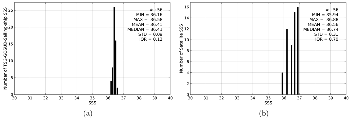
Figure 2: Histograms of SSS from TSG-GOSUD-Sailing-ship (a) and SMOS-L3-CATDS-CECOS-LOCEAN-V2.1-9DAYS-25KM (b) considering all match-up pairs per bins of 0.1 over the Mississippi river plume Pi-MEP region and for the full satellite product period.
