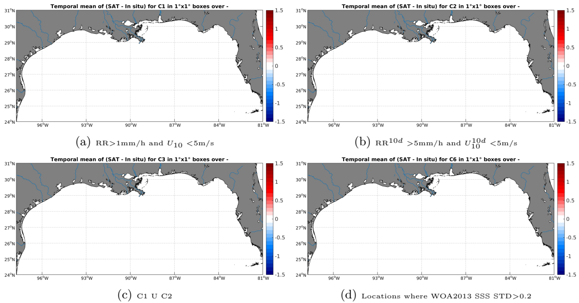
Figure 12: Temporal mean gridded over spatial boxes of size 1^\circ \times 1^\circ of \Delta SSS (SMOS-L3-CATDS-CECOS-LOCEAN-V2.1-9DAYS-25KM - TSG-GOSUD-Research-vessel) for 4 different subdatasets corresponding to:RR > 1 mm/h and U_{10} < 5 m/s (a), RR^{10d} > 5 mm/h and U_{10}^{10d} < 5 m/s (b), C1 U C2 (c),Locations where WOA2013 SSS STD > 0.2 (d).
