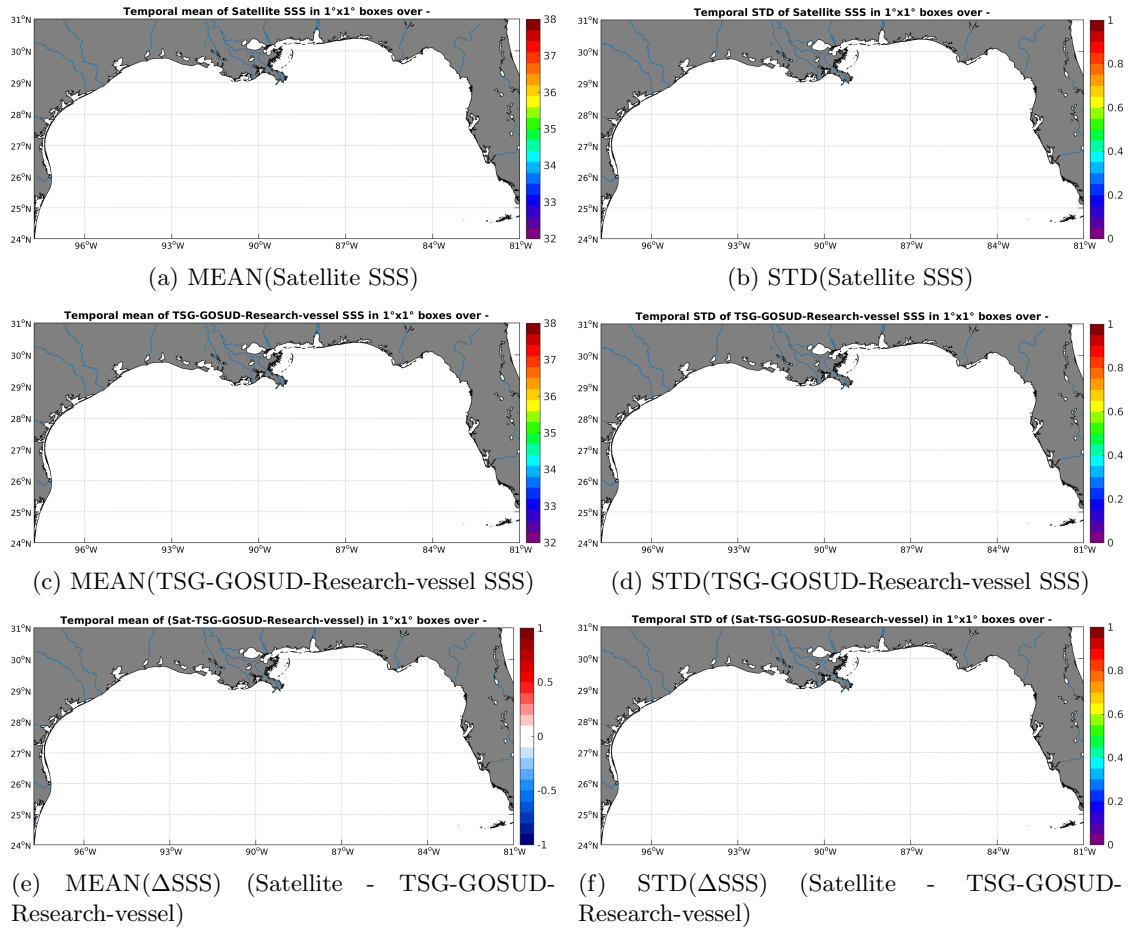
Figure 6: Temporal mean (left) and STD (right) of SSS from SMOS-L3-CATDS-CECOS-LOCEAN-V2.1-9DAYS-25KM (top), TSG-GOSUD-Research-vessel (middle), and of \Delta SSS (Satellite - TSG-GOSUD-Research-vessel). Only match-up pairs are used to generate these maps.
