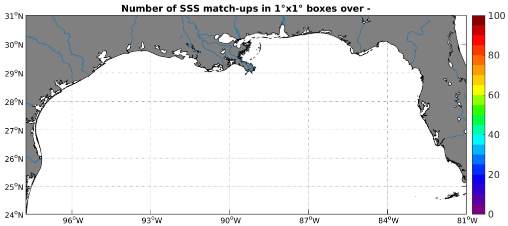
Figure 4: Number of SSS match-ups between Sea mammals SSS and the SMOS-L3-CATDS-CECOS-LOCEAN-V2.1-9DAYS-25KM SSS product for the Mississippi river plume Pi-MEP region over 1^\circ \times 1^\circ boxes and for the full satellite product period.
