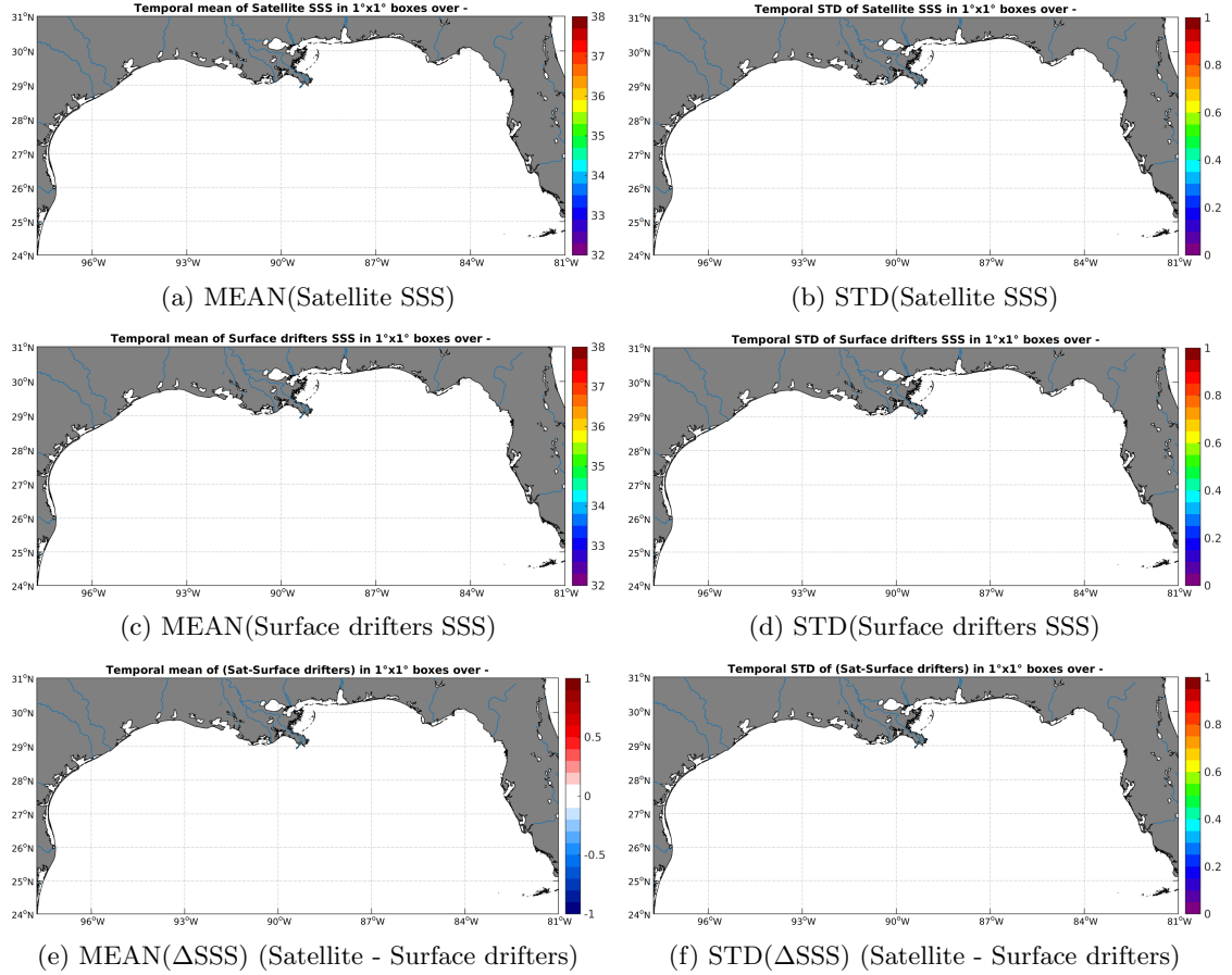
Figure 5: Temporal mean (left) and STD (right) of SSS from SMOS-L3-CATDS-CECOS-LOCEAN-V2.1-9DAYS-25KM (top), Surface drifters (middle), and of \Delta SSS (Satellite - Surface drifters). Only match-up pairs are used to generate these maps.
