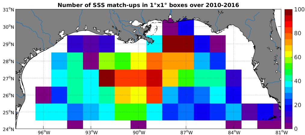
Figure 4: Number of SSS match-ups between Argo SSS and the SMOS-L3-CATDS-CECOS-LOCEAN-V2.1-9DAYS-25KM SSS product for the Mississippi river plume Pi-MEP region over 1^{\circ} \times 1^{\circ} boxes and for the full satellite product period.
