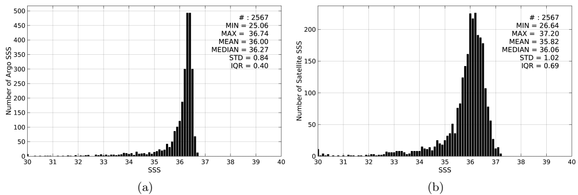
Figure 2: Histograms of SSS from Argo (a) and SMOS-L3-CATDS-CECOS-LOCEAN-V2.1-9DAYS-25KM (b) considering all match-up pairs per bins of 0.1 over the Mississippi river plume Pi-MEP region and for the full satellite product period.
