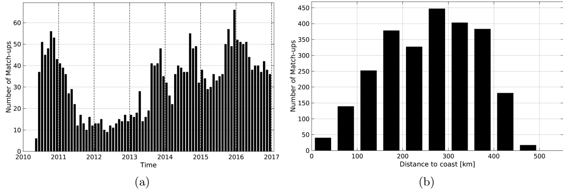
Figure 1: Number of match-ups between Argo and SMOS-L3-CATDS-CECOS-LOCEAN-V2.1-9DAYS-25KM SSS as a function of time (a) and as function of the distance to coast (b) over the Mississippi river plume Pi-MEP region and for the full satellite product period.
