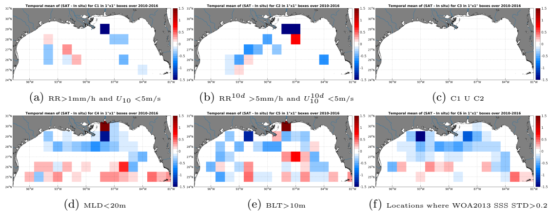
Figure 12: Temporal mean gridded over spatial boxes of size 1^\circ \times 1^\circ of \Delta SSS (SMOS-L3-CATDS-CECOS-LOCEAN-V2.1-9DAYS-25KM - Argo) for 6 different subdatasets corresponding to: RR > 1\text{mm/h} and U_{10} < 5\text{m/s} (a), RR^{10d} > 5\text{mm/h} and U_{10}^{10d} < 5\text{m/s} (b), C1 U C2 (c), MLD < 20\text{m} (d), BLT > 10\text{m} (e), Locations where WOA2013 SSS STD > 0.2 (f).
