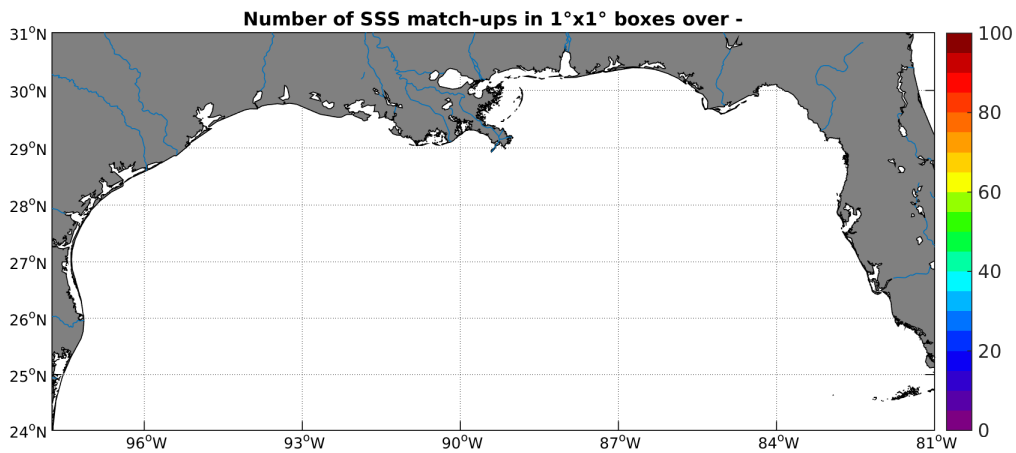
Figure 4: Number of SSS match-ups between TSG-GOSUD-Research-vessel SSS and the SMOS-L3-CATDS-CECOS-LOCEAN-V2-9DAYS-25KM SSS product for the Mississippi river plume Pi-MEP region over 1^{\circ} \times 1^{\circ} boxes and for the full satellite product period.
