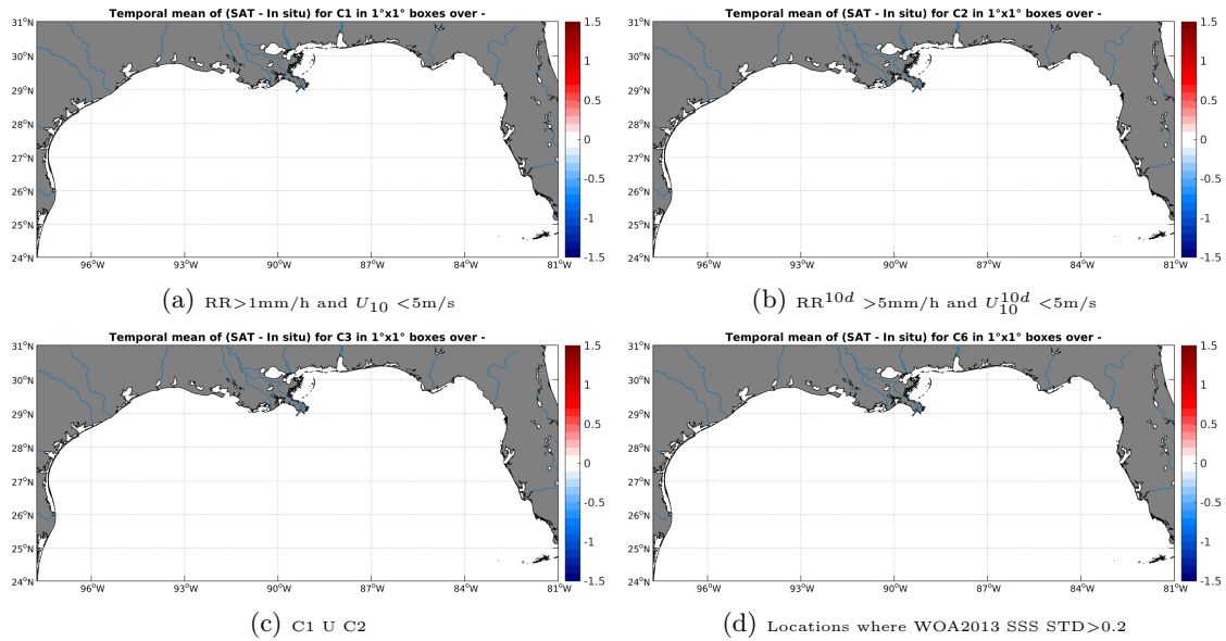
Figure 12: Temporal mean gridded over spatial boxes of size 1^\circ \times 1^\circ of \Delta SSS (SMOS-L3-CATDS-CECOS-LOCEAN-V2-9DAYS-25KM - TSG-GOSUD-Research-vessel) for 4 different subdatasets corresponding to:RR >1 mm/h and U_{10} < 5 m/s (a), RR ^{10d} > 5 mm/h and U_{10}^{10d} < 5 m/s (b), C1 U C2 (c),Locations where WOA2013 SSS STD >0.2 (d).
