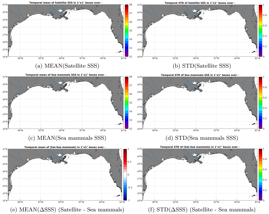
Figure 6: Temporal mean (left) and STD (right) of SSS from SMOS-L3-CATDS-CECOS-LOCEAN-V2-9DAYS-25KM (top), Sea mammals (middle), and of \Delta SSS (Satellite - Sea mammals). Only match-up pairs are used to generate these maps.
