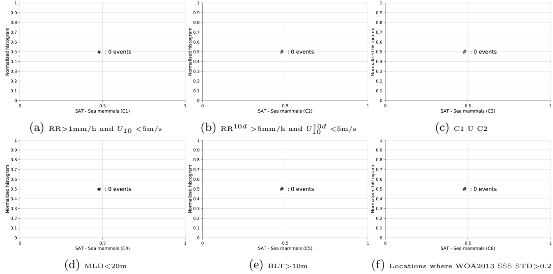
Figure 13: Normalized histogram of \Delta\text{SSS} (SMOS-L3-CATDS-CECOS-LOCEAN-V2-9DAYS-25KM - Sea mammals) for 6 different subdatasets corresponding to: RR > 1\text{mm/h} and U_{10} < 5\text{m/s} (a), RR^{10d} > 5\text{mm/h} and U_{10}^{10d} < 5\text{m/s} (b), C1 \cup C2 (c), MLD < 20\text{m} (d), BLT > 10\text{m} (e), Locations where WOA2013 SSS STD > 0.2 (f).
