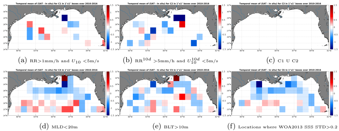
Figure 12: Temporal mean gridded over spatial boxes of size 1^\circ \times 1^\circ of \Delta SSS (SMOS-L3-CATDS-CECOS-LOCEAN-V2-9DAYS-25KM - Argo) for 6 different subdatasets corresponding to: RR > 1\text{mm/h} and U_{10} < 5\text{m/s} (a), RR^{10d} > 5\text{mm/h} and U_{10}^{10d} < 5\text{m/s} (b), C1 U C2 (c), MLD < 20\text{m} (d), BLT > 10\text{m} (e), Locations where WOA2013 SSS STD > 0.2 (f).
