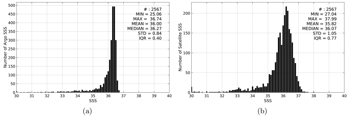
Figure 2: Histograms of SSS from Argo (a) and SMOS-L3-CATDS-CECOS-LOCEAN-V2-9DAYS-25KM (b) considering all match-up pairs per bins of 0.1 over the Mississippi river plume Pi-MEP region and for the full satellite product period.
