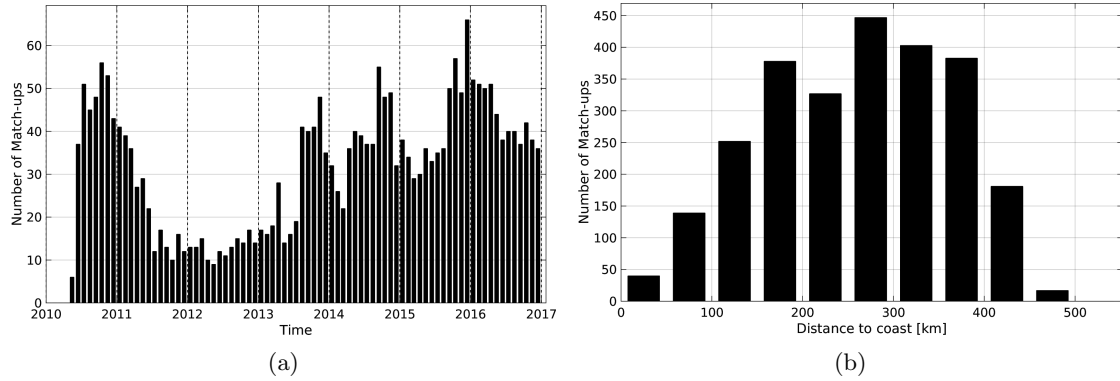
Figure 1: Number of match-ups between Argo and SMOS-L3-CATDS-CECOS-LOCEAN-V2-9DAYS-25KM SSS as a function of time (a) and as function of the distance to coast (b) over the Mississippi river plume Pi-MEP region and for the full satellite product period.
