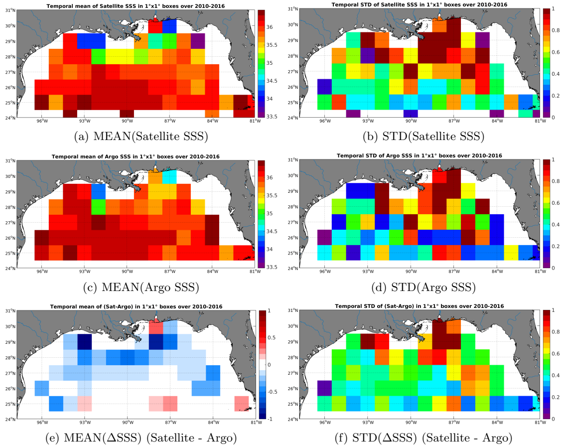
Figure 6: Temporal mean (left) and STD (right) of SSS from SMOS-L3-CATDS-CECOS-LOCEAN-V2-9DAYS-25KM (top), Argo (middle), and of \Delta SSS (Satellite - Argo). Only match-up pairs are used to generate these maps.
