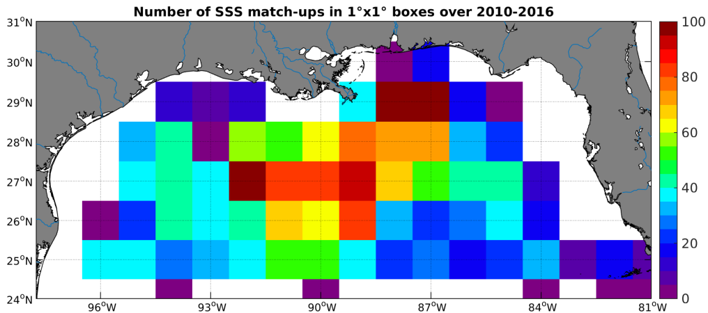
Figure 4: Number of SSS match-ups between Argo SSS and the SMOS-L3-CATDS-CECOS-LOCEAN-V2-9DAYS-25KM SSS product for the Mississippi river plume Pi-MEP region over 1^{\circ} \times 1^{\circ} boxes and for the full satellite product period.
