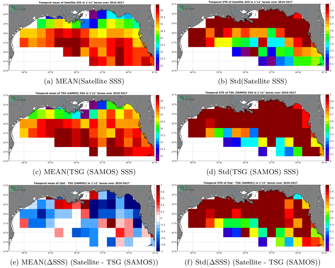
Figure 6: Temporal mean (left) and Std (right) of SSS from SMOS SSS L3 v2 - Monthly - 0.25 Deg (CATDS-CECOS-IFREMER) (top), TSG (SAMOS) ( in situ ) (middle), and of \Delta SSS (Satellite - TSG (SAMOS)). Only match-up pairs are used to generate these maps.
