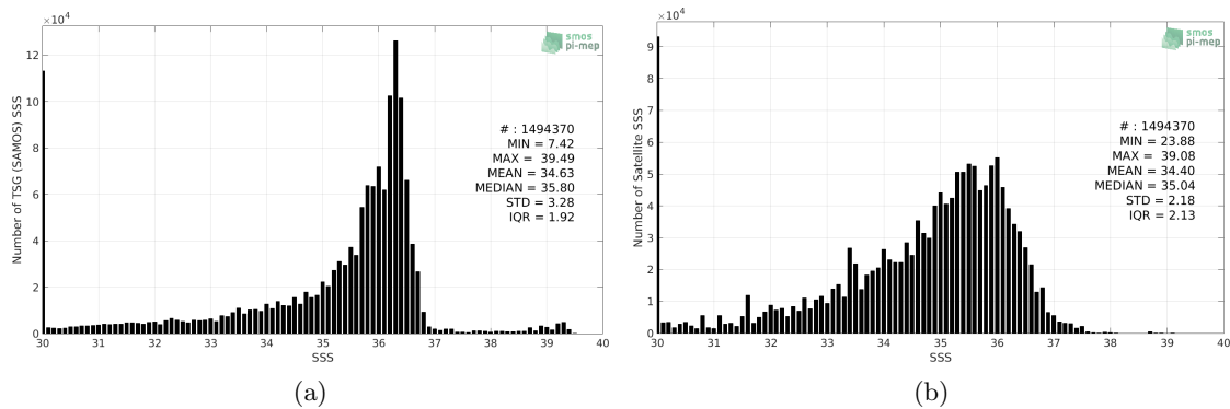
Figure 2: Histograms of SSS from TSG (SAMOS) (a) and SMOS SSS L3 v2 - Monthly - 0.25 Deg (CATDS-CECOS-IFREMER) (b) considering all match-up pairs per bins of 0.1 over the Mississippi river plume Pi-MEP region and for the full satellite product period.
