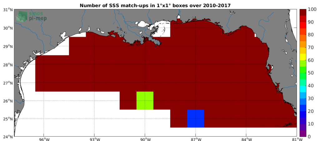
Figure 4: Number of SSS match-ups between TSG (SAMOS) SSS and the SMOS SSS L3 v2 - Monthly - 0.25 Deg (CATDS-CECOS-IFREMER) SSS product for the Mississippi river plume Pi-MEP region over 1^\circ \times 1^\circ boxes and for the full satellite product period.
