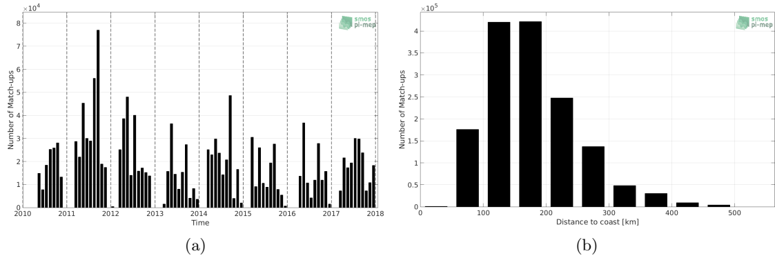
Figure 1: Number of match-ups between TSG (SAMOS) and SMOS SSS L3 v2 - Monthly - 0.25 Deg (CATDS-CECOS-IFREMER) SSS as a function of time (a) and as function of the distance to coast (b) over the Mississippi river plume Pi-MEP region and for the full satellite product period.
