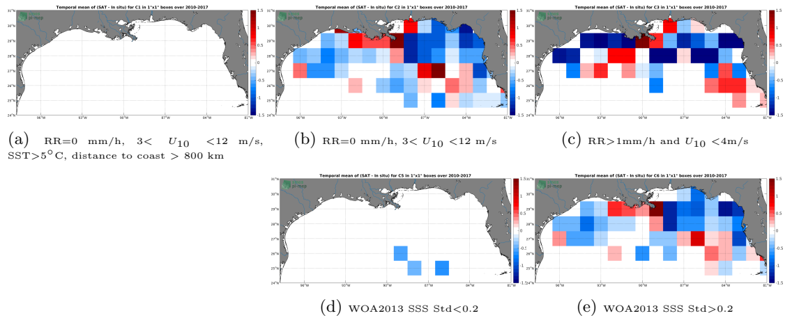
Figure 12: Temporal mean gridded over spatial boxes of size 1^{\circ}\times 1^{\circ} of \Delta\text{SSS} (SMOS SSS L3 v2 - Monthly - 0.25 Deg (CATDS-CECOS-IFREMER) - TSG (SAMOS)) for 5 different subdatasets corresponding to:RR=0 mm/h, 3 < U_{10} < 12 m/s, SST >5^{\circ}\text{C} , distance to coast > 800 km (a), RR=0 mm/h, 3 < U_{10} < 12 m/s (b), RR >1 mm/h and U_{10} < 4 m/s (c), WOA2013 SSS Std <0.2 (d), WOA2013 SSS Std >0.2 (e).
