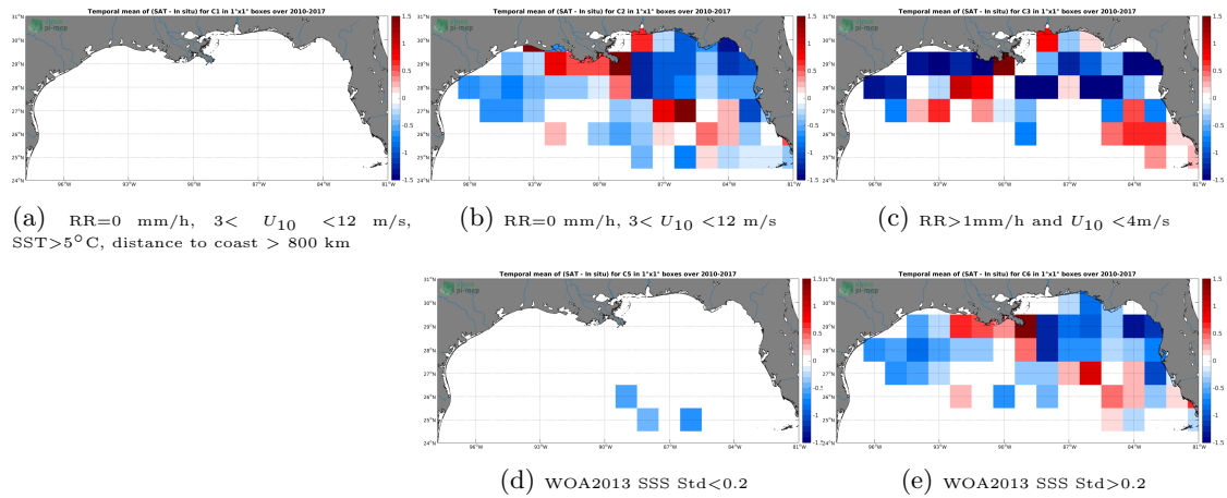
Figure 12: Temporal mean gridded over spatial boxes of size 1^{\circ}\times 1^{\circ} of \Delta\text{SSS} (SMOS L3 v2 - Monthly - 0.25 Deg (CATDS-CECOS-IFREMER) - TSG-SAMOS) for 5 different subdatasets corresponding to:RR=0 mm/h, 3 < U_{10} < 12 m/s, SST >5^{\circ}\text{C} , distance to coast > 800 km (a), RR=0 mm/h, 3 < U_{10} < 12 m/s (b), RR >1 mm/h and U_{10} < 4 m/s (c), WOA2013 SSS Std <0.2 (d), WOA2013 SSS Std >0.2 (e).
