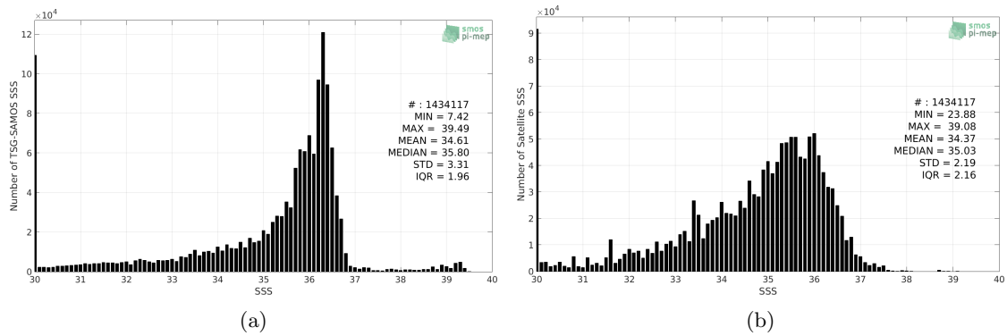
Figure 2: Histograms of SSS from TSG-SAMOS (a) and SMOS L3 v2 - Monthly - 0.25 Deg (CATDS-CECOS-IFREMER) (b) considering all match-up pairs per bins of 0.1 over the Mississippi river plume Pi-MEP region and for the full satellite product period.
