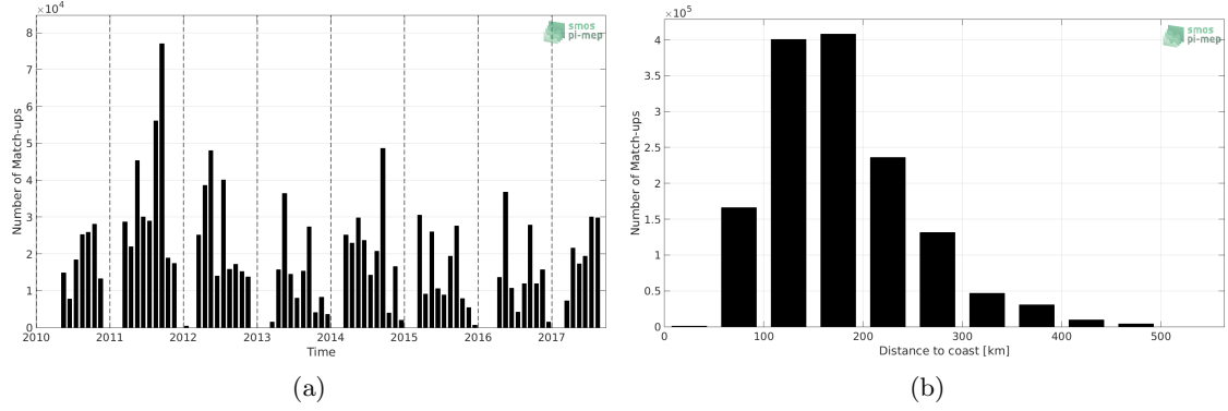
Figure 1: Number of match-ups between TSG-SAMOS and SMOS L3 v2 - Monthly - 0.25 Deg (CATDS-CECOS-IFREMER) SSS as a function of time (a) and as function of the distance to coast (b) over the Mississippi river plume Pi-MEP region and for the full satellite product period.
