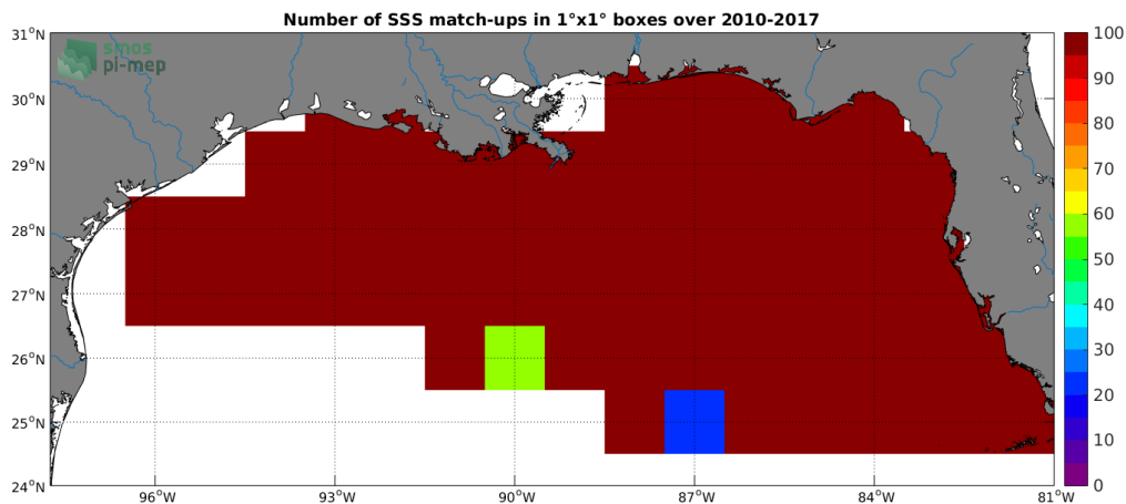
Figure 4: Number of SSS match-ups between TSG-SAMOS SSS and the SMOS L3 v2 - Monthly - 0.25 Deg (CATDS-CECOS-IFREMER) SSS product for the Mississippi river plume Pi-MEP region over 1^\circ \times 1^\circ boxes and for the full satellite product period.
