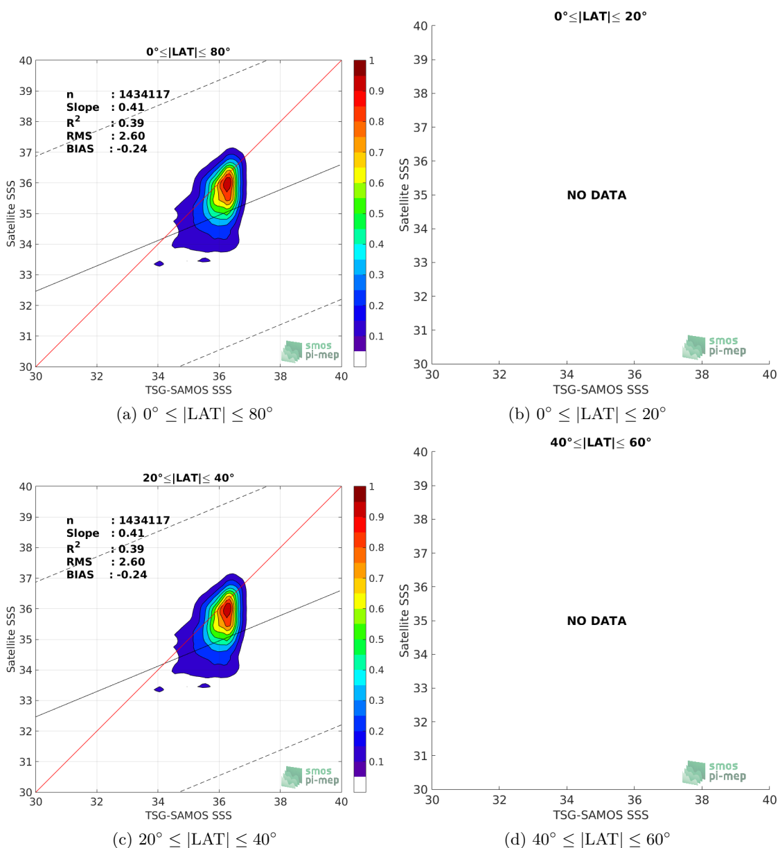
Figure 9: Contour maps of the concentration of SMOS L3 v2 - Monthly - 0.25 Deg (CATDS-CECOS-IFREMER) SSS (y-axis) versus TSG-SAMOS SSS (x-axis) at match-up pairs for different latitude bands. For each plot, the red line shows x=y . The black thin and dashed lines indicate a linear fit through the data cloud and the \pm 95\% confidence levels, respectively. The number match-up pairs n , the slope and R^2 coefficient of the linear fit, the root mean square (RMS) and the mean bias between satellite and in situ data are indicated for each latitude band in each plots.
