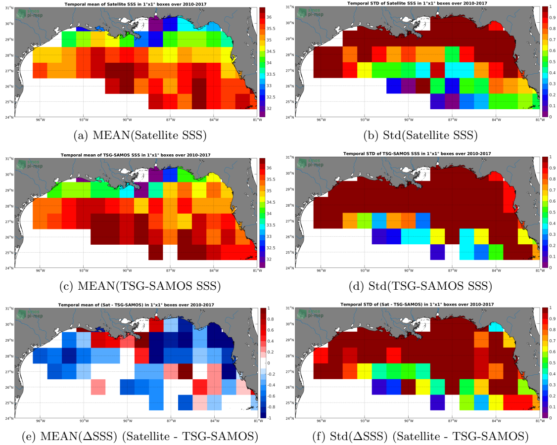
Figure 6: Temporal mean (left) and Std (right) of SSS from SMOS L3 v2 - Monthly - 0.25 Deg (CATDS-CECOS-IFREMER) (top), TSG-SAMOS (middle), and of \Delta SSS (Satellite - TSG-SAMOS). Only match-up pairs are used to generate these maps.
