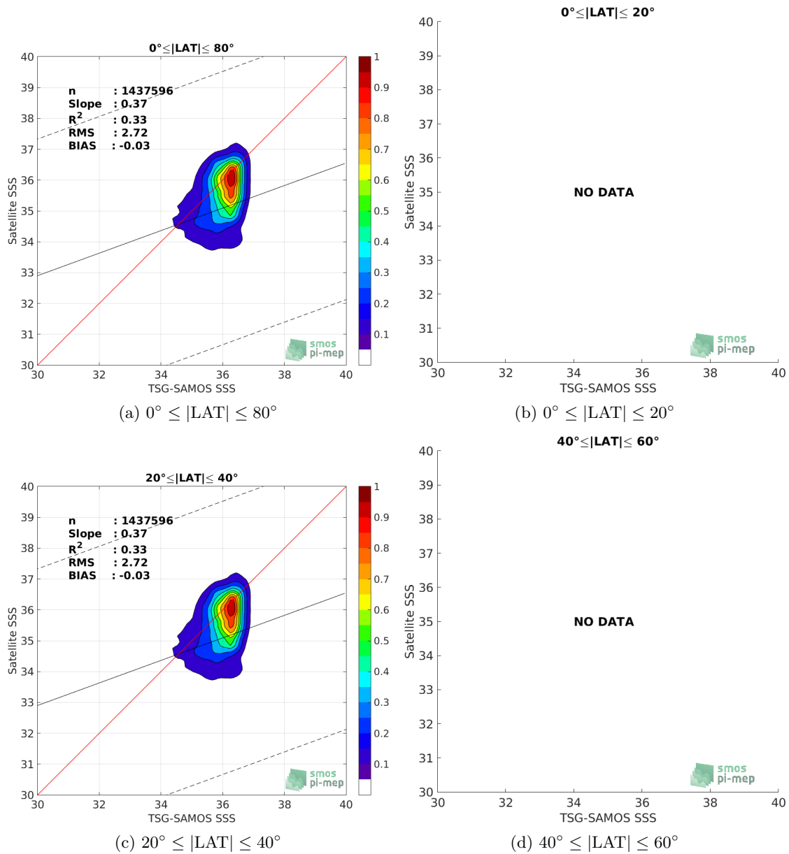
Figure 9: Contour maps of the concentration of SMOS-L3-CATDS-IFREMER-CECOS-V2-MONTHLY-0.25DEG SSS (y-axis) versus TSG-SAMOS SSS (x-axis) at match-up pairs for different latitude bands. For each plot, the red line shows x=y . The black thin and dashed lines indicate a linear fit through the data cloud and the \pm 95\% confidence levels, respectively. The number match-up pairs n , the slope and R^2 coefficient of the linear fit, the root mean square (RMS) and the mean bias between satellite and in situ data are indicated for each latitude band in each plots.
