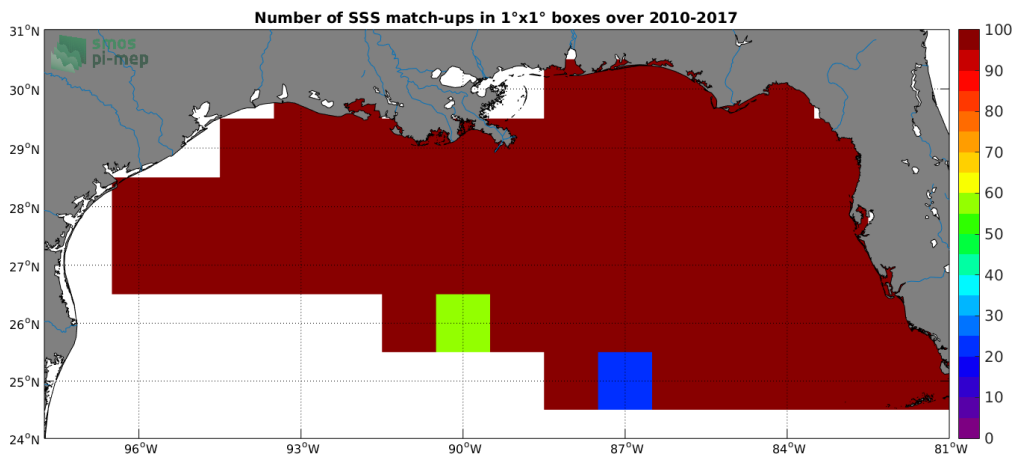
Figure 4: Number of SSS match-ups between TSG-SAMOS SSS and the SMOS-L3-CATDS-IFREMER-CECOS-V2-MONTHLY-0.25DEG SSS product for the Mississippi river plume Pi-MEP region over 1^\circ \times 1^\circ boxes and for the full satellite product period.
