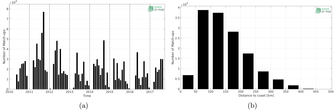
Figure 1: Number of match-ups between TSG-SAMOS and SMOS-L3-CATDS-IFREMER-CECOS-V2-MONTHLY-0.25DEG SSS as a function of time (a) and as function of the distance to coast (b) over the Mississippi river plume Pi-MEP region and for the full satellite product period.
