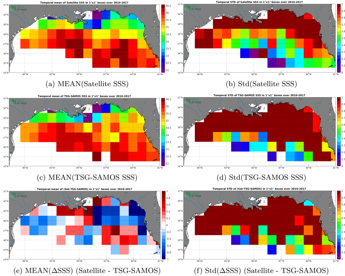
Figure 6: Temporal mean (left) and Std (right) of SSS from SMOS-L3-CATDS-IFREMER-CECOS-V2-MONTHLY-0.25DEG (top), TSG-SAMOS (middle), and of \Delta SSS (Satellite - TSG-SAMOS). Only match-up pairs are used to generate these maps.
