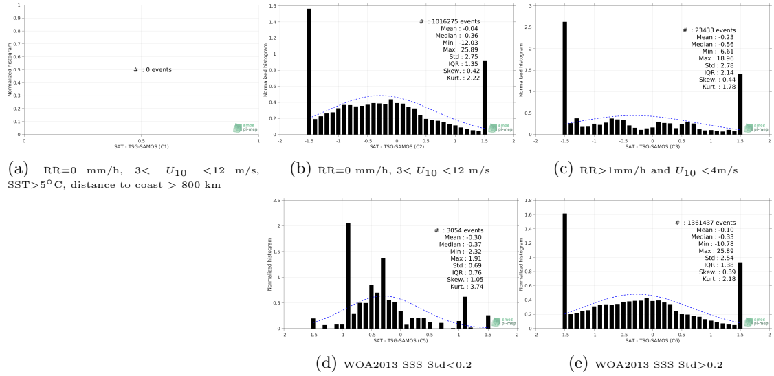
Figure 13: Normalized histogram of \Delta SSS (SMOS-L3-CATDS-IFREMER-CECOS-V2-MONTHLY-0.25DEG - TSG-SAMOS) for 5 different subdatasets corresponding to: RR=0 mm/h, 3 < U_{10} < 12 m/s, SST > 5°C, distance to coast > 800 km (a), RR=0 mm/h, 3 < U_{10} < 12 m/s (b), RR > 1mm/h and U_{10} < 4 m/s (c), WOA2013 SSS Std < 0.2 (d), WOA2013 SSS Std > 0.2 (e).
