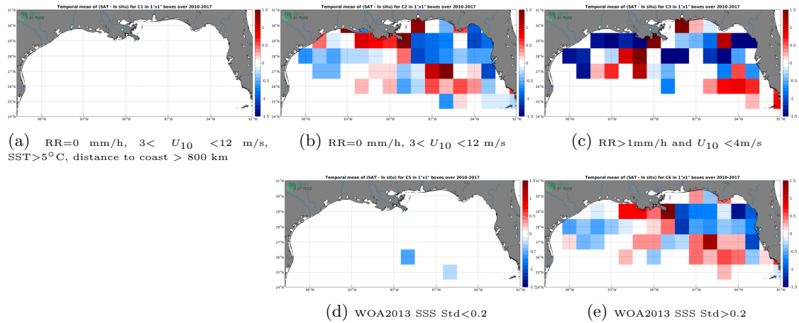
Figure 12: Temporal mean gridded over spatial boxes of size 1^\circ \times 1^\circ of \Delta SSS (SMOS-L3-CATDS-IFREMER-CECOS-V2-MONTHLY-0.25DEG - TSG-SAMOS) for 5 different subdatasets corresponding to:RR=0 mm/h, 3 < U_{10} < 12 m/s, SST >5^\circ C, distance to coast > 800 km (a), RR=0 mm/h, 3 < U_{10} < 12 m/s (b), RR >1 mm/h and U_{10} < 4 m/s (c), WOA2013 SSS Std <0.2 (d), WOA2013 SSS Std >0.2 (e).
