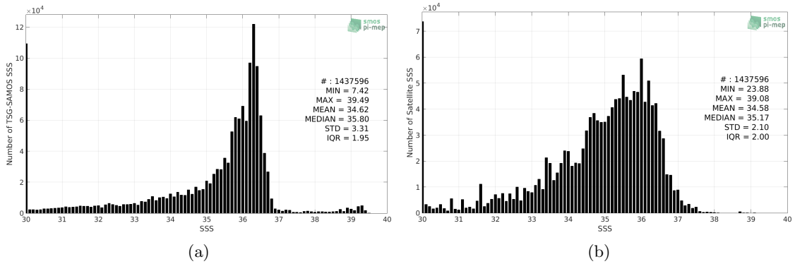
Figure 2: Histograms of SSS from TSG-SAMOS (a) and SMOS-L3-CATDS-IFREMER-CECOS-V2-MONTHLY-0.25DEG (b) considering all match-up pairs per bins of 0.1 over the Mississippi river plume Pi-MEP region and for the full satellite product period.
