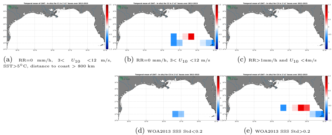
Figure 12: Temporal mean gridded over spatial boxes of size 1^{\circ}\times 1^{\circ} of \Delta SSS (SMOS SSS L3 v2 - Monthly - 0.25 Deg (CATDS-CECOS-IFREMER) - TSG (GOSUD-Sailing-ship)) for 5 different subdatasets corresponding to: RR=0 mm/h, 3 < U_{10} < 12 m/s, SST > 5^{\circ}\text{C} , distance to coast > 800 km (a), RR=0 mm/h, 3 < U_{10} < 12 m/s (b), RR > 1 mm/h and U_{10} < 4 m/s (c), WOA2013 SSS Std < 0.2 (d), WOA2013 SSS Std > 0.2 (e).
