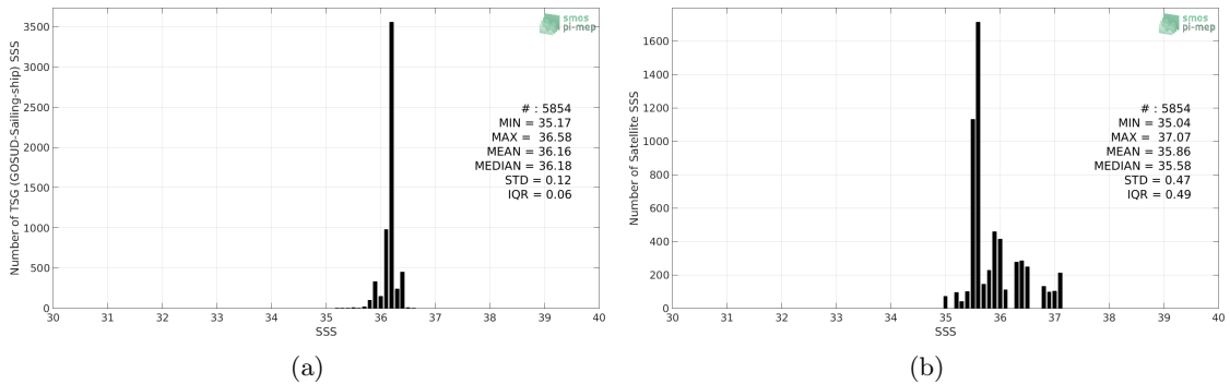
Figure 2: Histograms of SSS from TSG (GOSUD-Sailing-ship) (a) and SMOS SSS L3 v2 - Monthly - 0.25 Deg (CATDS-CECOS-IFREMER) (b) considering all match-up pairs per bins of 0.1 over the Mississippi river plume Pi-MEP region and for the full satellite product period.
