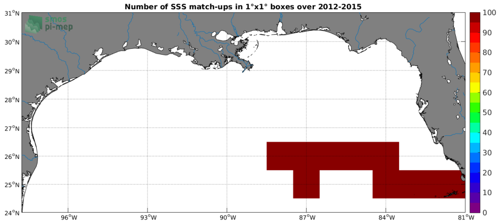
Figure 4: Number of SSS match-ups between TSG (GOSUD-Sailing-ship) SSS and the SMOS SSS L3 v2 - Monthly - 0.25 Deg (CATDS-CECOS-IFREMER) SSS product for the Mississippi river plume Pi-MEP region over 1^\circ \times 1^\circ boxes and for the full satellite product period.
