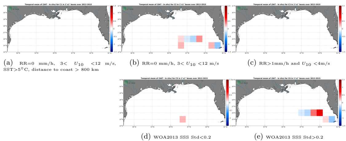
Figure 12: Temporal mean gridded over spatial boxes of size 1^\circ \times 1^\circ of \Delta SSS (SMOS-L3-CATDS-IFREMER-CECOS-V2-MONTHLY-0.25DEG - TSG-GOSUD-Sailing-ship) for 5 different sub-datasets corresponding to:RR=0 mm/h, 3 < U_{10} < 12 m/s, SST >5^\circ C, distance to coast > 800 km (a), RR=0 mm/h, 3 < U_{10} < 12 m/s (b), RR >1 mm/h and U_{10} < 4 m/s (c), WOA2013 SSS Std <0.2 (d), WOA2013 SSS Std >0.2 (e).
