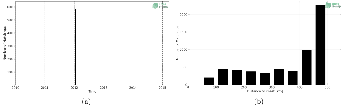
Figure 1: Number of match-ups between TSG-GOSUD-Sailing-ship and SMOS-L3-CATDS-IFREMER-CECOS-V2-MONTHLY-0.25DEG SSS as a function of time (a) and as function of the distance to coast (b) over the Mississippi river plume Pi-MEP region and for the full satellite product period.
