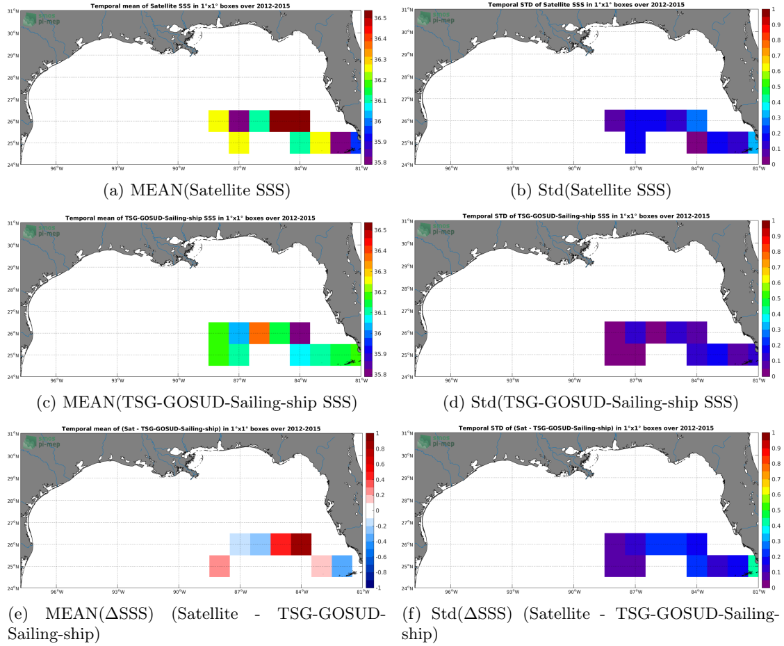
Figure 6: Temporal mean (left) and Std (right) of SSS from SMOS-L3-CATDS-IFREMER-CECOS-V2-MONTHLY-0.25DEG (top), TSG-GOSUD-Sailing-ship (middle), and of \Delta SSS (Satellite - TSG-GOSUD-Sailing-ship). Only match-up pairs are used to generate these maps.
