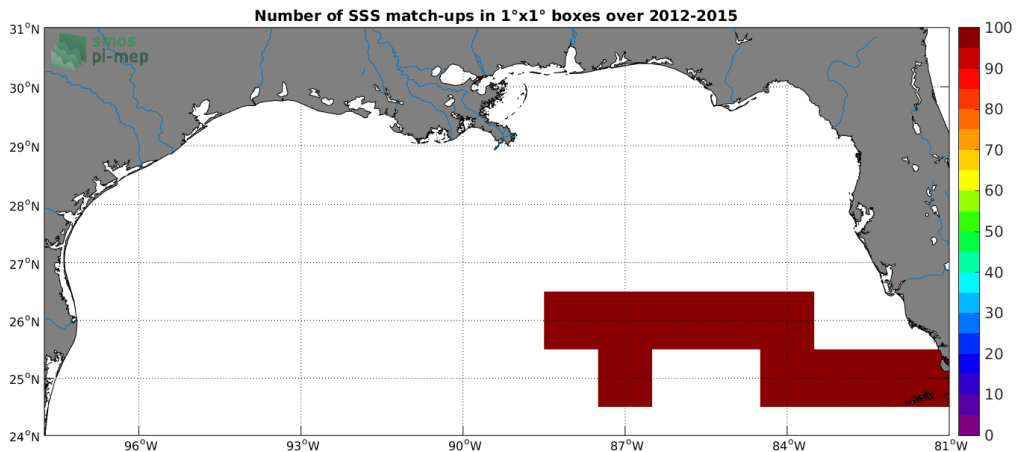
Figure 4: Number of SSS match-ups between TSG-GOSUD-Sailing-ship SSS and the SMOS-L3-CATDS-IFREMER-CECOS-V2-MONTHLY-0.25DEG SSS product for the Mississippi river plume Pi-MEP region over 1^\circ \times 1^\circ boxes and for the full satellite product period.
