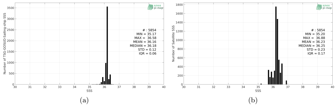
Figure 2: Histograms of SSS from TSG-GOSUD-Sailing-ship (a) and SMOS-L3-CATDS-IFREMER-CECOS-V2-MONTHLY-0.25DEG (b) considering all match-up pairs per bins of 0.1 over the Mississippi river plume Pi-MEP region and for the full satellite product period.
