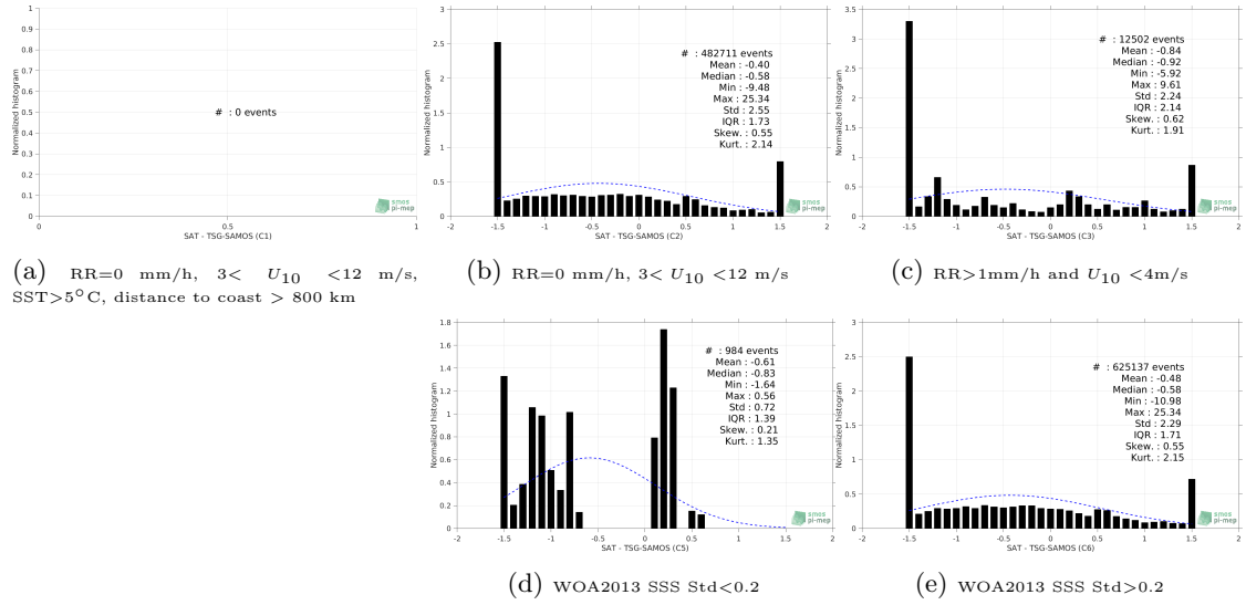
Figure 13: Normalized histogram of \Delta SSS (SMOS-L3-CATDS-CECOS-IFREMER-V2-1DAY-0.5DEG - TSG-SAMOS) for 5 different subdatasets corresponding to: RR=0 mm/h, 3 < U_{10} < 12 m/s, SST > 5°C, distance to coast > 800 km (a), RR=0 mm/h, 3 < U_{10} < 12 m/s (b), RR > 1mm/h and U_{10} < 4 m/s (c), WOA2013 SSS Std < 0.2 (d), WOA2013 SSS Std > 0.2 (e).
