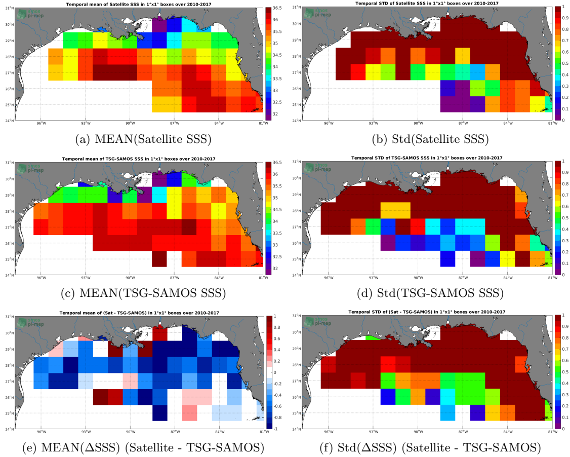
Figure 6: Temporal mean (left) and Std (right) of SSS from SMOS-L3-CATDS-CECOS-IFREMER-V2-1DAY-0.5DEG (top), TSG-SAMOS (middle), and of \Delta SSS (Satellite - TSG-SAMOS). Only match-up pairs are used to generate these maps.
