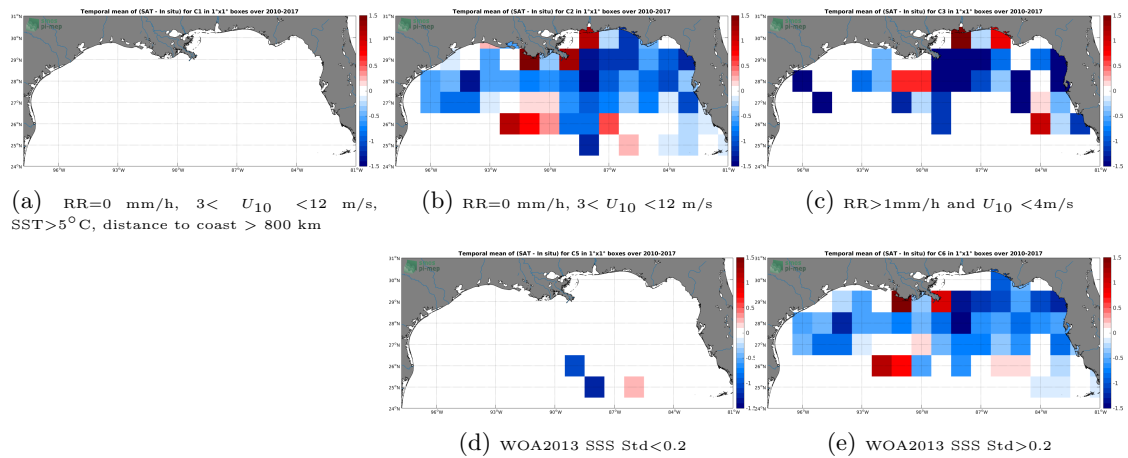
Figure 12: Temporal mean gridded over spatial boxes of size 1^\circ \times 1^\circ of \Delta SSS (SMOS-L3-CATDS-CECOS-IFREMER-V2-1DAY-0.5DEG - TSG-SAMOS) for 5 different subdatasets corresponding to: RR=0 mm/h, 3 < U_{10} < 12 m/s, SST > 5^\circ\text{C} , distance to coast > 800 km (a), RR=0 mm/h, 3 < U_{10} < 12 m/s (b), RR > 1 mm/h and U_{10} < 4 m/s (c), WOA2013 SSS Std < 0.2 (d), WOA2013 SSS Std > 0.2 (e).
