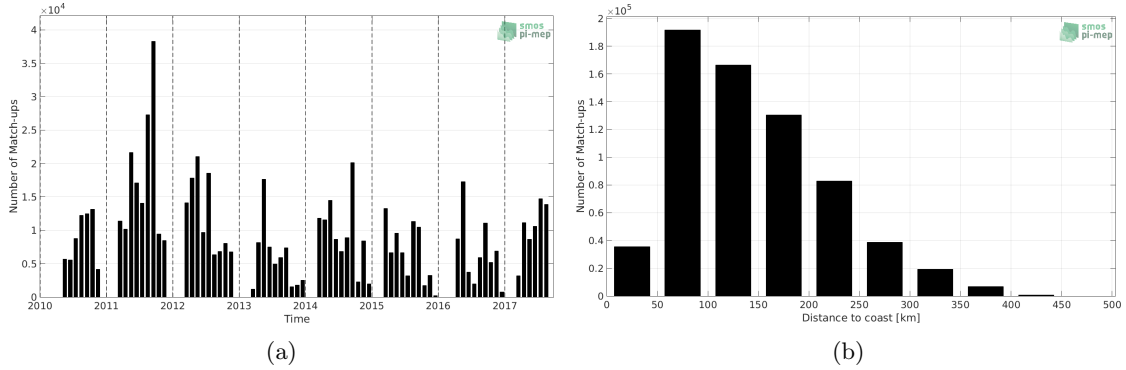
Figure 1: Number of match-ups between TSG-SAMOS and SMOS-L3-CATDS-CECOS-IFREMER-V2-1DAY-0.5DEG SSS as a function of time (a) and as function of the distance to coast (b) over the Mississippi river plume Pi-MEP region and for the full satellite product period.
