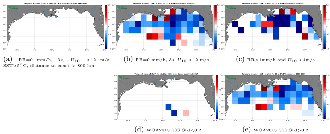
Figure 12: Temporal mean gridded over spatial boxes of size 1^\circ \times 1^\circ of \Delta SSS (SMOS-L3-CATDS-CECOS-IFREMER-V2-1DAY-0.5DEG - TSG-SAMOS) for 5 different subdatasets corresponding to:RR=0 mm/h, 3 < U_{10} < 12 m/s, SST >5^\circ C, distance to coast > 800 km (a), RR=0 mm/h, 3 < U_{10} < 12 m/s (b), RR >1 mm/h and U_{10} < 4 m/s (c), WOA2013 SSS Std <0.2 (d), WOA2013 SSS Std >0.2 (e).
