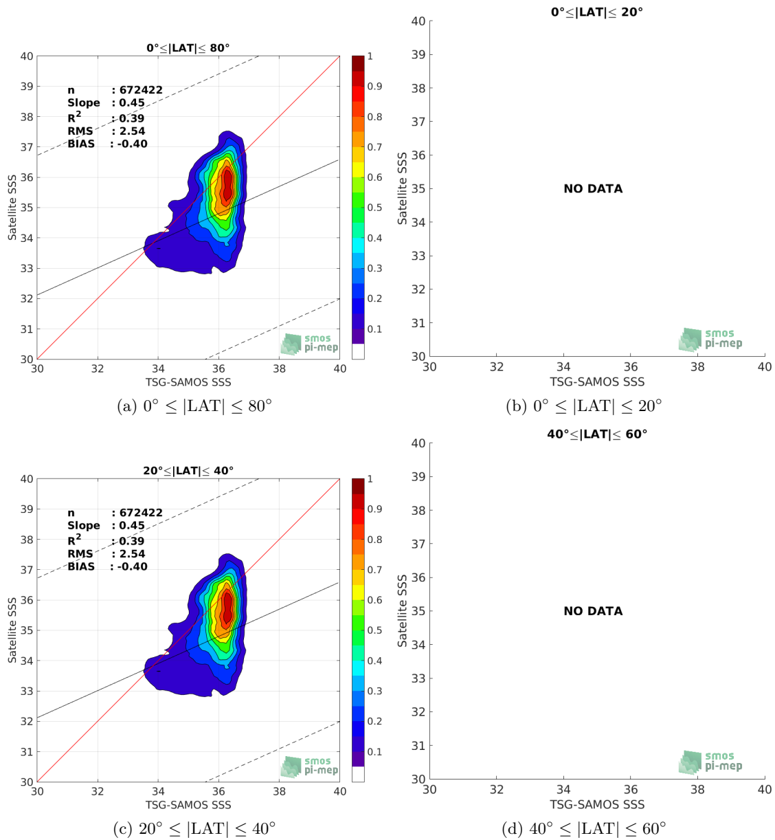
Figure 9: Contour maps of the concentration of SMOS-L3-CATDS-CECOS-IFREMER-V2-1DAY-0.5DEG SSS (y-axis) versus TSG-SAMOS SSS (x-axis) at match-up pairs for different latitude bands. For each plot, the red line shows x=y . The black thin and dashed lines indicate a linear fit through the data cloud and the \pm 95\% confidence levels, respectively. The number match-up pairs n , the slope and R^2 coefficient of the linear fit, the root mean square (RMS) and the mean bias between satellite and in situ data are indicated for each latitude band in each plots.
