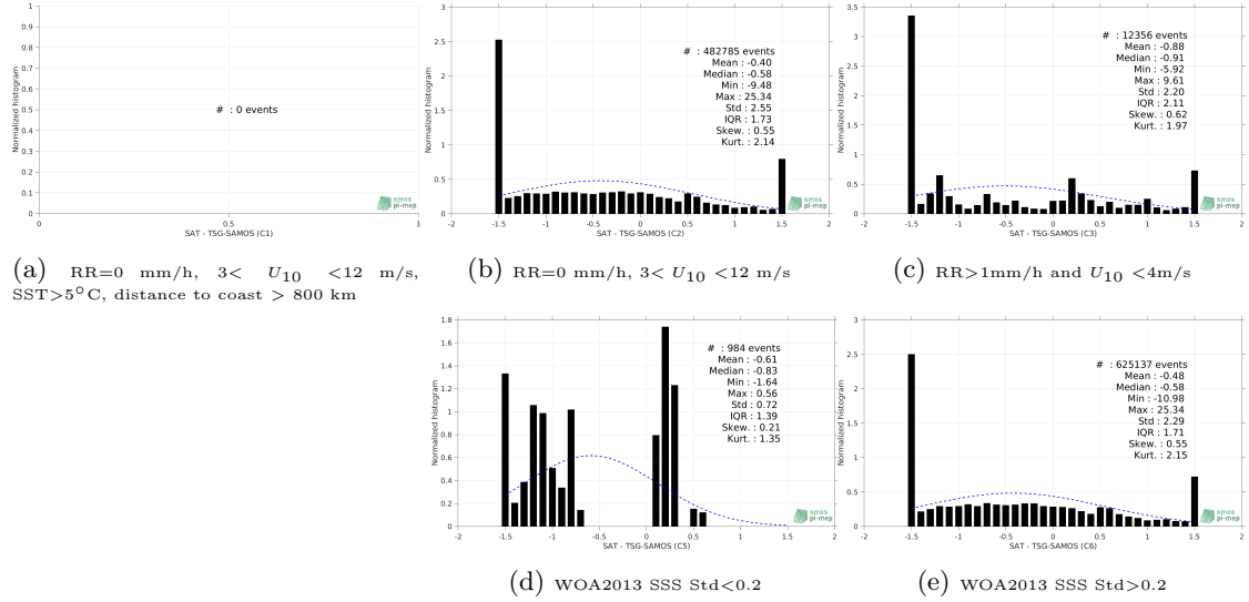
Figure 13: Normalized histogram of \Delta SSS (SMOS-L3-CATDS-CECOS-IFREMER-V2-1DAY-0.5DEG - TSG-SAMOS) for 5 different subdatasets corresponding to: RR=0 mm/h, 3 < U_{10} < 12 m/s, SST > 5°C, distance to coast > 800 km (a), RR=0 mm/h, 3 < U_{10} < 12 m/s (b), RR > 1mm/h and U_{10} < 4 m/s (c), WOA2013 SSS Std < 0.2 (d), WOA2013 SSS Std > 0.2 (e).
