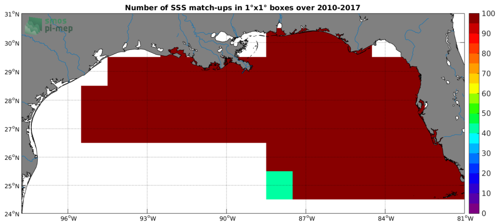
Figure 4: Number of SSS match-ups between TSG-SAMOS SSS and the SMOS-L3-CATDS-CECOS-IFREMER-V2-1DAY-0.5DEG SSS product for the Mississippi river plume Pi-MEP region over 1^\circ \times 1^\circ boxes and for the full satellite product period.
