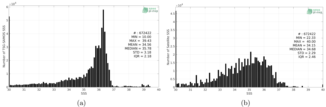
Figure 2: Histograms of SSS from TSG-SAMOS (a) and SMOS-L3-CATDS-CECOS-IFREMER-V2-1DAY-0.5DEG (b) considering all match-up pairs per bins of 0.1 over the Mississippi river plume Pi-MEP region and for the full satellite product period.
