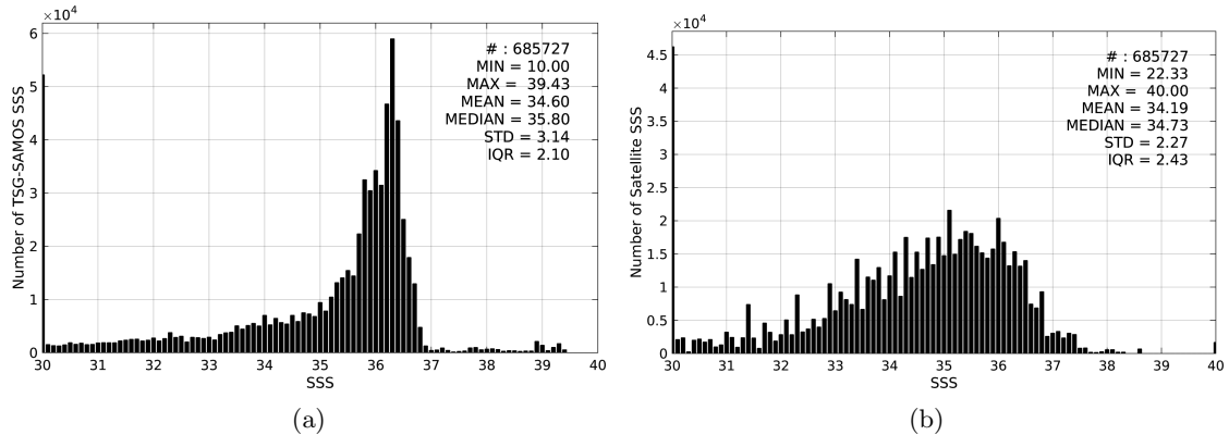
Figure 2: Histograms of SSS from TSG-SAMOS (a) and SMOS-L3-CATDS-CECOS-IFREMER-V2-1DAY-0.5deg (b) considering all match-up pairs per bins of 0.1 over the Mississippi river plume Pi-MEP region and for the full satellite product period.
