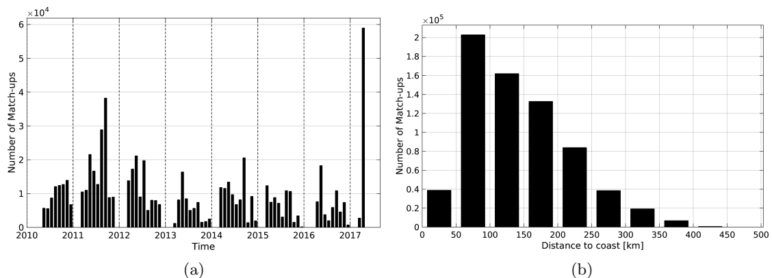
Figure 1: Number of match-ups between TSG-SAMOS and SMOS-L3-CATDS-CECOS-IFREMER-V2-1DAY-0.5deg SSS as a function of time (a) and as function of the distance to coast (b) over the Mississippi river plume Pi-MEP region and for the full satellite product period.
