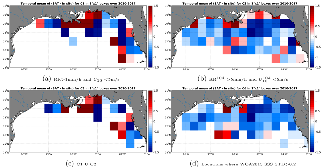
Figure 12: Temporal mean gridded over spatial boxes of size 1^\circ \times 1^\circ of \Delta SSS (SMOS-L3-CATDS-CECOS-IFREMER-V2-1DAY-0.5deg - TSG-SAMOS) for 4 different subdatasets corresponding to:RR > 1 mm/h and U_{10} < 5 m/s (a), RR^{10d} > 5 mm/h and U_{10}^{10d} < 5 m/s (b), C1 U C2 (c),Locations where WOA2013 SSS STD > 0.2 (d).
