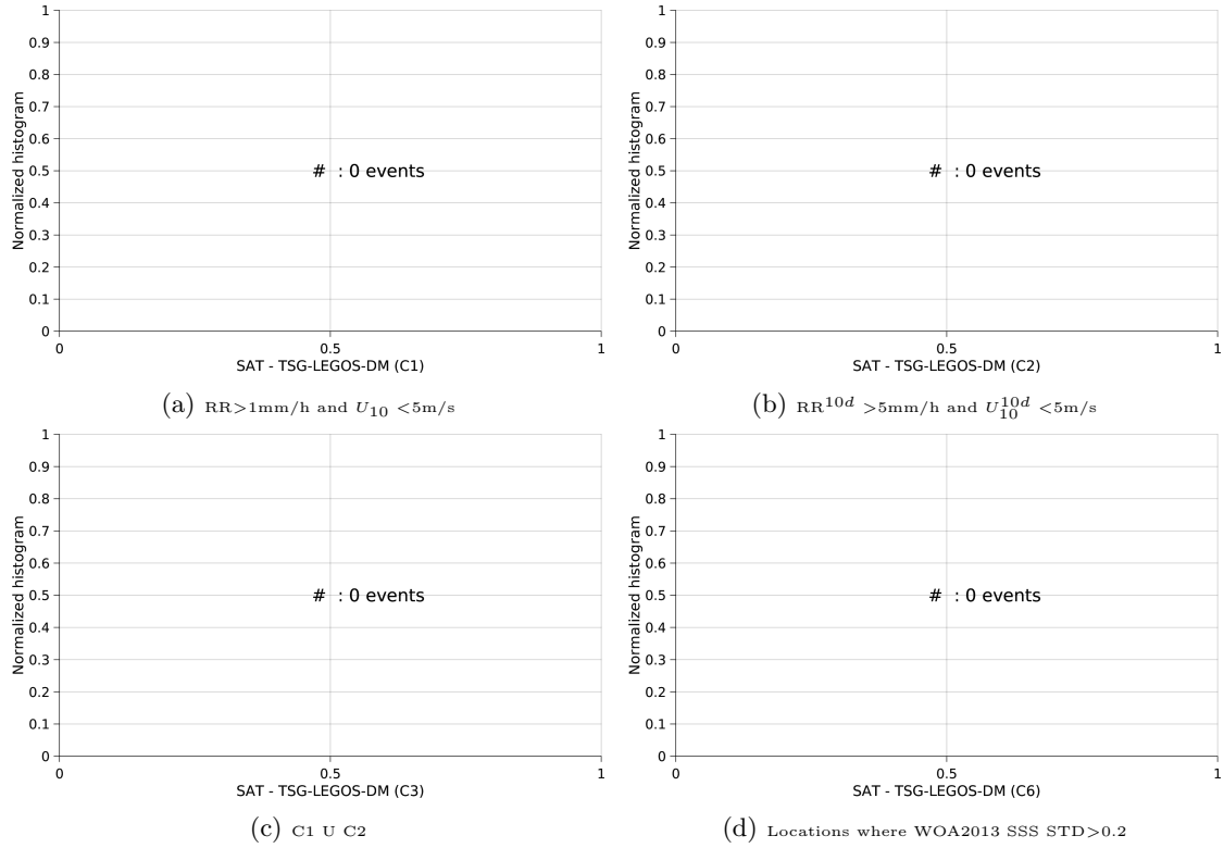
Figure 13: Normalized histogram of \Delta\text{SSS} (SMOS-L3-CATDS-CECOS-IFREMER-V2-1DAY-0.5deg - TSG-LEGOS-DM) for 6 different subdatasets corresponding to: RR > 1\text{mm/h} and U_{10} < 5\text{m/s} (a), RR^{10d} > 5\text{mm/h} and U_{10}^{10d} < 5\text{m/s} (b), C1 U C2 (c), Locations where WOA2013 SSS STD > 0.2 (d).
