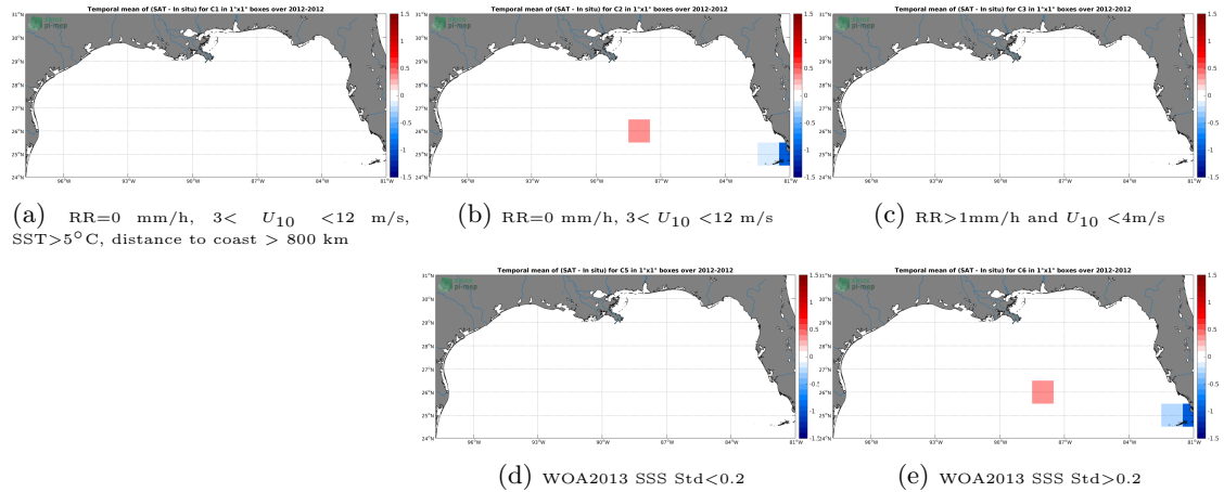
Figure 12: Temporal mean gridded over spatial boxes of size 1^\circ \times 1^\circ of \Delta SSS (SMOS SSS L3 v2 - Daily - 0.5 Deg (CATDS-CECOS-IFREMER) - TSG (GOSUD-Sailing-ship)) for 5 different subdatasets corresponding to:RR=0 mm/h, 3 < U_{10} < 12 m/s, SST > 5^\circ\text{C} , distance to coast > 800 km (a), RR=0 mm/h, 3 < U_{10} < 12 m/s (b), RR > 1 mm/h and U_{10} < 4 m/s (c), WOA2013 SSS Std < 0.2 (d), WOA2013 SSS Std > 0.2 (e).
