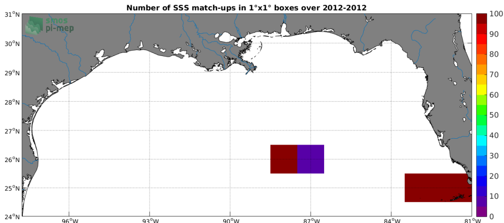
Figure 4: Number of SSS match-ups between TSG (GOSUD-Sailing-ship) SSS and the SMOS SSS L3 v2 - Daily - 0.5 Deg (CATDS-CECOS-IFREMER) SSS product for the Mississippi river plume Pi-MEP region over 1°x1° boxes and for the full satellite product period.
