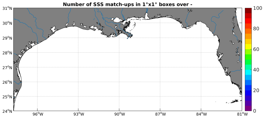
Figure 4: Number of SSS match-ups between TSG-GOSUD-Sailing-ship SSS and the SMOS-L3-CATDS-CECOS-IFREMER-V2-1DAY-0.5deg SSS product for the Mississippi river plume Pi-MEP region over 1^\circ \times 1^\circ boxes and for the full satellite product period.
