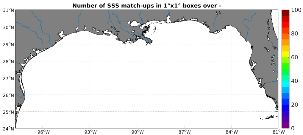
Figure 4: Number of SSS match-ups between TSG-GOSUD-Research-vessel SSS and the SMOS-L3-CATDS-CECOS-IFREMER-V2-1DAY-0.5deg SSS product for the Mississippi river plume Pi-MEP region over 1^{\circ} \times 1^{\circ} boxes and for the full satellite product period.
