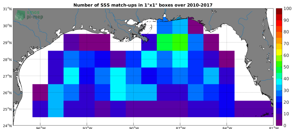
Figure 4: Number of SSS match-ups between Argo SSS and the SMOS SSS L3 v2 - Daily - 0.5 Deg (CATDS-CECOS-IFREMER) SSS product for the Mississippi river plume Pi-MEP region over 1°x1° boxes and for the full satellite product period.
