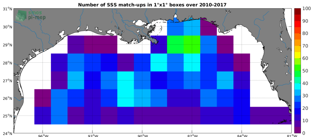
Figure 4: Number of SSS match-ups between Argo SSS and the SMOS L3 v2 - Daily - 0.5 Deg (CATDS-CECOS-IFREMER) SSS product for the Mississippi river plume Pi-MEP region over 1^\circ \times 1^\circ boxes and for the full satellite product period.
