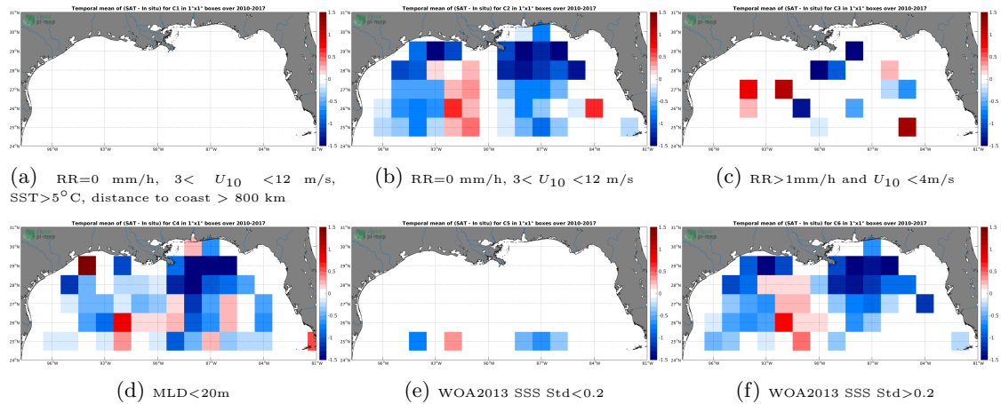
Figure 12: Temporal mean gridded over spatial boxes of size 1^{\circ}\times 1^{\circ} of \Delta\text{SSS} (SMOS L3 v2 - Daily - 0.5 Deg (CATDS-CECOS-IFREMER) - Argo) for 6 different subdatasets corresponding to: RR=0 mm/h, 3 < U_{10} < 12 m/s, SST > 5^{\circ}\text{C} , distance to coast > 800 km (a), RR=0 mm/h, 3 < U_{10} < 12 m/s (b), RR > 1 mm/h and U_{10} < 4 m/s (c), MLD < 20\text{m} (d), WOA2013 SSS Std < 0.2 (e), WOA2013 SSS Std > 0.2 (f).
