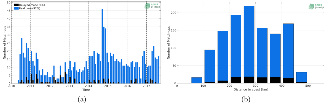
Figure 1: Number of match-ups between Argo and SMOS L3 v2 - Daily - 0.5 Deg (CATDS-CECOS-IFREMER) SSS as a function of time (a) and as function of the distance to coast (b) over the Mississippi river plume Pi-MEP region and for the full satellite product period.
