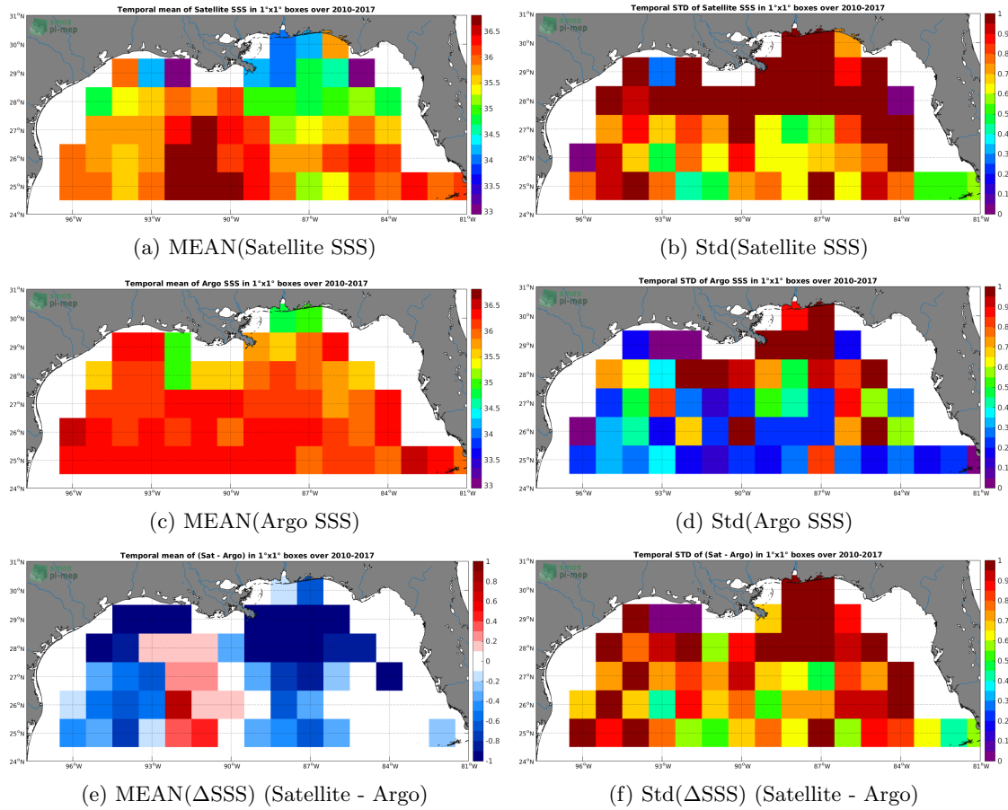
Figure 6: Temporal mean (left) and Std (right) of SSS from SMOS L3 v2 - Daily - 0.5 Deg (CATDS-CECOS-IFREMER) (top), Argo (middle), and of \Delta SSS (Satellite - Argo). Only match-up pairs are used to generate these maps.
