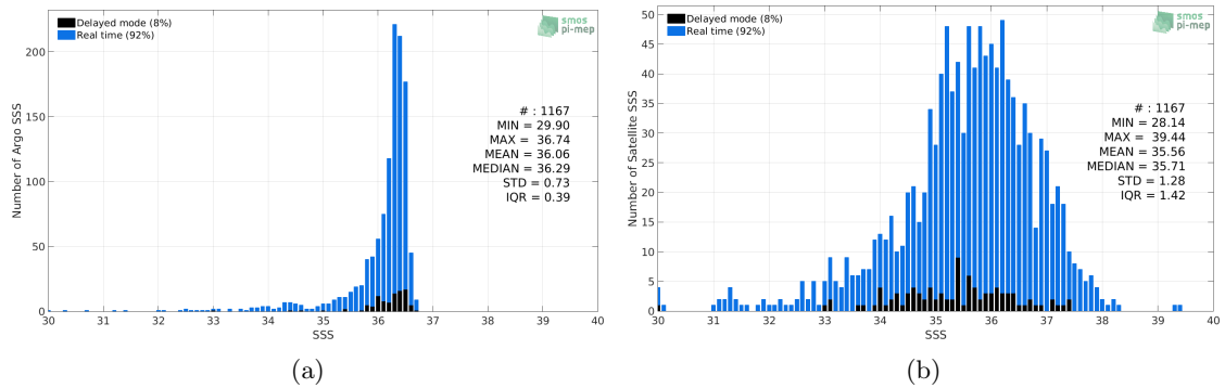
Figure 2: Histograms of SSS from Argo (a) and SMOS L3 v2 - Daily - 0.5 Deg (CATDS-CECOS-IFREMER) (b) considering all match-up pairs per bins of 0.1 over the Mississippi river plume Pi-MEP region and for the full satellite product period.
