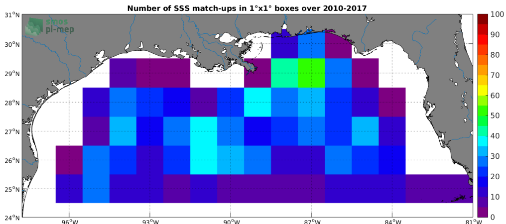
Figure 4: Number of SSS match-ups between Argo SSS and the SMOS-L3-CATDS-CECOS-IFREMER-V2-1DAY-0.5DEG SSS product for the Mississippi river plume Pi-MEP region over 1^\circ \times 1^\circ boxes and for the full satellite product period.
