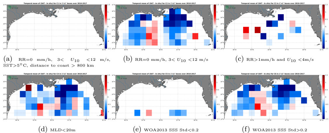
Figure 12: Temporal mean gridded over spatial boxes of size 1^\circ \times 1^\circ of \Delta SSS (SMOS-L3-CATDS-CECOS-IFREMER-V2-1DAY-0.5DEG - Argo) for 6 different subdatasets corresponding to: RR=0 mm/h, 3 < U_{10} < 12 m/s, SST > 5^\circ\text{C} , distance to coast > 800 km (a), RR=0 mm/h, 3 < U_{10} < 12 m/s (b), RR > 1 mm/h and U_{10} < 4 m/s (c), MLD < 20 m (d), WOA2013 SSS Std < 0.2 (e), WOA2013 SSS Std > 0.2 (f).
