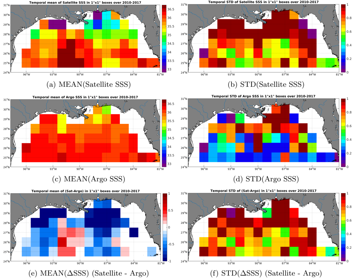
Figure 6: Temporal mean (left) and STD (right) of SSS from SMOS-L3-CATDS-CECOS-IFREMER-V2-1DAY-0.5deg (top), Argo (middle), and of \Delta\text{SSS} (Satellite - Argo). Only match-up pairs are used to generate these maps.
