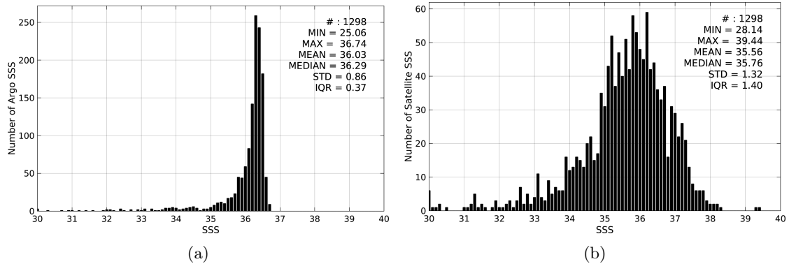
Figure 2: Histograms of SSS from Argo (a) and SMOS-L3-CATDS-CECOS-IFREMER-V2-1DAY-0.5deg (b) considering all match-up pairs per bins of 0.1 over the Mississippi river plume Pi-MEP region and for the full satellite product period.
