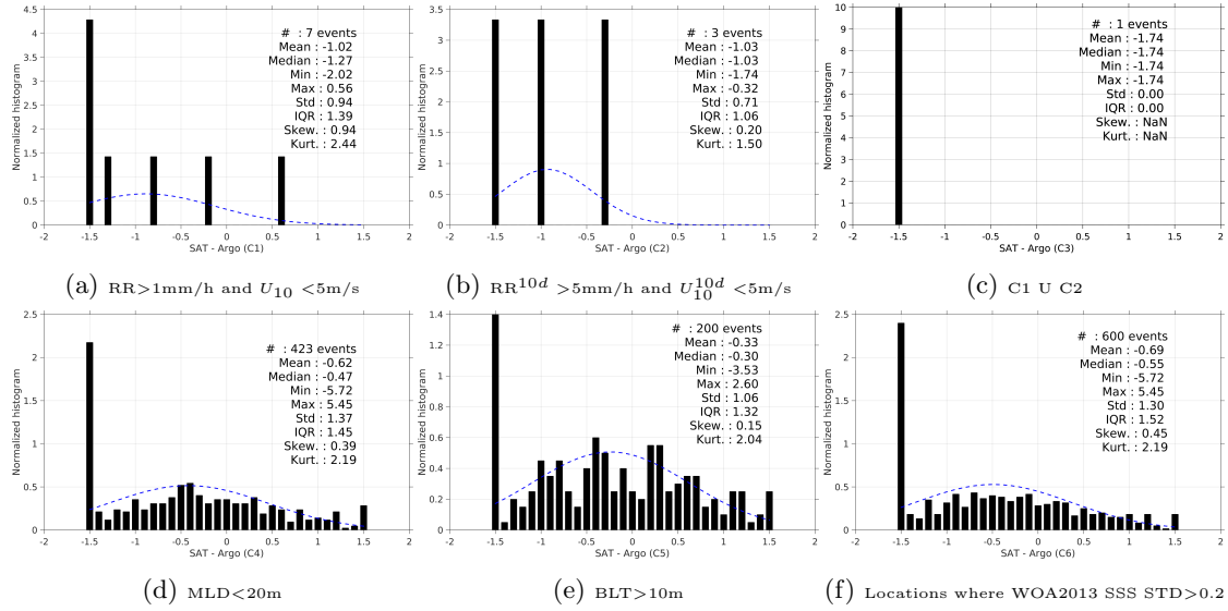
Figure 13: Normalized histogram of \Delta SSS (SMOS-L3-CATDS-CECOS-IFREMER-V2-1DAY-0.5deg - Argo) for 6 different subdatasets corresponding to: RR > 1\text{mm/h} and U_{10} < 5\text{m/s} (a), RR^{10d} > 5\text{mm/h} and U_{10}^{10d} < 5\text{m/s} (b), C1 U C2 (c), MLD < 20\text{m} (d), BLT > 10\text{m} (e), Locations where WOA2013 SSS STD > 0.2 (f).
