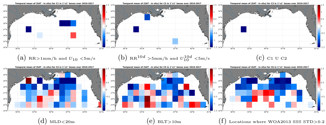
Figure 12: Temporal mean gridded over spatial boxes of size 1^\circ \times 1^\circ of \Delta SSS (SMOS-L3-CATDS-CECOS-IFREMER-V2-1DAY-0.5deg - Argo) for 6 different subdatasets corresponding to: RR > 1\text{mm/h} and U_{10} < 5\text{m/s} (a), RR^{10d} > 5\text{mm/h} and U_{10}^{10d} < 5\text{m/s} (b), C1 U C2 (c), MLD < 20\text{m} (d), BLT > 10\text{m} (e), Locations where WOA2013 SSS STD > 0.2 (f).
