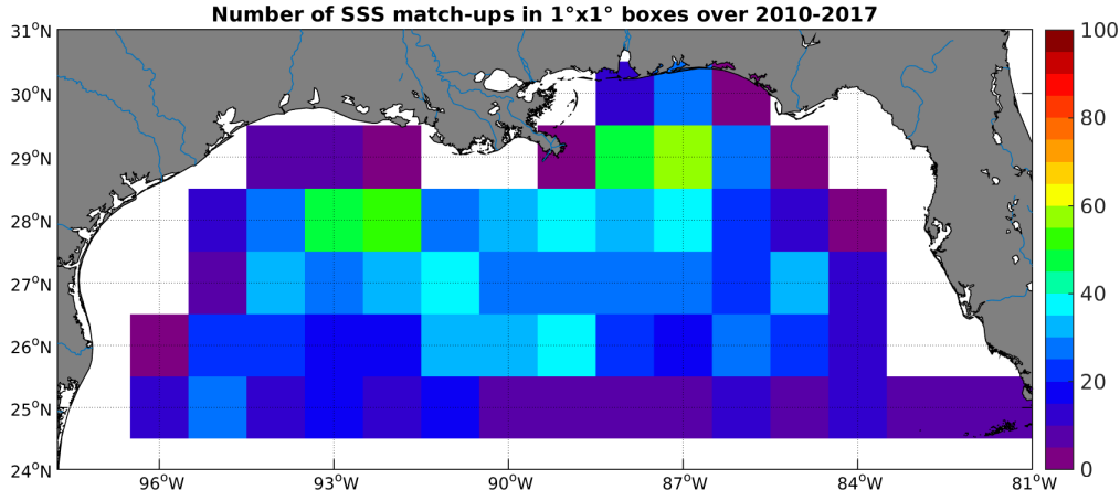
Figure 4: Number of SSS match-ups between Argo SSS and the SMOS-L3-CATDS-CECOS-IFREMER-V2-1DAY-0.5deg SSS product for the Mississippi river plume Pi-MEP region over 1^\circ \times 1^\circ boxes and for the full satellite product period.
