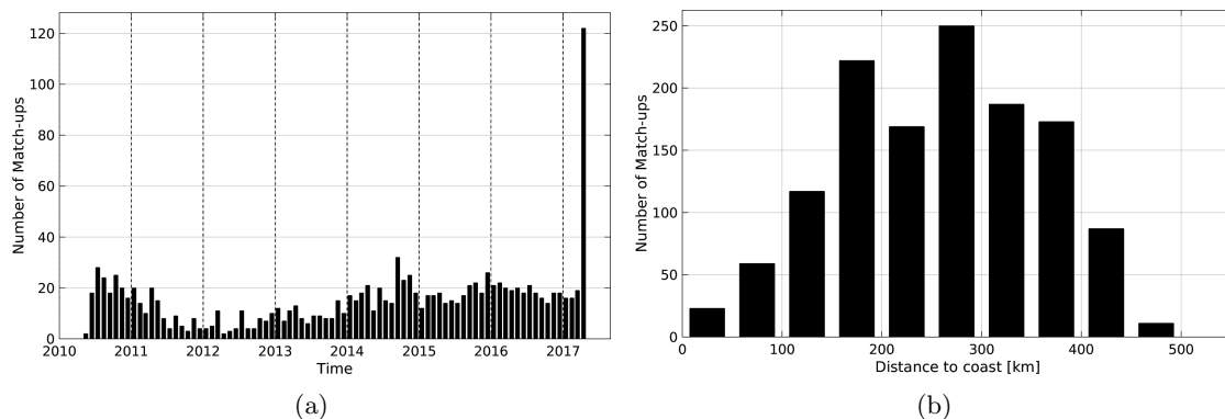
Figure 1: Number of match-ups between Argo and SMOS-L3-CATDS-CECOS-IFREMER-V2-1DAY-0.5deg SSS as a function of time (a) and as function of the distance to coast (b) over the Mississippi river plume Pi-MEP region and for the full satellite product period.
