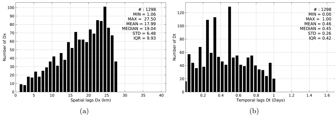
Figure 5: Histograms of the spatial (a) and temporal (b) lags between the time of the Argo measurements and the date of the corresponding SMOS-L3-CATDS-CECOS-IFREMER-V2-1DAY-0.5deg SSS product.
